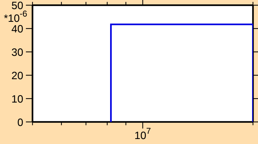
\sigma vs. E for ^{196}\text{Tl}(n,3n)
