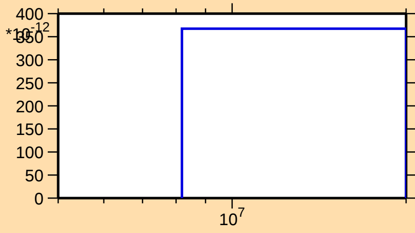
\sigma vs. E for ^{196}\text{Tl}(n,nt)
