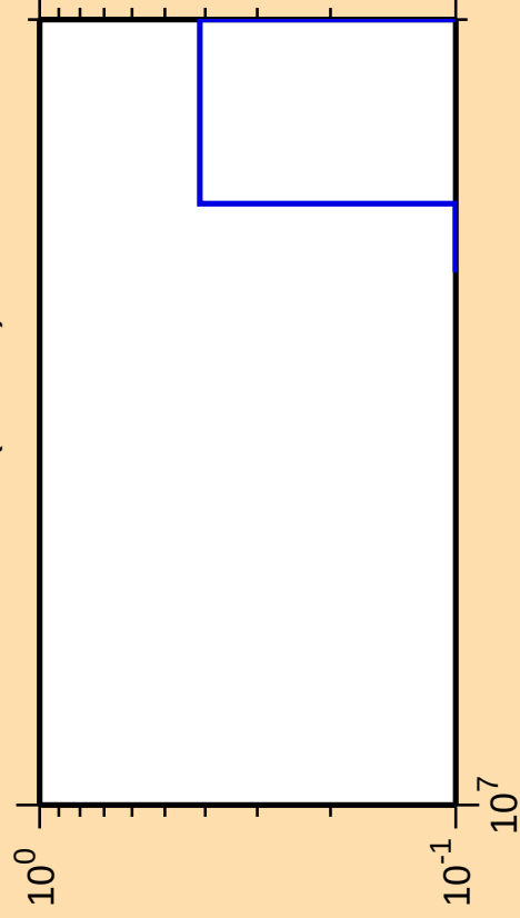
\Delta\sigma/\sigma vs. E for ^{213}\text{Tl}(\text{mt } 42)
