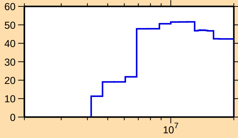
\Delta\sigma/\sigma vs. E for ^{213}\text{Tl}(n,n\text{cont.})
