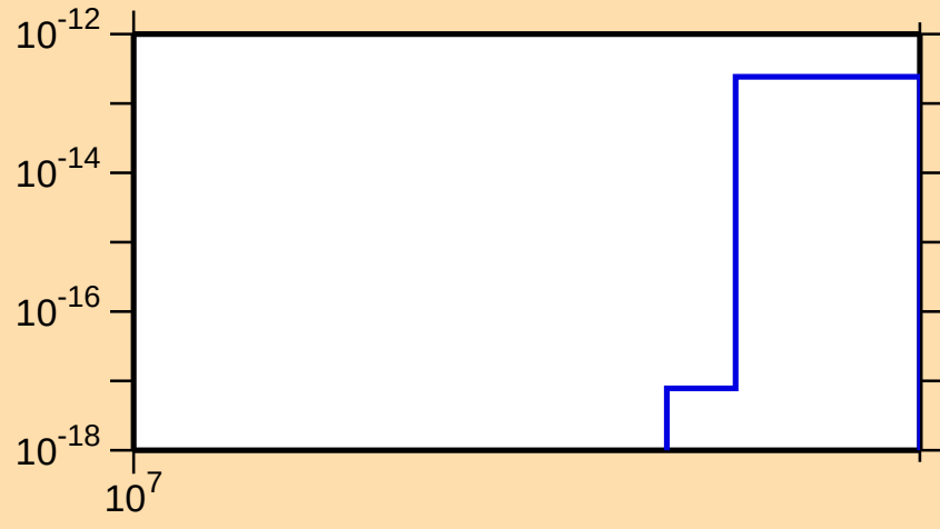
\sigma vs. E for ^{213}\text{Tl}(\text{mt } 42)
