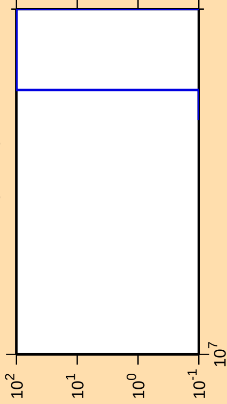
\Delta\sigma/\sigma vs. E for ^{213}\text{Tl}(\text{mt 11})
