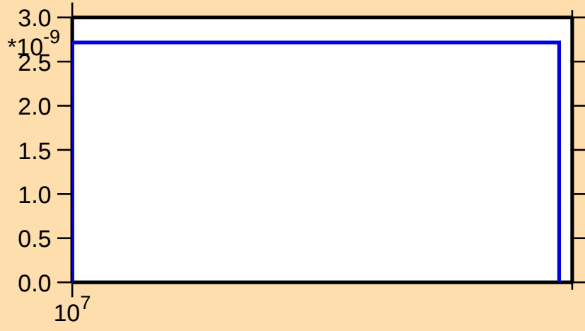
\sigma vs. E for ^{213}\text{Tl}(n,2n\alpha)
