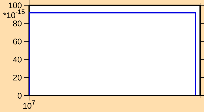
\sigma vs. E for ^{213}\text{Tl}(\text{mt } 11)
