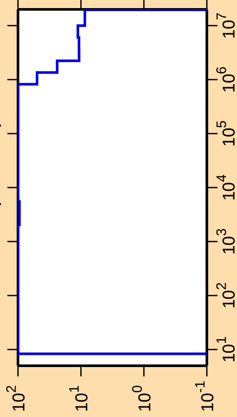
\Delta\sigma/\sigma vs. E for ^{213}\text{Tl}(n,\text{nonel.})
