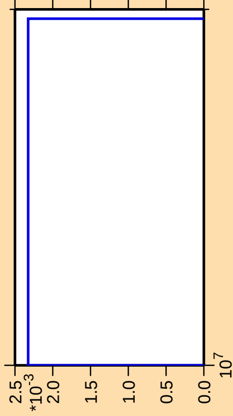
\Delta\sigma/\sigma vs. E for ^{213}\text{Tl}(\text{mt 42})
