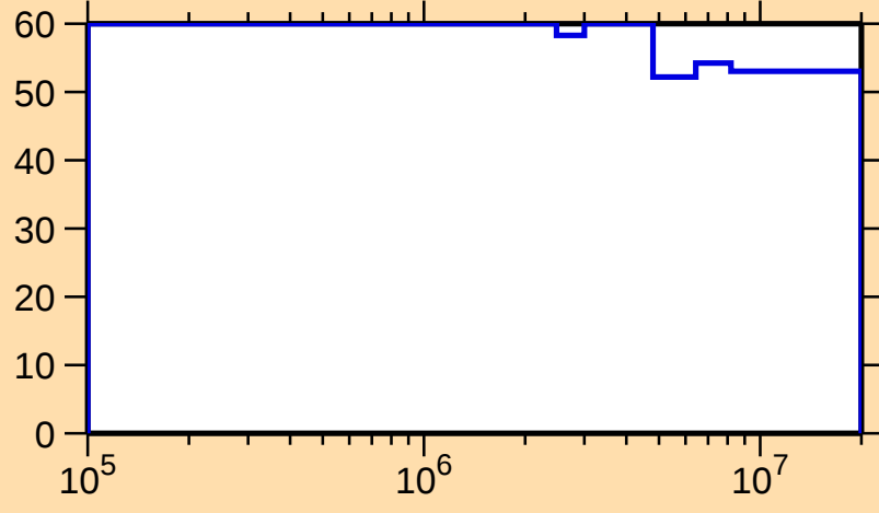
\Delta\sigma/\sigma vs. E for ^{213}\text{Tl}(n,n_1)
