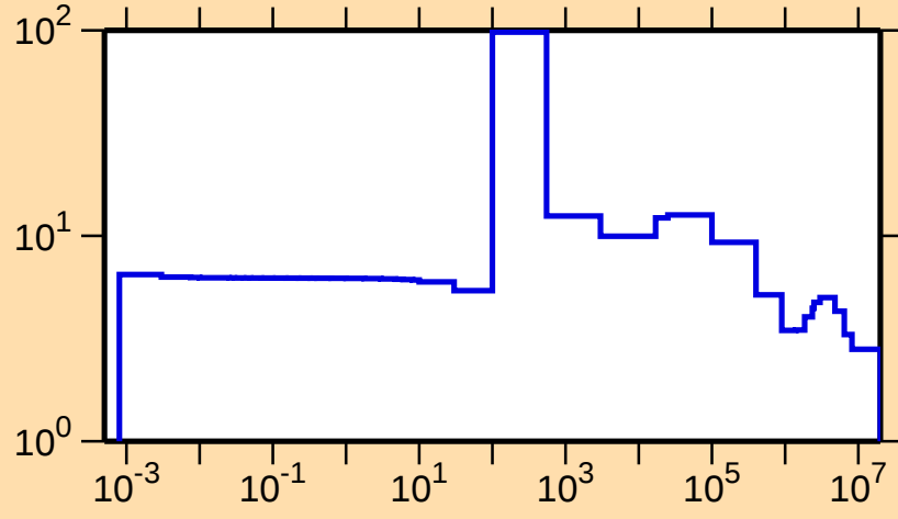
\sigma vs. E for ^{213}\text{Tl}(n,\text{el.})
