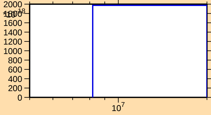
\sigma vs. E for ^{213}\text{Tl}(\text{mt } 42)
