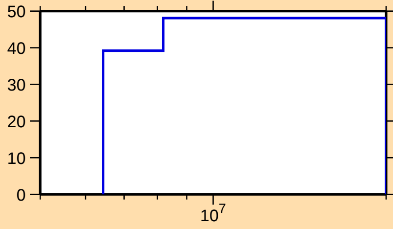
\Delta\sigma/\sigma vs. E for ^{213}\text{Tl}(n,n\text{cont.})
