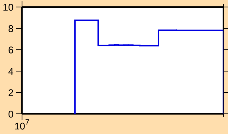
\Delta\sigma/\sigma vs. E for ^{151}\text{Tm}(n,\text{el.})
