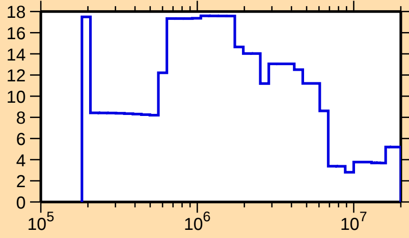
\Delta\sigma/\sigma vs. E for ^{151}\text{Tm}(n,\text{tot.})
