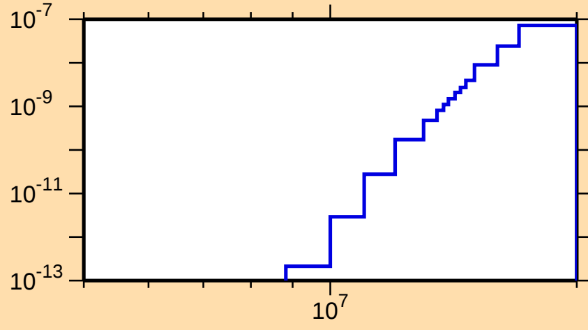
\sigma vs. E for ^{151}\text{Tm}(\text{mt117})
