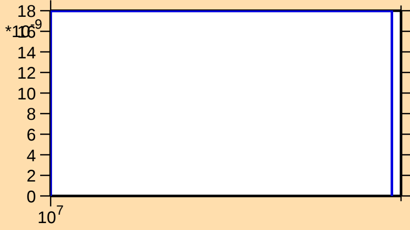
\sigma vs. E for ^{151}\text{Tm}(n,\text{nd})
