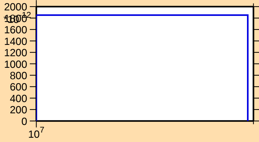
\sigma vs. E for ^{151}\text{Tm}(n,\text{pt})
