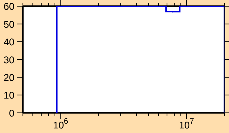
\Delta\sigma/\sigma vs. E for ^{152}\text{Tm}(n,n\text{cont.})
