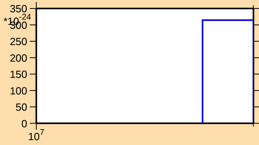
\sigma vs. E for ^{152}\text{Tm}(\text{mt } 11)
