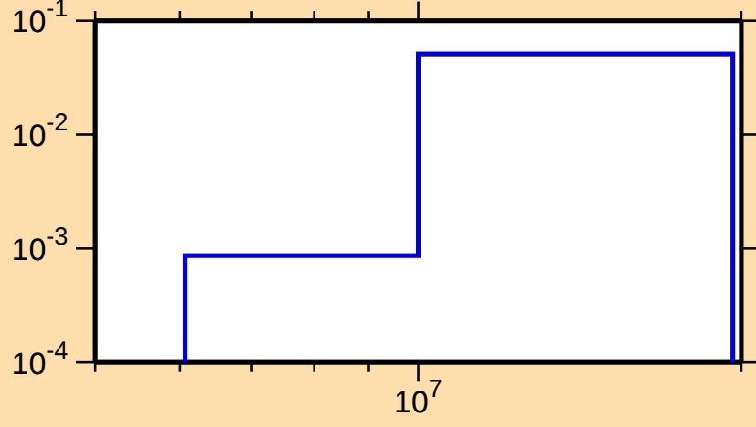
\sigma vs. E for ^{152}\text{Tm}(n,2n)
