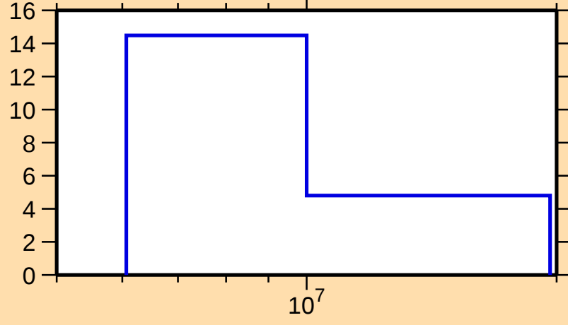
\Delta\sigma/\sigma vs. E for ^{152}\text{Tm}(n,\text{el.})
