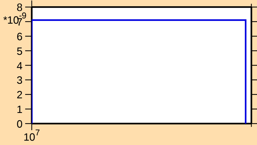
\sigma vs. E for ^{152}\text{Tm}(n,2n\alpha)
