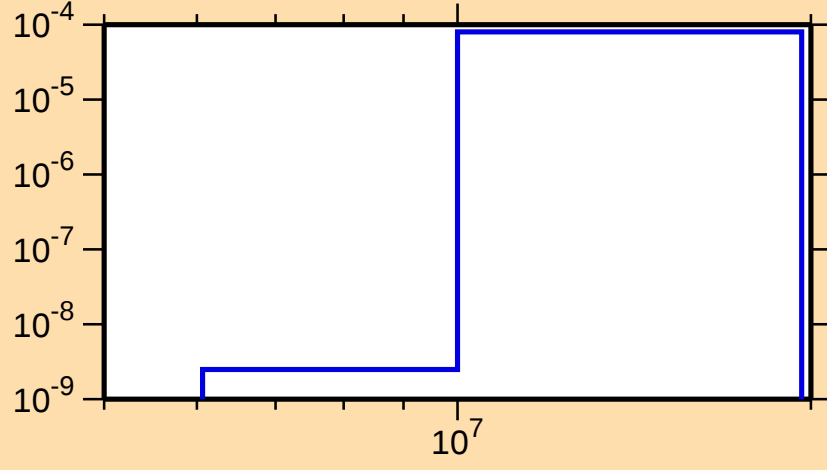
\sigma vs. E for ^{152}\text{Tm} (mt 45)
