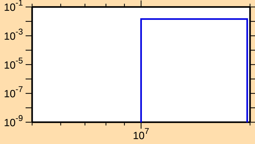
\sigma vs. E for ^{152}\text{Tm}(n,2np)
