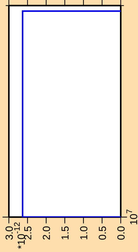
\Delta\sigma/\sigma vs. E for ^{152}\text{Tm} (mt 11)
