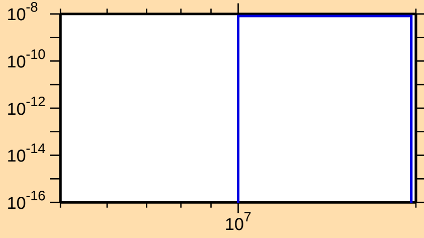
\sigma vs. E for ^{152}\text{Tm} (mt 34)
