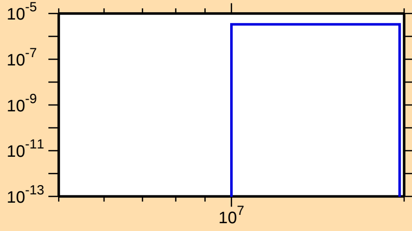
\sigma vs. E for ^{152}\text{Tm}(n,\text{pt})
