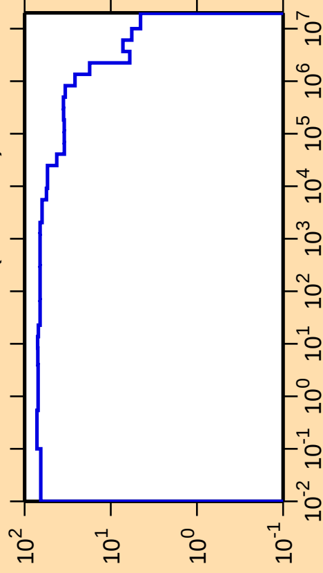
\Delta\sigma/\sigma vs. E for ^{152}\text{Tm}(n,\text{nonel.})
