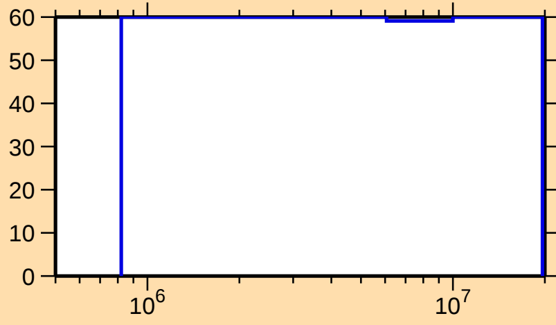
\Delta\sigma/\sigma vs. E for ^{152}\text{Tm}(n,n\text{cont.})
