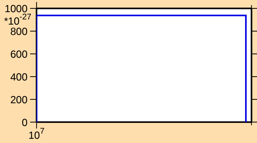
\sigma vs. E for ^{152}\text{Tm} (mt 11)
