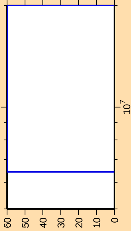
\Delta\sigma/\sigma vs. E for ^{152}\text{Tm}(\text{mt } 45)
