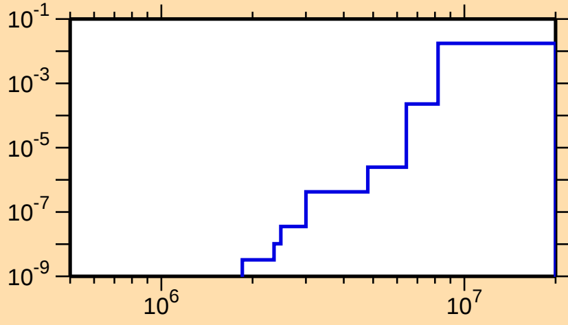
\sigma vs. E for ^{152}\text{Tm}(n,d)
