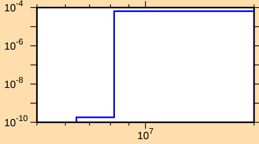
\sigma vs. E for ^{152}\text{Tm}(\text{mt } 45)
