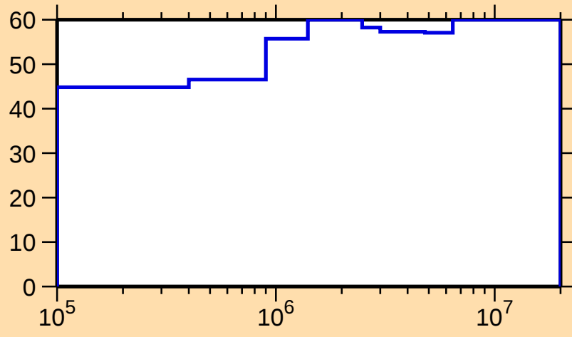
\Delta\sigma/\sigma vs. E for ^{152}\text{Tm}(n,n_1)
