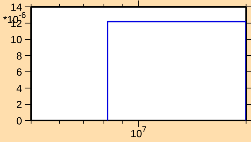
\sigma vs. E for ^{152}\text{Tm}(n,\text{nd})
