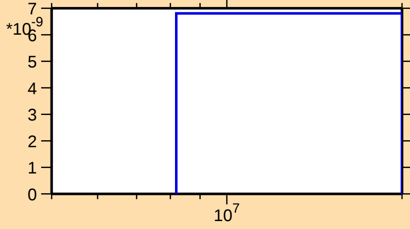
\sigma vs. E for ^{152}\text{Tm}(\text{mt } 34)
