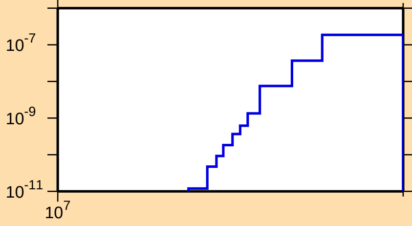
\sigma vs. E for ^{152}\text{Tm}(n,2n\alpha)
