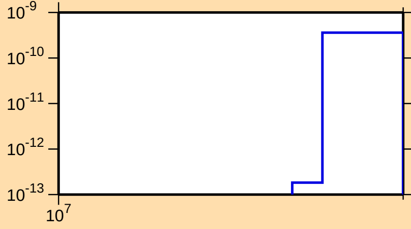
\sigma vs. E for ^{152}\text{Tm}(n,nt)
