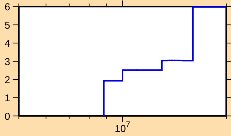
\Delta\sigma/\sigma vs. E for ^{152}\text{Tm}(n,\text{tot.})
