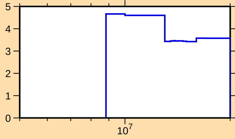
\Delta\sigma/\sigma vs. E for ^{152}\text{Tm}(n,\text{nonel.})
