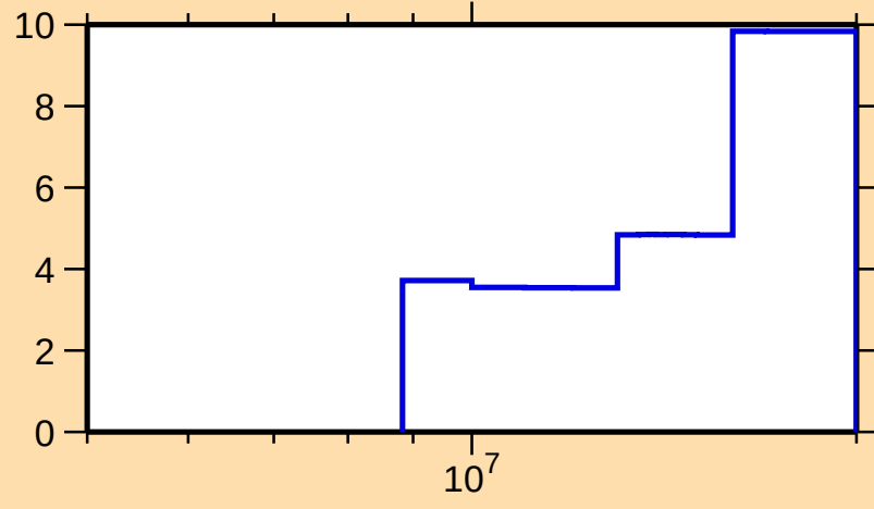
\Delta\sigma/\sigma vs. E for ^{152}\text{Tm}(n,\text{el.})
