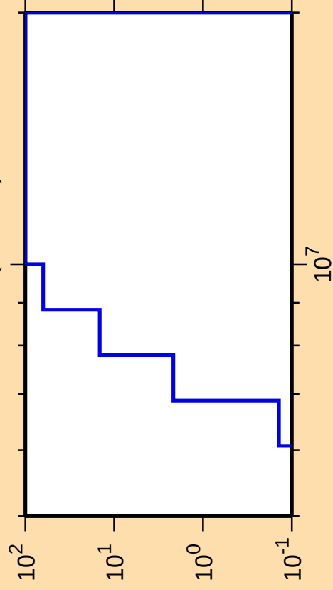
\Delta\sigma/\sigma vs. E for ^{152}\text{Tm}(\text{mt117})
