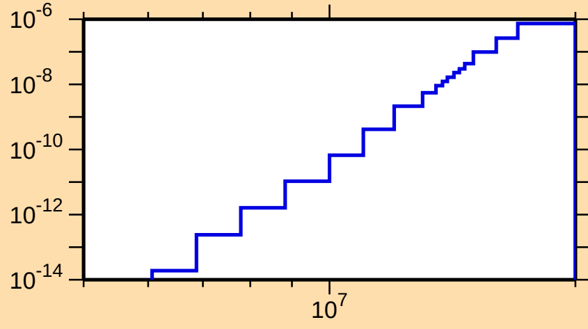
\sigma vs. E for ^{152}\text{Tm}(\text{mt117})
