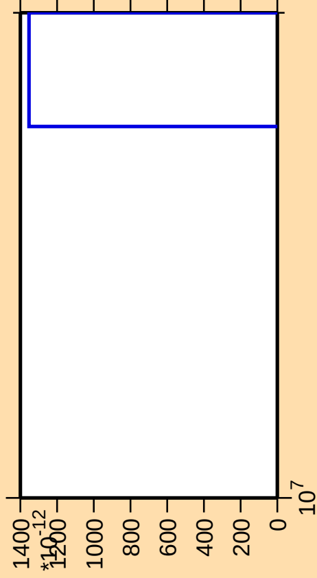
\Delta\sigma/\sigma vs. E for ^{152}\text{Tm}(\text{mt } 11)
