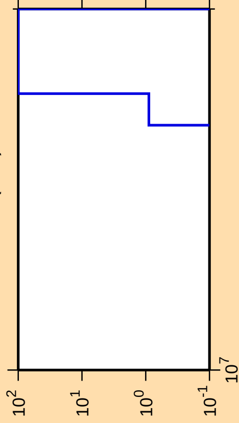
\Delta\sigma/\sigma vs. E for ^{152}\text{Tm}(n,nt)
