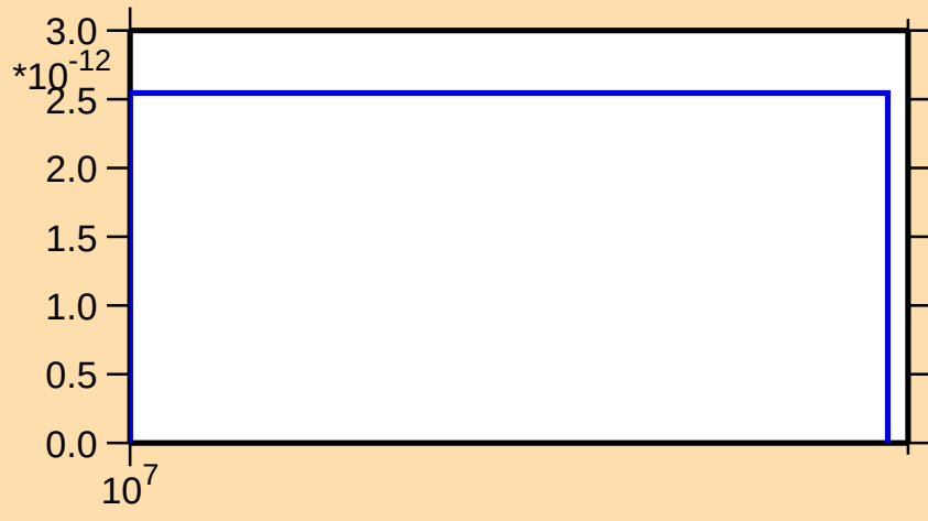
\sigma vs. E for ^{152}\text{Tm}(n,nt)
