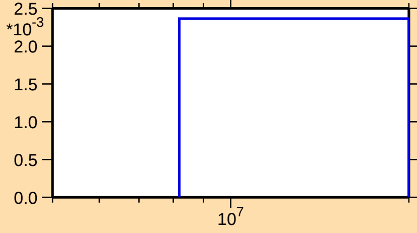
\sigma vs. E for ^{152}\text{Tm}(n,2np)
