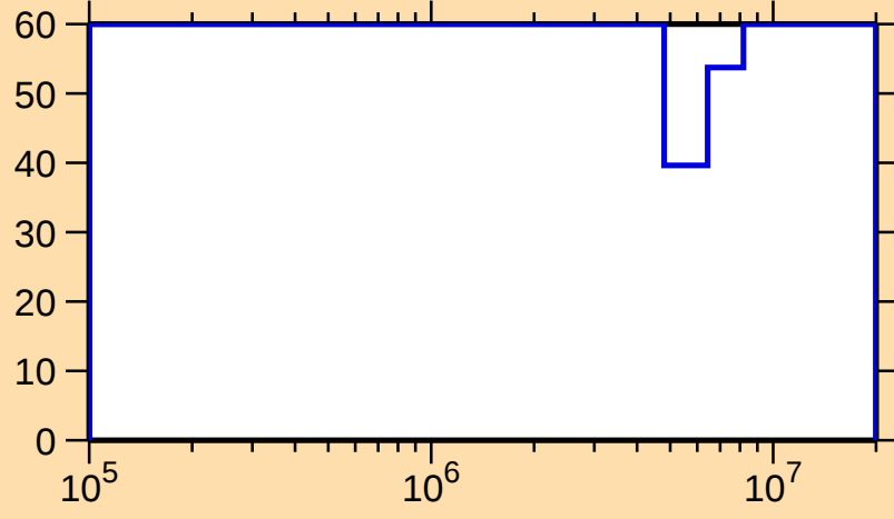
\Delta\sigma/\sigma vs. E for ^{152}\text{Tm}(n,n_1)
