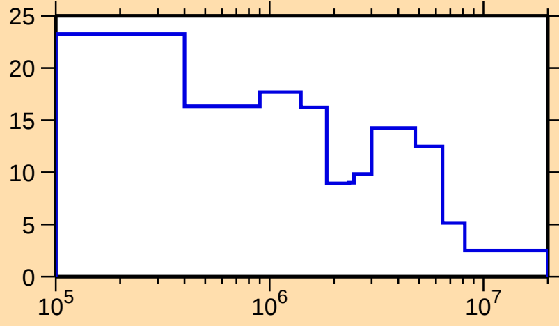
\Delta\sigma/\sigma vs. E for ^{152}\text{Tm}(n,\text{tot.})
