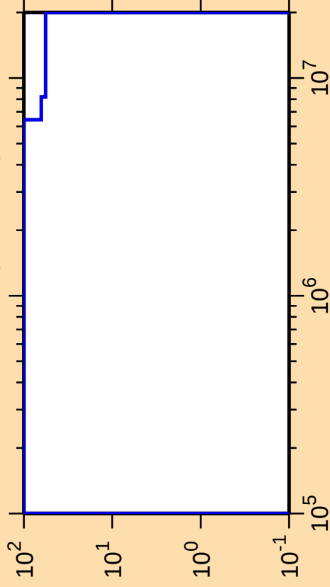
\Delta\sigma/\sigma vs. E for ^{152}\text{Tm}(n,n_{\text{cont}})
