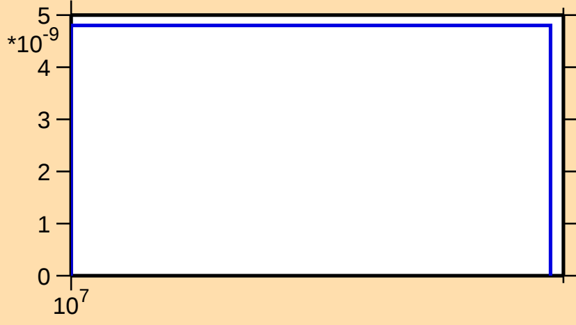
\sigma vs. E for ^{153}\text{Tm}(n,\text{pt})
