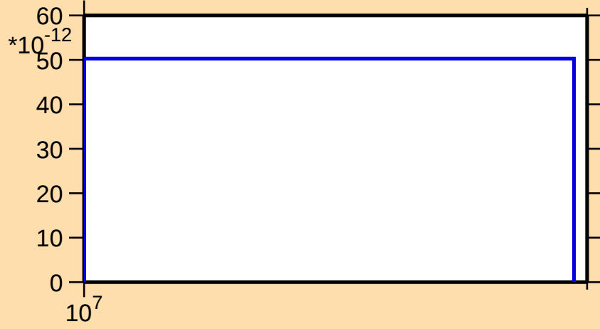
\sigma vs. E for ^{153}\text{Tm} (mt 34)
