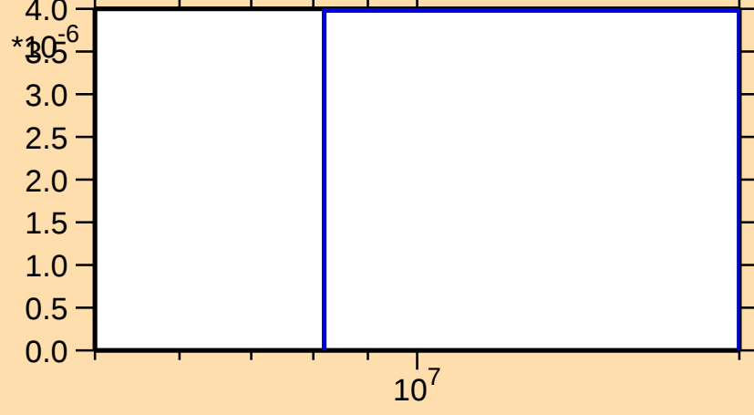
\sigma vs. E for ^{153}\text{Tm}(n,\text{pd})
