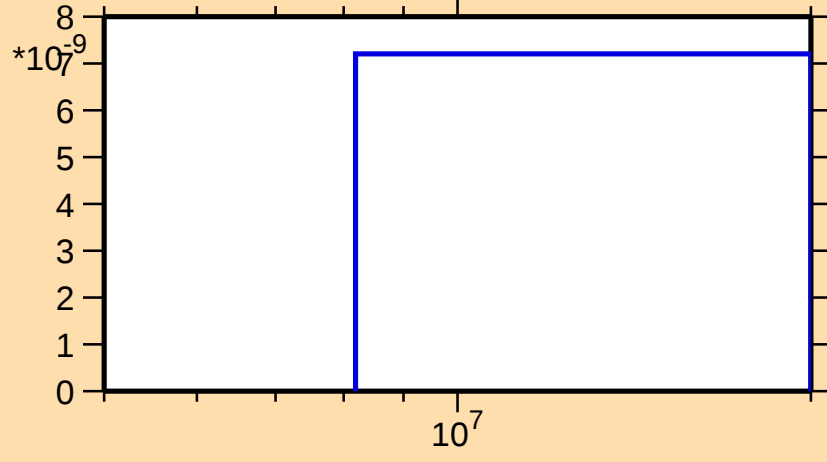
\sigma vs. E for ^{153}\text{Tm}(n,3n)
