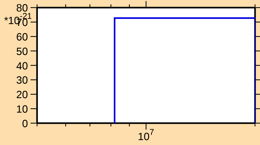
\sigma vs. E for ^{153}\text{Tm} (mt 42)
