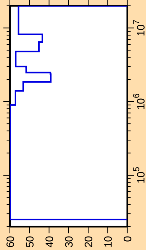
\Delta\sigma/\sigma vs. E for ^{153}\text{Tm}(n,\text{inel.})
