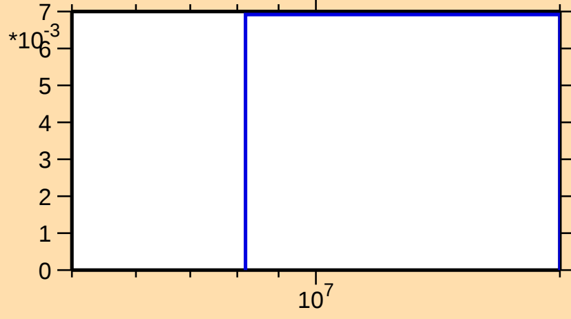
\sigma vs. E for ^{153}\text{Tm}(n,2n)
