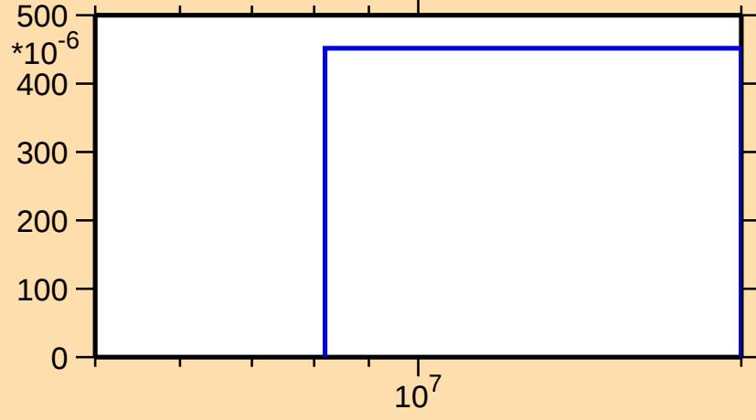
\sigma vs. E for ^{153}\text{Tm}(n,2np)
