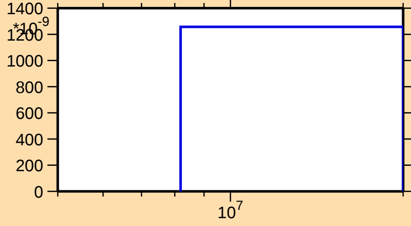
\sigma vs. E for ^{153}\text{Tm}(n,\text{nd})
