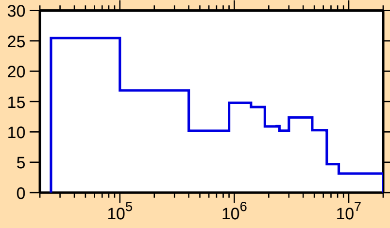
\Delta\sigma/\sigma vs. E for ^{153}\text{Tm}(n,\text{tot.})
