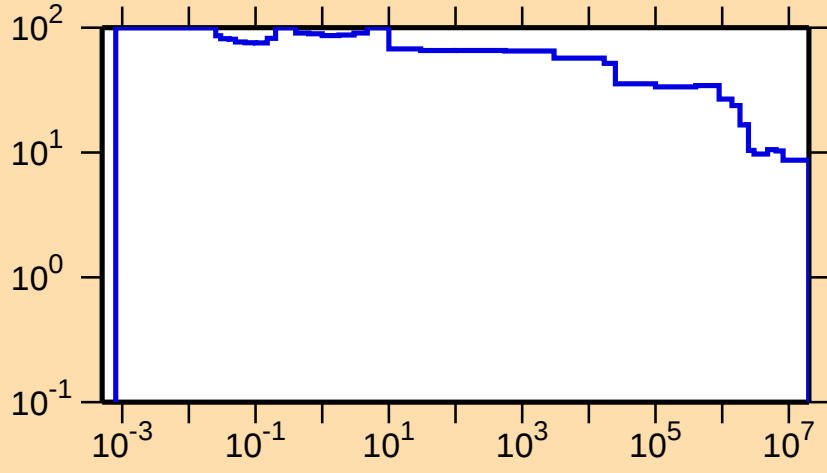
\Delta\sigma/\sigma vs. E for ^{153}\text{Tm}(n,\text{nonel.})
