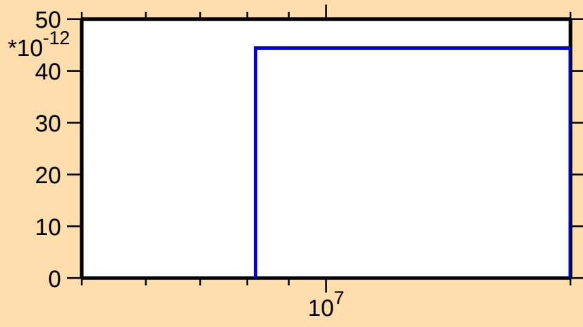
\sigma vs. E for ^{153}\text{Tm} (mt 34)
