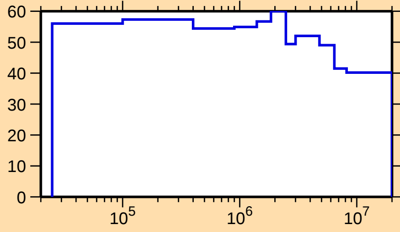
\Delta\sigma/\sigma vs. E for ^{153}\text{Tm}(n,n_1)
