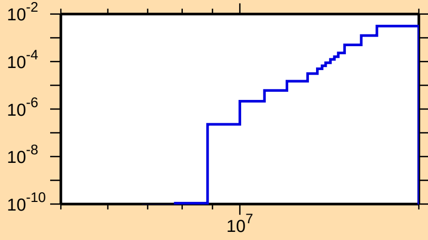
\sigma vs. E for ^{156}\text{Tm}(n,2n\alpha)
