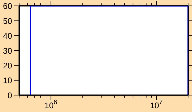
\Delta\sigma/\sigma vs. E for ^{156}\text{Tm}(n,n\text{cont.})
