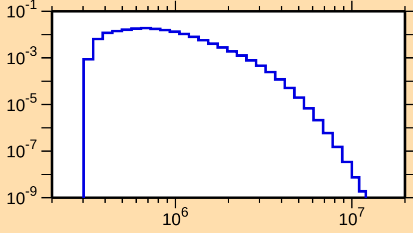
\sigma vs. E for ^{156}\text{Tm}(n,n_2)
