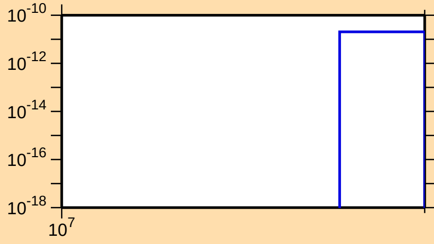
\sigma vs. E for ^{156}\text{Tm}(n,3n\alpha)
