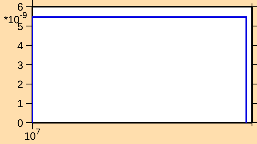
\sigma vs. E for ^{156}\text{Tm}(n,nt)
