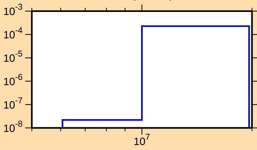
\sigma vs. E for ^{156}\text{Tm}(n,2n\alpha)
