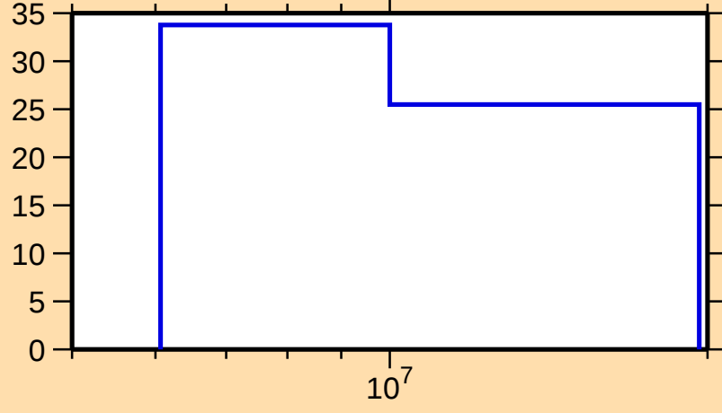
\Delta\sigma/\sigma vs. E for ^{156}\text{Tm}(n,\text{tot.})
