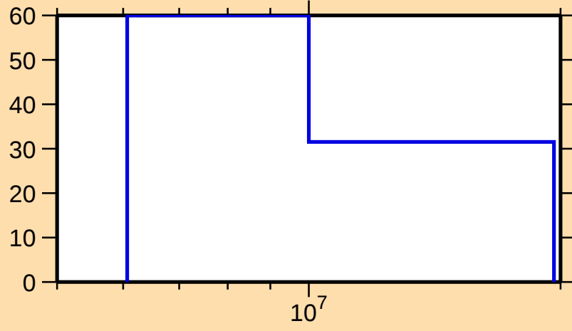
\Delta\sigma/\sigma vs. E for ^{156}\text{Tm}(n,\text{el.})
