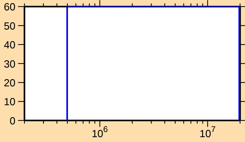
\Delta\sigma/\sigma vs. E for ^{156}\text{Tm}(n,n_1)
