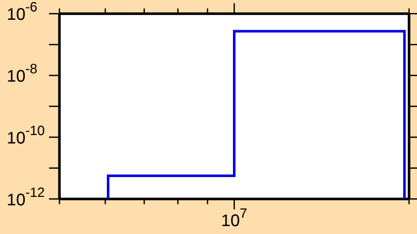
\sigma vs. E for ^{156}\text{Tm}(\text{mt117})
