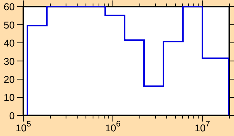
\Delta\sigma/\sigma vs. E for ^{156}\text{Tm}(n,\text{el.})
