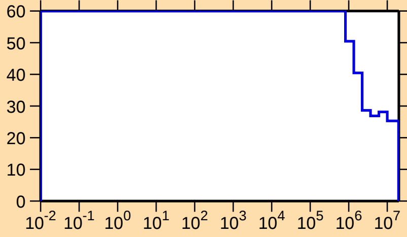
\Delta\sigma/\sigma vs. E for ^{156}\text{Tm}(n,\text{nonel.})
