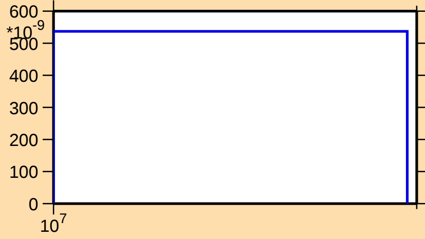
\sigma vs. E for ^{156}\text{Tm}(n,3n)
