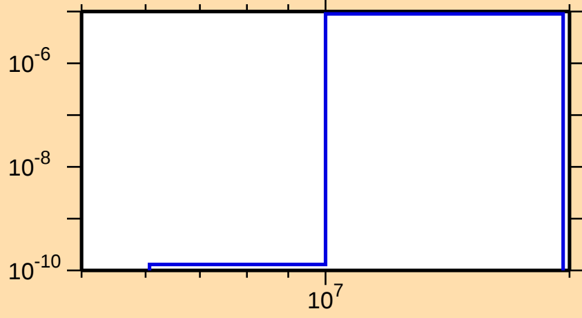
\sigma vs. E for ^{156}\text{Tm}(n,\text{He3})
