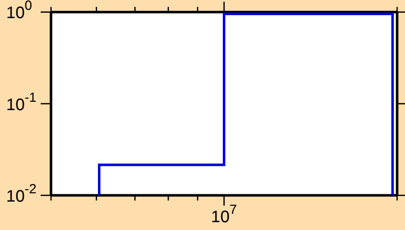
\sigma vs. E for ^{156}\text{Tm}(n,2n)
