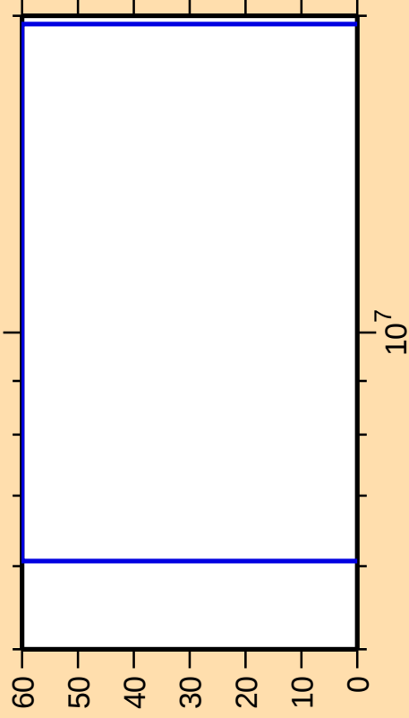
\Delta\sigma/\sigma vs. E for ^{156}\text{Tm}(\text{mt } 45)
