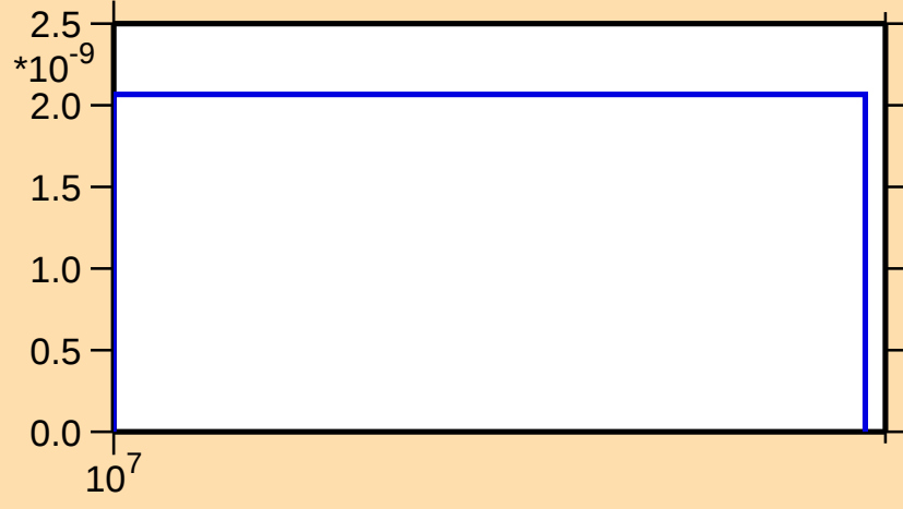
\sigma vs. E for ^{156}\text{Tm}(n,\text{pt})
