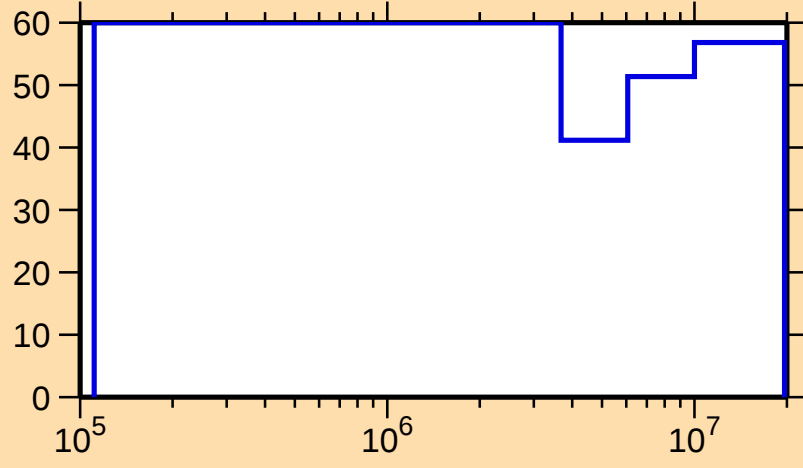
\Delta\sigma/\sigma vs. E for ^{156}\text{Tm}(n,\text{inel.})
