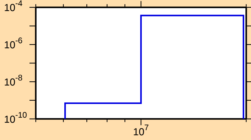
\sigma vs. E for ^{156}\text{Tm}(\text{mt } 45)
