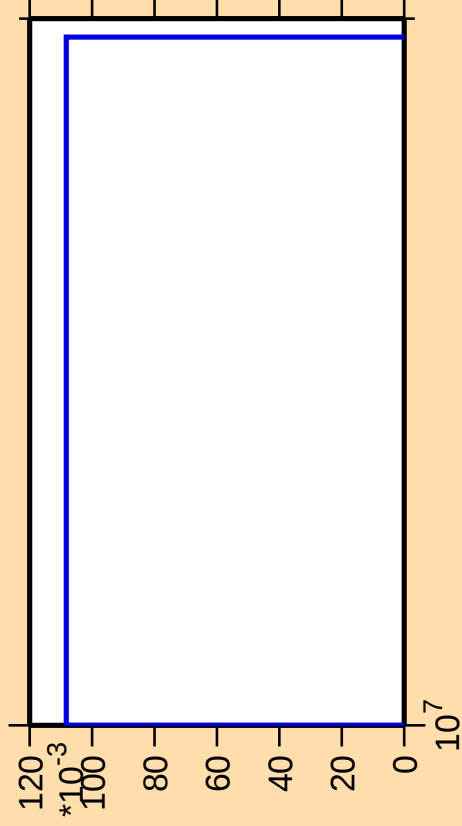
\Delta\sigma/\sigma vs. E for ^{156}\text{Tm}(n,3n\alpha)
