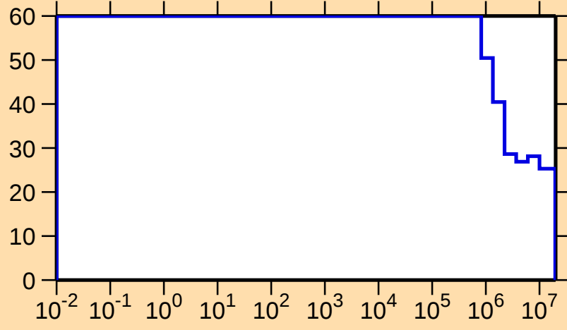
\Delta\sigma/\sigma vs. E for ^{156}\text{Tm}(n,\text{nonel.})
