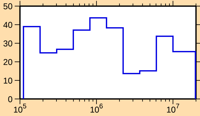
\Delta\sigma/\sigma vs. E for ^{156}\text{Tm}(n,\text{tot.})
