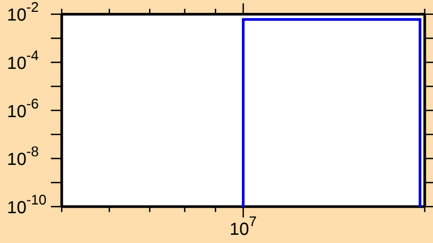
\sigma vs. E for ^{156}\text{Tm}(n,2np)
