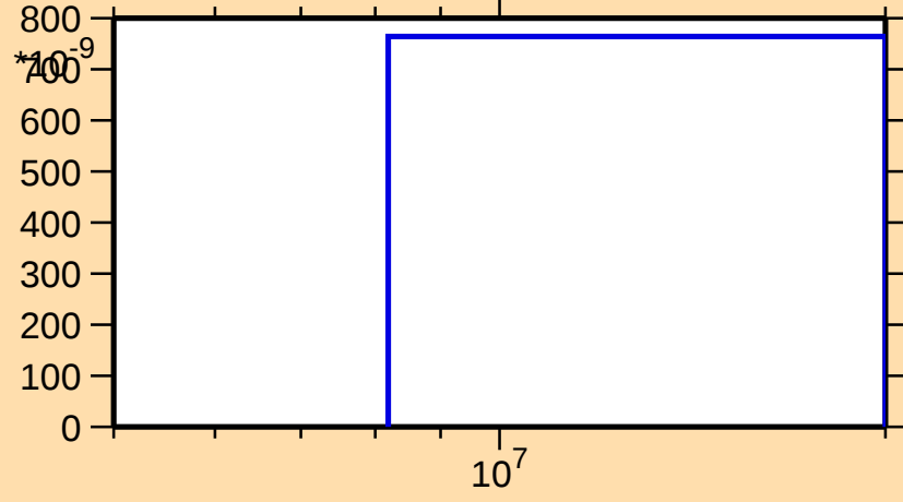
\sigma vs. E for ^{156}\text{Tm}(n,3n)
