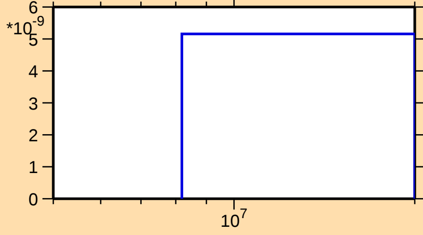
\sigma vs. E for ^{156}\text{Tm}(n,nt)
