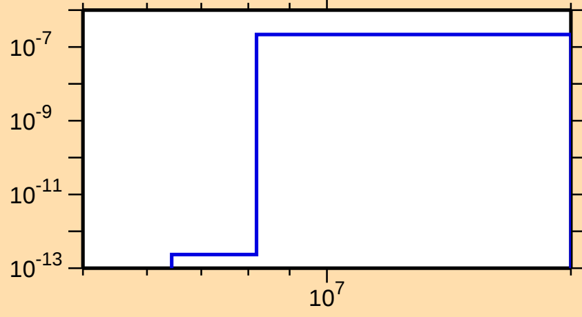
\sigma vs. E for ^{156}\text{Tm}(\text{mt117})
