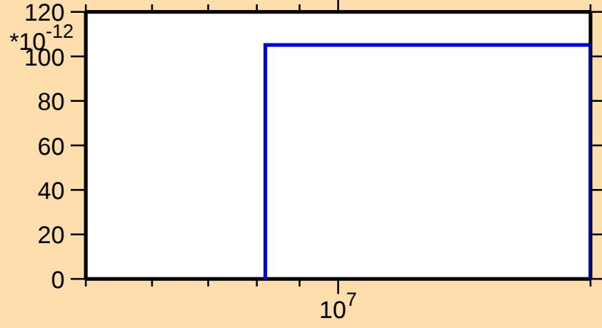
\sigma vs. E for ^{156}\text{Tm}(\text{mt } 34)
