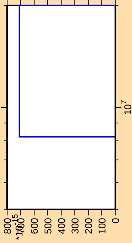
\Delta\sigma/\sigma vs. E for ^{156}\text{Tm}(\text{mt } 42)
