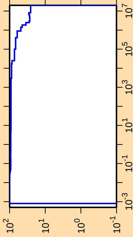
\Delta\sigma/\sigma vs. E for ^{156}\text{Tm}(n,\text{nonel.})
