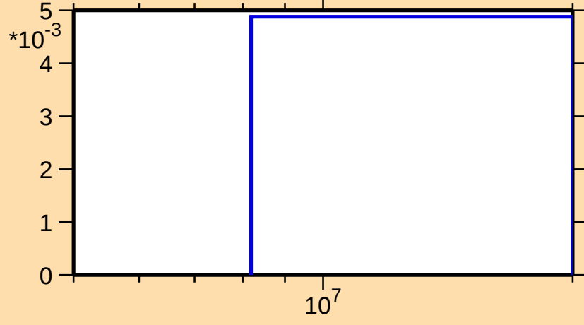
\sigma vs. E for ^{156}\text{Tm}(n,2np)
