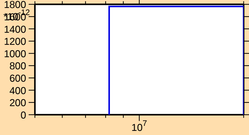
\sigma vs. E for ^{156}\text{Tm}(n,\text{pt})
