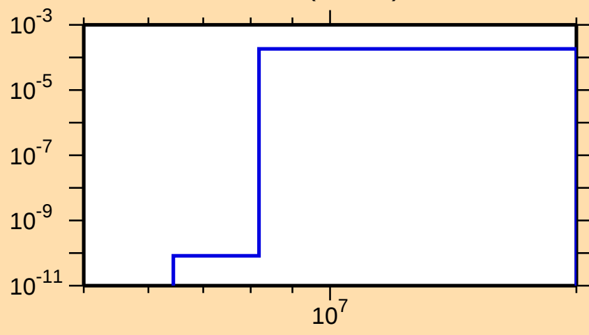
\sigma vs. E for ^{156}\text{Tm}(n,2n\alpha)
