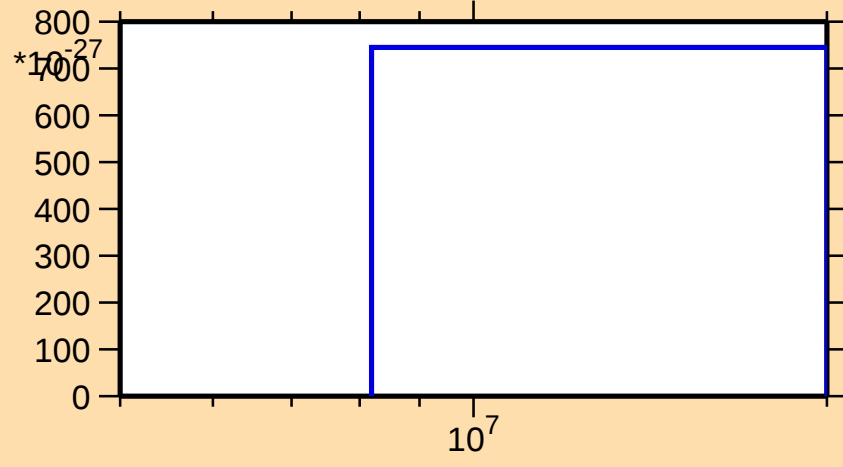
\sigma vs. E for ^{156}\text{Tm}(\text{mt } 42)
