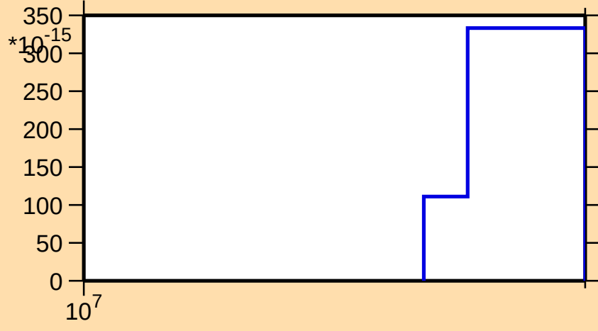
\sigma vs. E for ^{158}\text{Tm}(n,3n\alpha)
