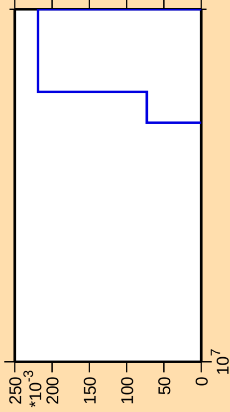
\Delta\sigma/\sigma vs. E for ^{158}\text{Tm}(n,3n\alpha)
