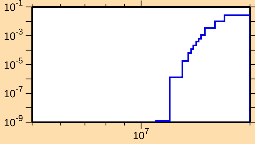
\sigma vs. E for ^{158}\text{Tm}(n,2np)
