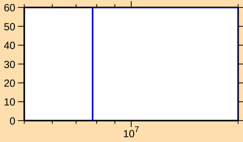
\Delta\sigma/\sigma vs. E for ^{158}\text{Tm}(n,2n)
