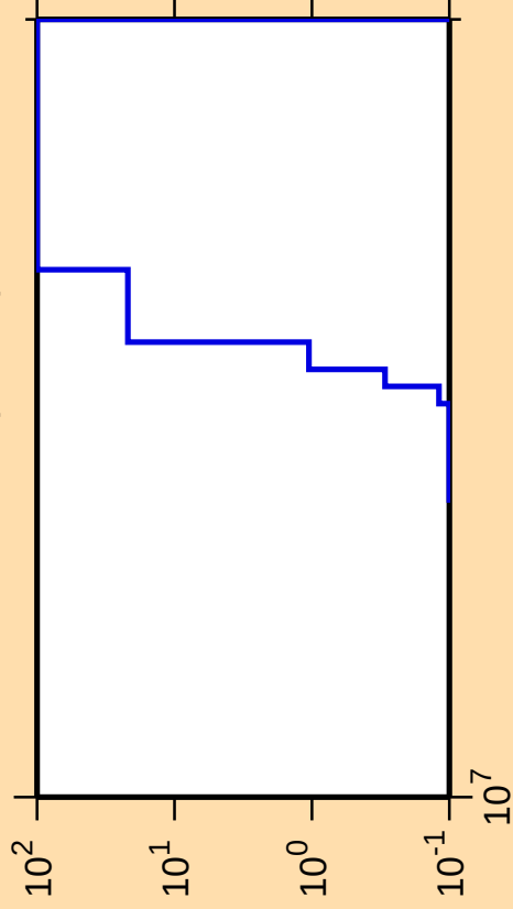
\Delta\sigma/\sigma vs. E for ^{158}\text{Tm}(\text{mt } 34)
