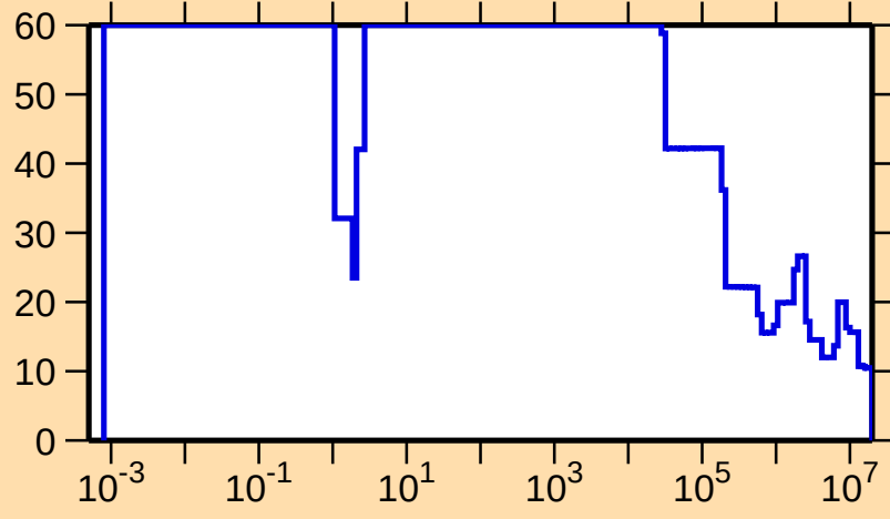
\Delta\sigma/\sigma vs. E for ^{158}\text{Tm}(n,\text{tot.})
