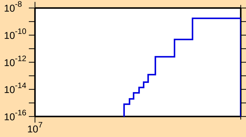
\sigma vs. E for ^{158}\text{Tm}(\text{mt } 34)
