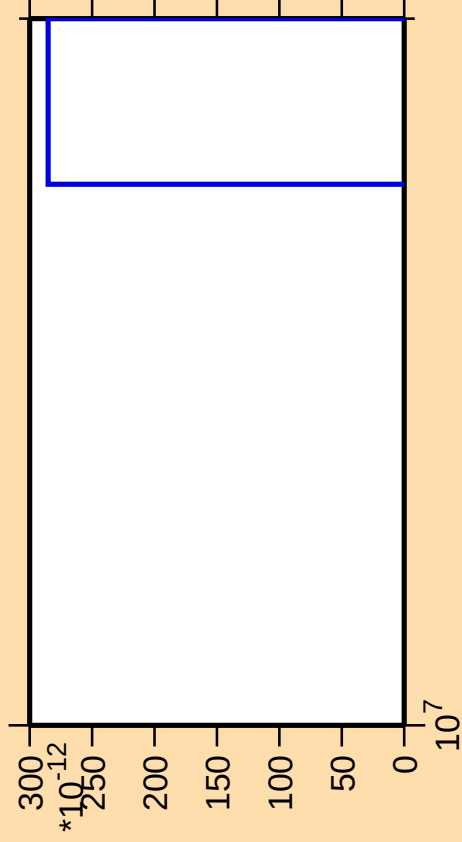
\Delta\sigma/\sigma vs. E for ^{158}\text{Tm}(\text{mt } 42)
