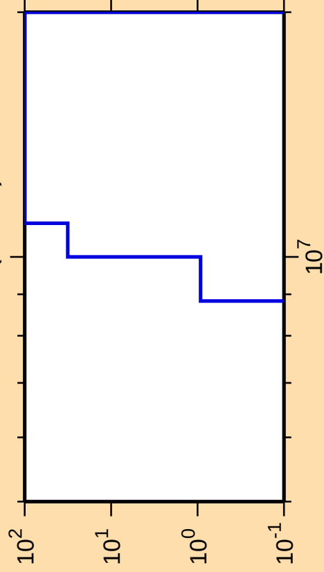
\Delta\sigma/\sigma vs. E for ^{158}\text{Tm}(\text{mt } 45)
