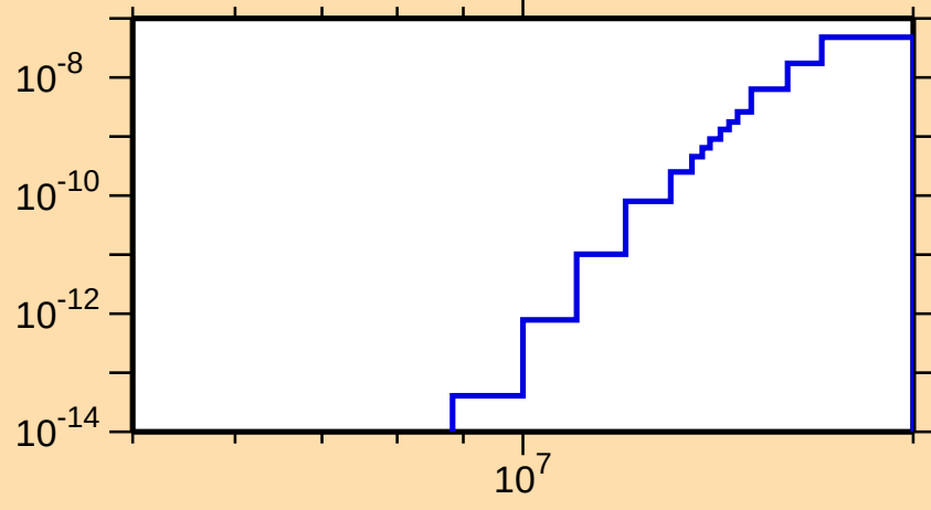
\sigma vs. E for ^{158}\text{Tm}(\text{mt117})
