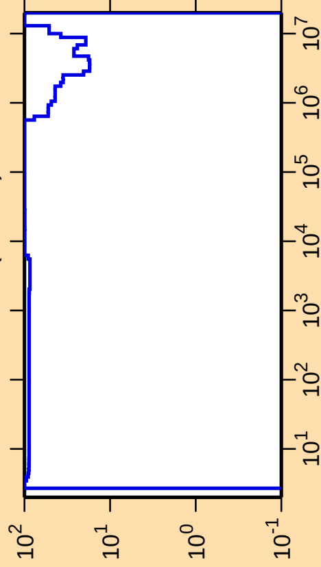
\Delta\sigma/\sigma vs. E for ^{158}\text{Tm}(n,\text{inel.})
