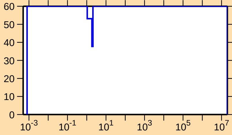
\Delta\sigma/\sigma vs. E for ^{158}\text{Tm}(n,\gamma)
