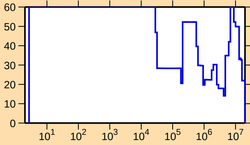
\Delta\sigma/\sigma vs. E for ^{158}\text{Tm}(n,\text{el.})
