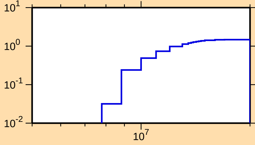
\sigma vs. E for ^{158}\text{Tm}(n,2n)
