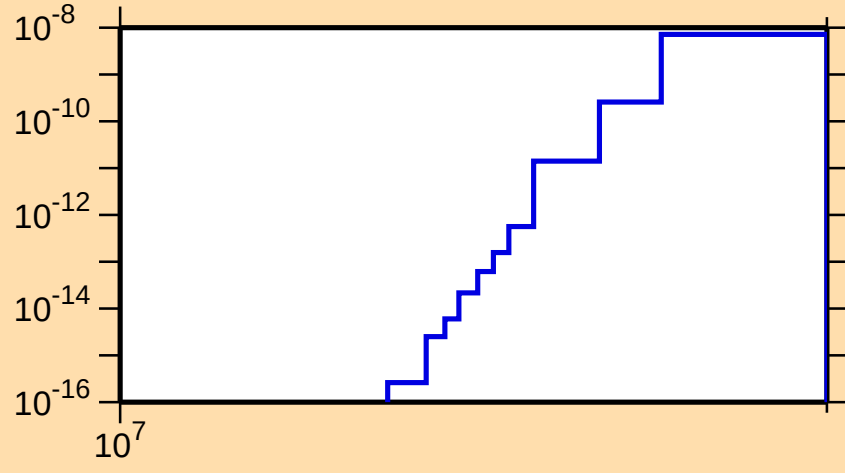
\sigma vs. E for ^{158}\text{Tm}(n,\text{pt})
