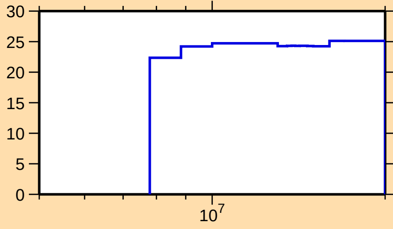
\Delta\sigma/\sigma vs. E for ^{158}\text{Tm}(n,\text{nonel.})
