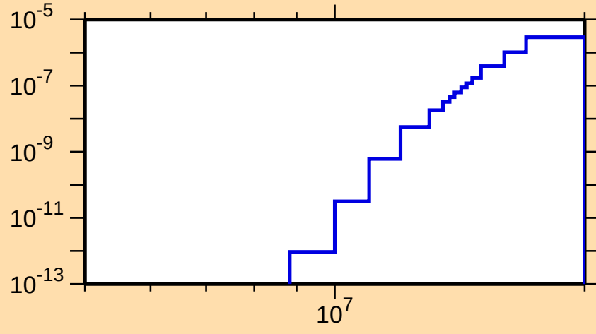
\sigma vs. E for ^{158}\text{Tm}(\text{mt } 45)
