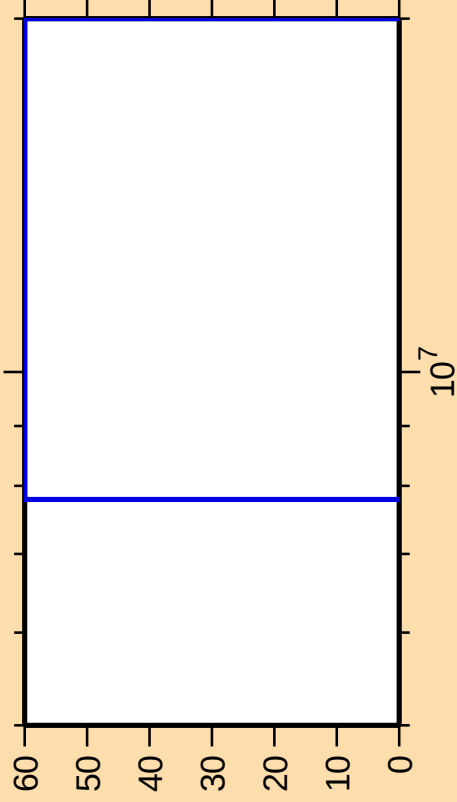
\Delta\sigma/\sigma vs. E for ^{158}\text{Tm}(n,p)
