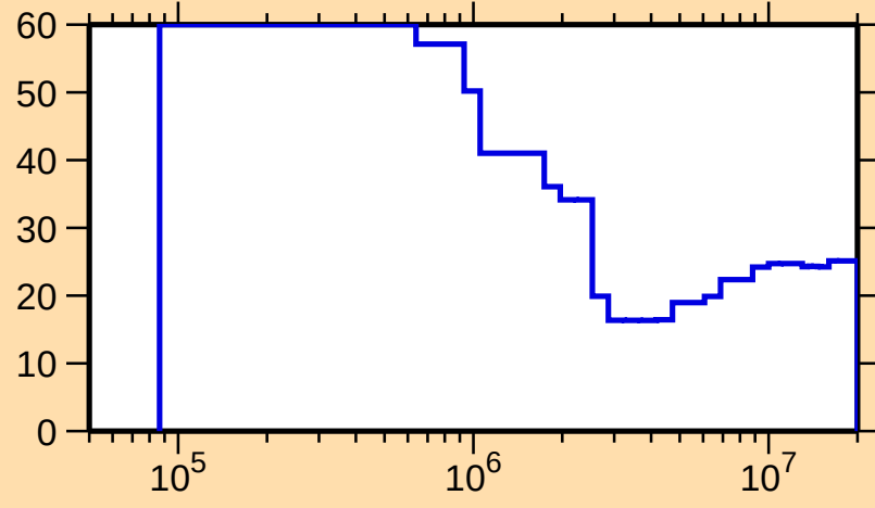
\Delta\sigma/\sigma vs. E for ^{158}\text{Tm}(n,\text{nonel.})
