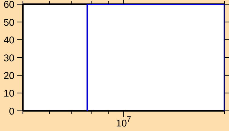
\Delta\sigma/\sigma vs. E for ^{158}\text{Tm}(n,2n)
