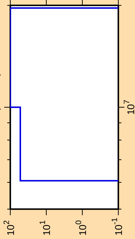
\Delta\sigma/\sigma vs. E for ^{158}\text{Tm}(n,\text{He}3)
