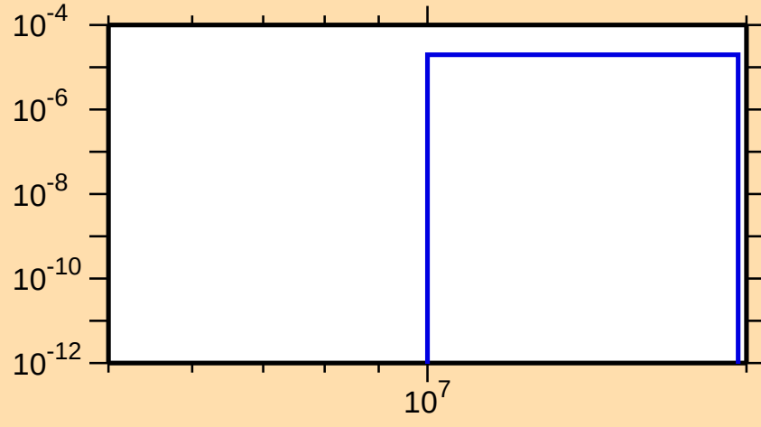
\sigma vs. E for ^{158}\text{Tm}(n,2n\alpha)
