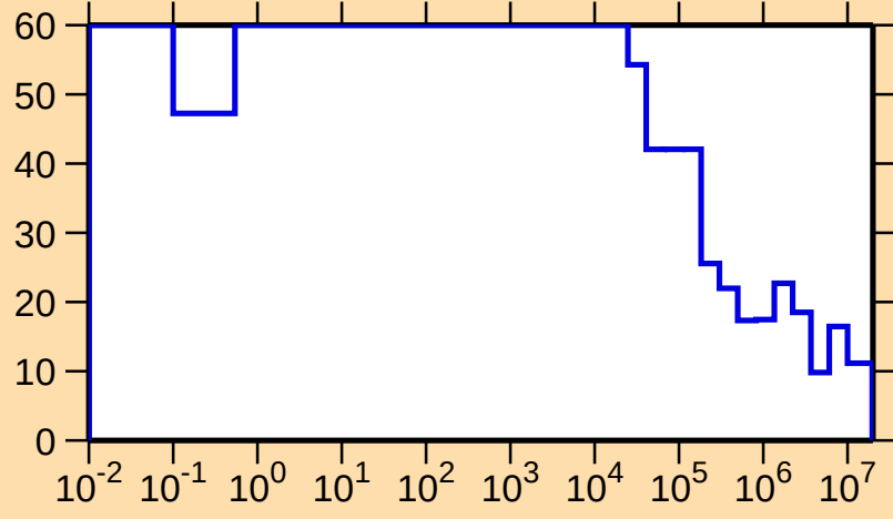
\Delta\sigma/\sigma vs. E for ^{158}\text{Tm}(n,\text{tot.})
