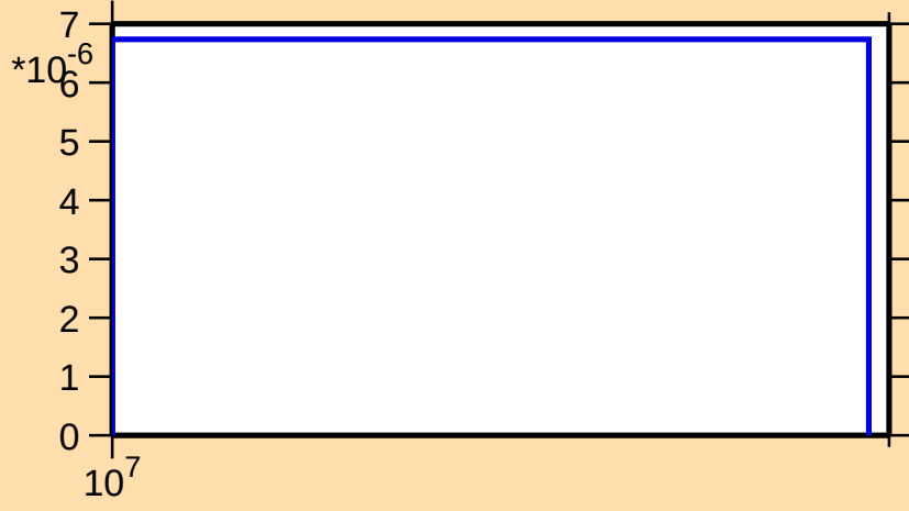
\sigma vs. E for ^{158}\text{Tm}(n,3n)
