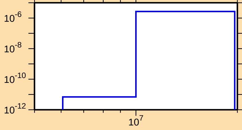
\sigma vs. E for ^{158}\text{Tm}(n,\text{He}3)
