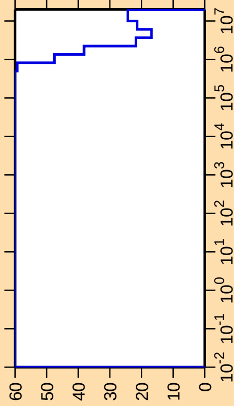
\Delta\sigma/\sigma vs. E for ^{158}\text{Tm}(n,\text{nonel.})
