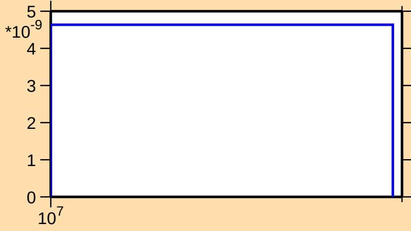
\sigma vs. E for ^{158}\text{Tm}(n,nt)
