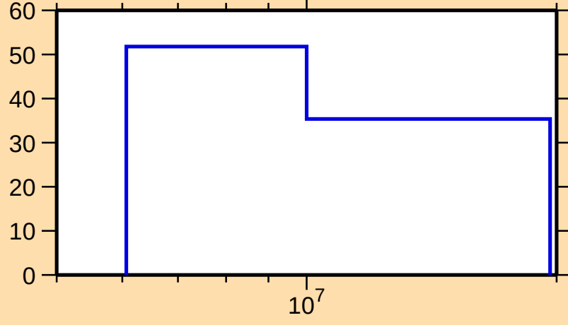
\Delta\sigma/\sigma vs. E for ^{158}\text{Tm}(n,\text{el.})
