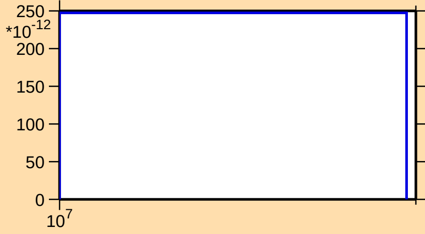
\sigma vs. E for ^{158}\text{Tm}(n,\text{pd})
