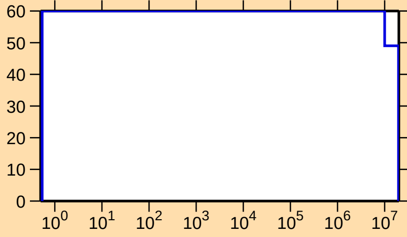
\Delta\sigma/\sigma vs. E for ^{158}\text{Tm}(n,n_1)
