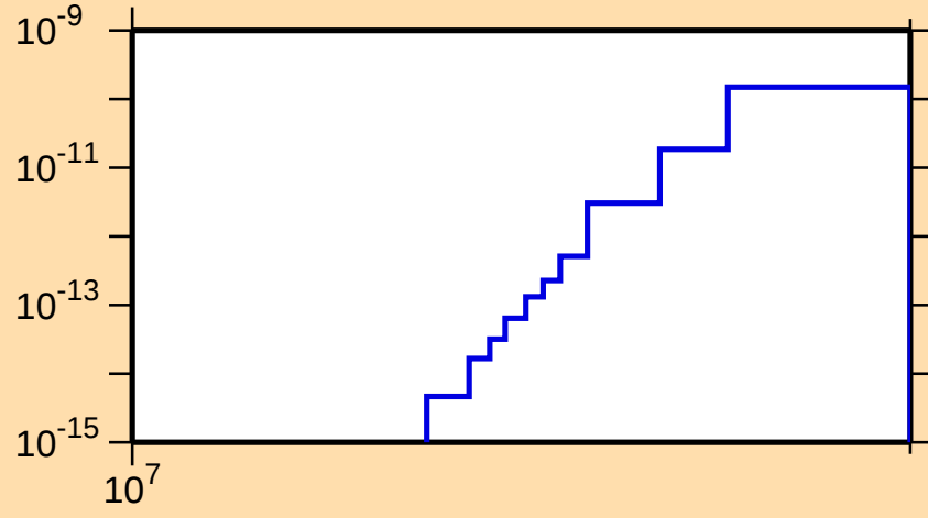
\sigma vs. E for ^{164}\text{Tm}(\text{mt } 45)
