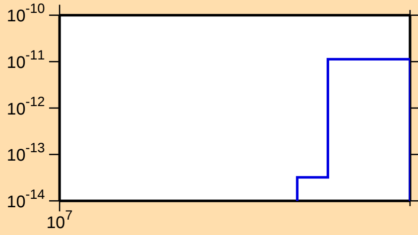
\sigma vs. E for ^{164}\text{Tm} (mt 34)
