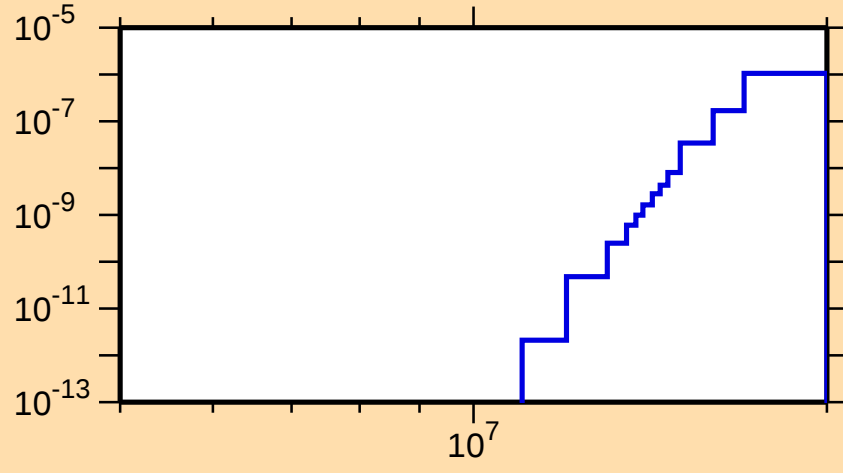
\sigma vs. E for ^{164}\text{Tm}(n,\text{He3})
