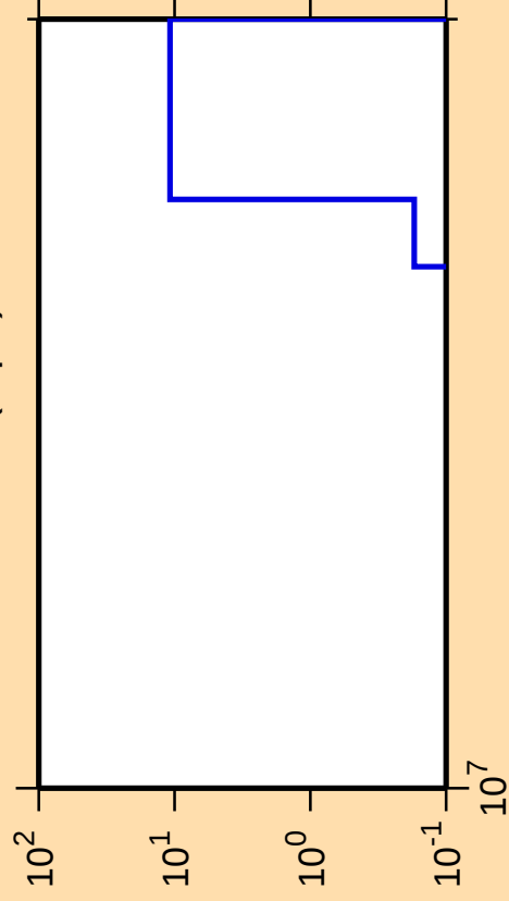
\Delta\sigma/\sigma vs. E for ^{164}\text{Tm}(n,\text{pd})
