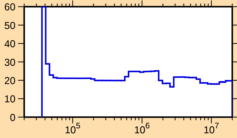
\Delta\sigma/\sigma vs. E for ^{164}\text{Tm}(n,n_1)
