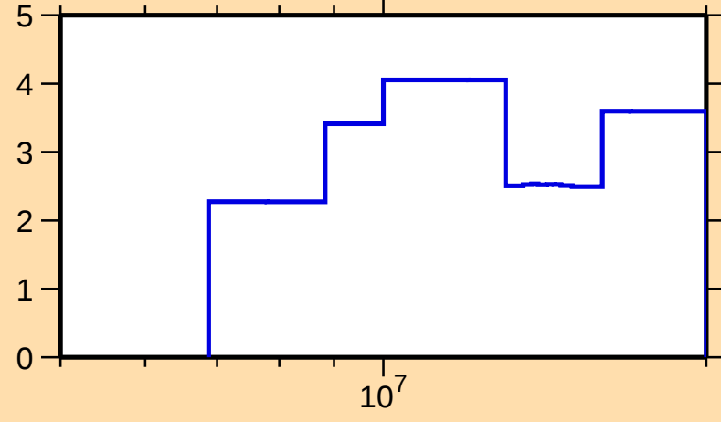
\Delta\sigma/\sigma vs. E for ^{164}\text{Tm}(n,\text{el.})
