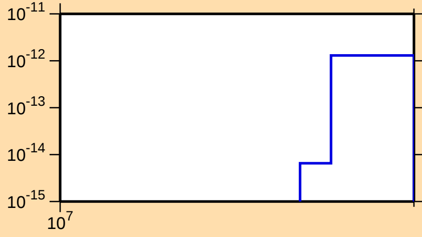
\sigma vs. E for ^{164}\text{Tm}(n,\text{pt})
