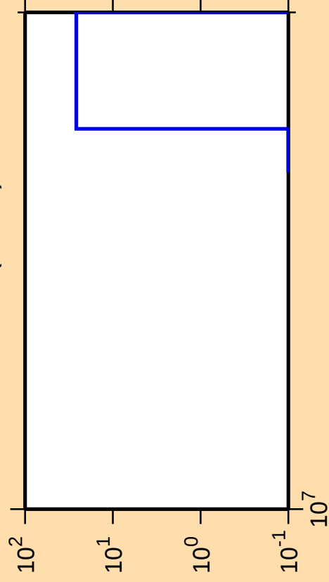
\Delta\sigma/\sigma vs. E for ^{164}\text{Tm} (mt 34)
