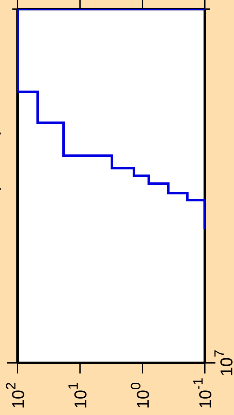
\Delta\sigma/\sigma vs. E for ^{164}\text{Tm}(\text{mt } 45)
