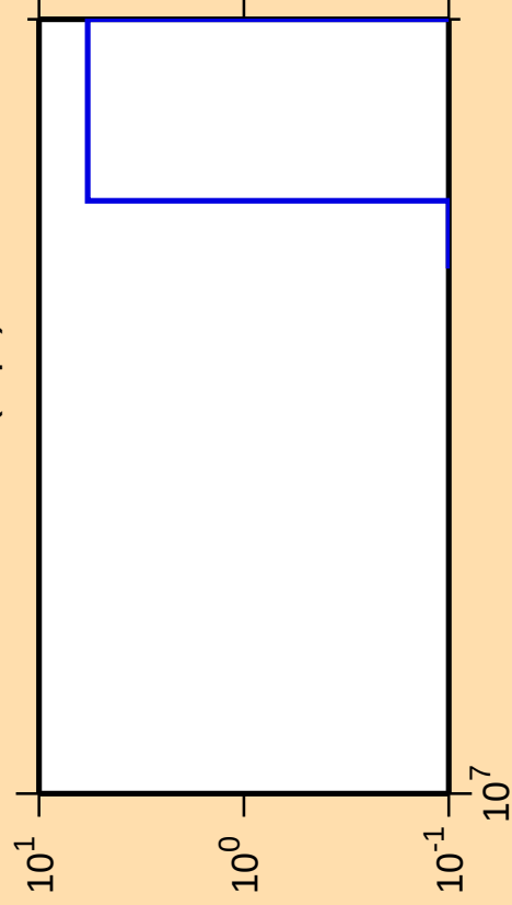
\Delta\sigma/\sigma vs. E for ^{164}\text{Tm}(n,\text{pt})
