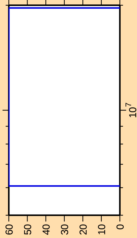
\Delta\sigma/\sigma vs. E for ^{164}\text{Tm}(n,p\alpha)
