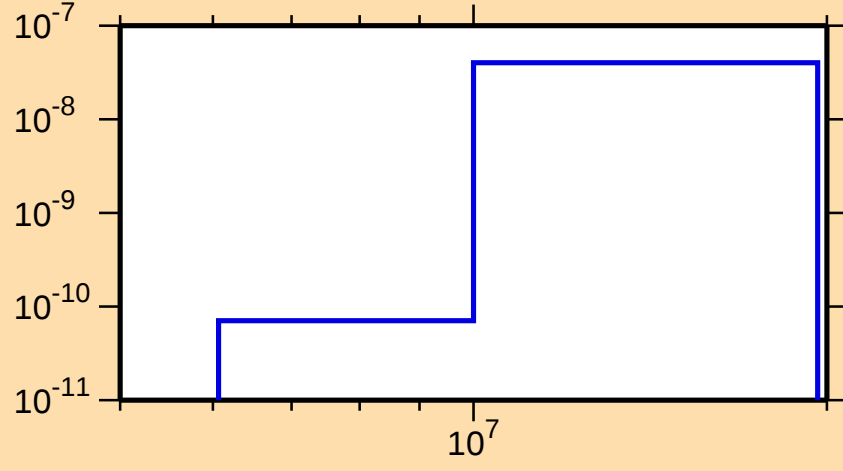
\sigma vs. E for ^{164}\text{Tm}(n,p\alpha)
