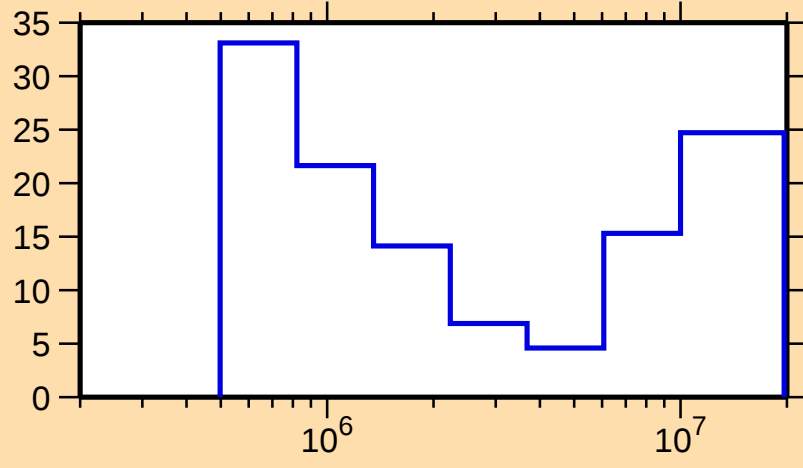
\Delta\sigma/\sigma vs. E for ^{164}\text{Tm}(n,n\text{cont.})
