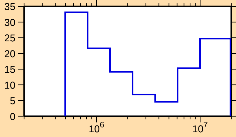
\Delta\sigma/\sigma vs. E for ^{164}\text{Tm}(n,ncont.)
