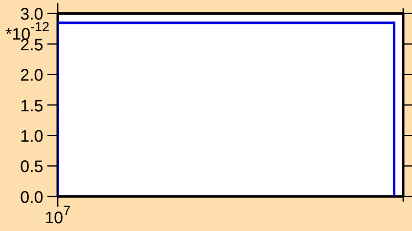
\sigma vs. E for ^{164}\text{Tm} (mt 45)
