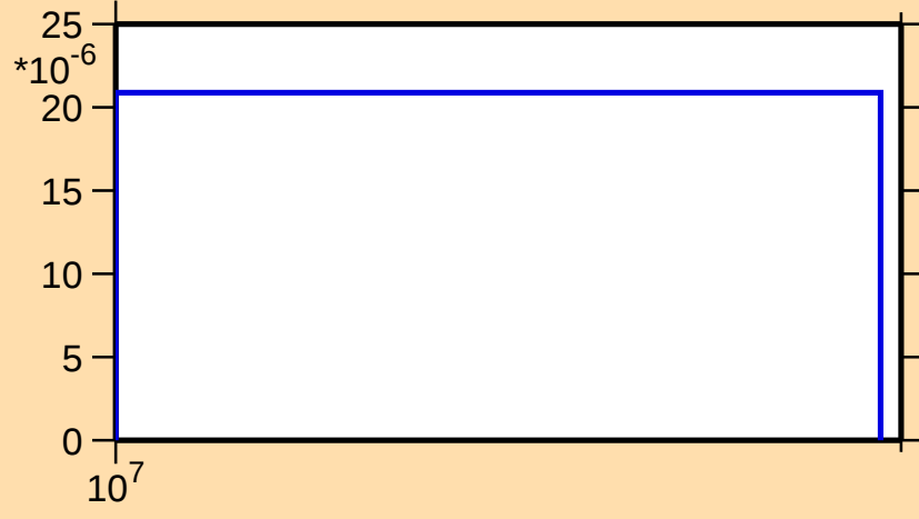
\sigma vs. E for ^{164}\text{Tm}(n,2np)
