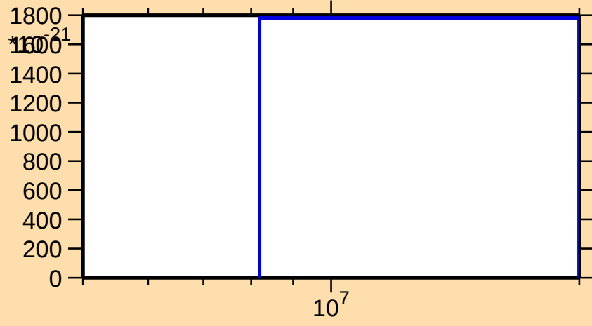
\sigma vs. E for ^{164}\text{Tm}(\text{mt } 11)
