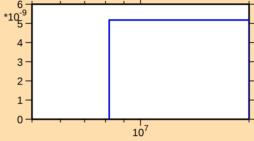
\sigma vs. E for ^{164}\text{Tm}(n,nt)
