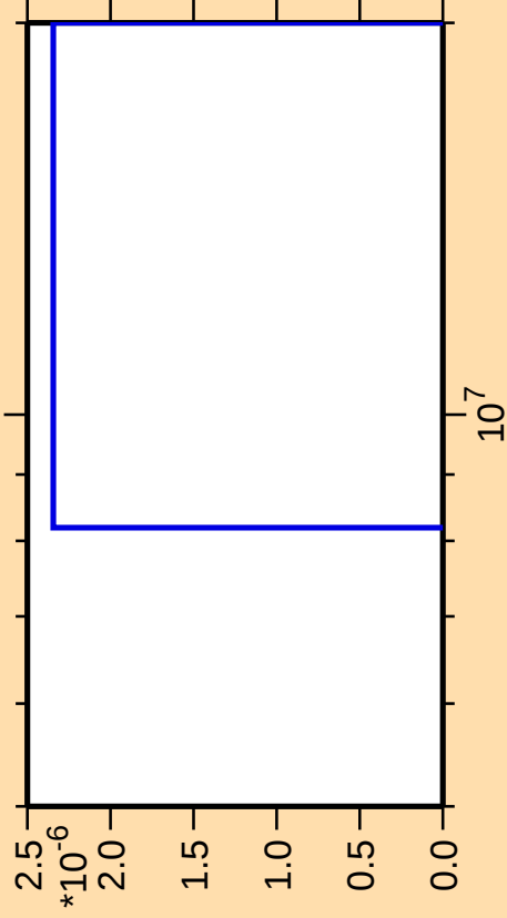
\Delta\sigma/\sigma vs. E for ^{164}\text{Tm}(\text{mt } 11)
