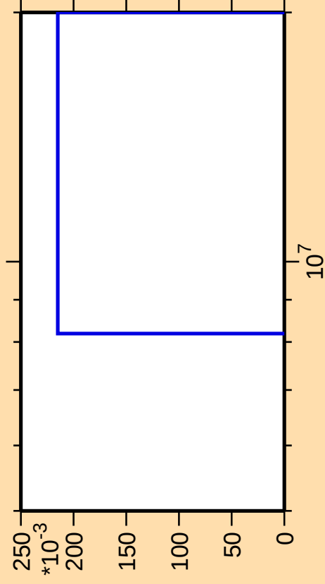
\Delta\sigma/\sigma vs. E for ^{164}\text{Tm}(\text{mt } 34)
