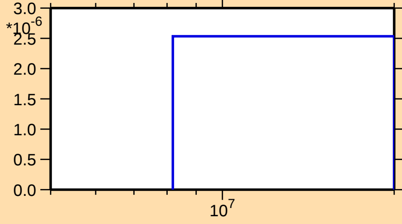
\sigma vs. E for ^{164}\text{Tm}(n,\text{nd})
