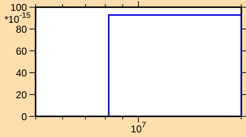
\sigma vs. E for ^{164}\text{Tm}(\text{mt } 34)
