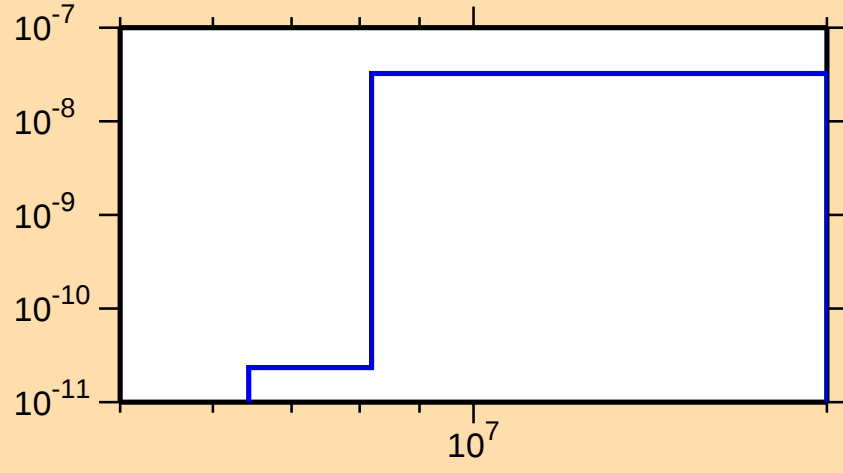
\sigma vs. E for ^{164}\text{Tm}(n,p\alpha)
