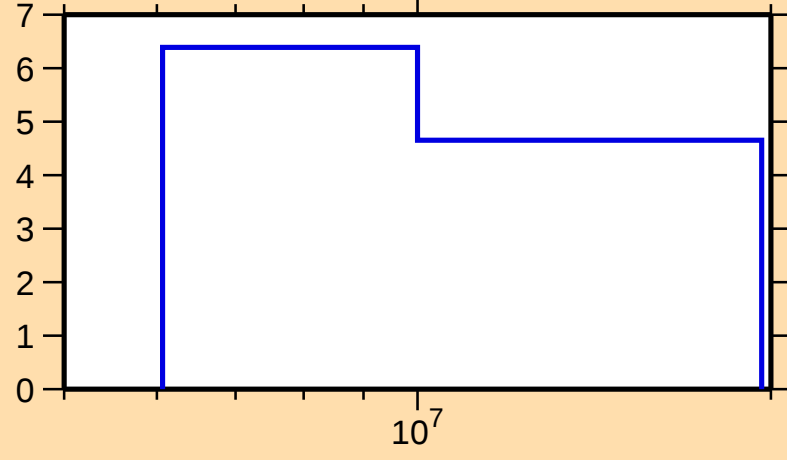
\Delta\sigma/\sigma vs. E for ^{165}\text{Tm}(n,\text{nonel.})
