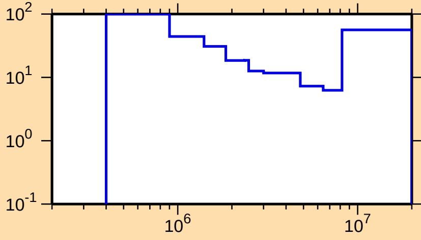
\Delta\sigma/\sigma vs. E for ^{165}\text{Tm}(n,n\text{cont.})
