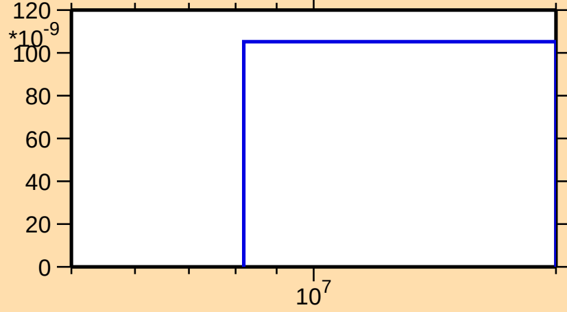
\sigma vs. E for ^{165}\text{Tm}(n,2np)
