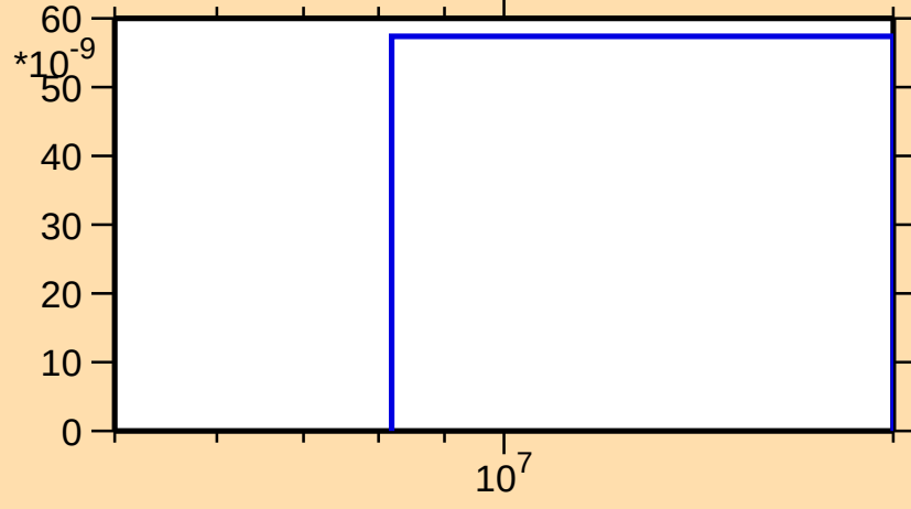
\sigma vs. E for ^{165}\text{Tm}(n,\text{nd})
