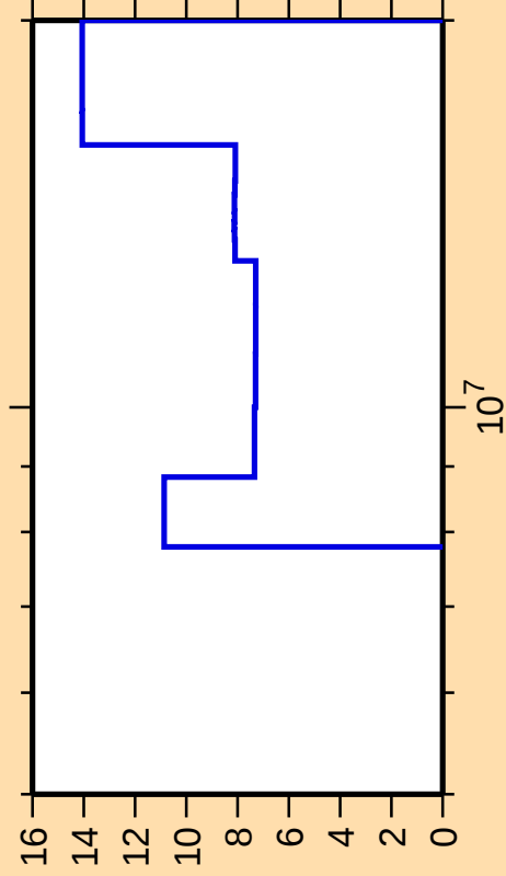
\Delta\sigma/\sigma vs. E for ^{169}\text{Tm}(n,2n)
