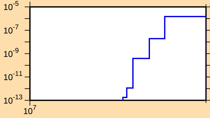
\sigma vs. E for ^{169}\text{Tm}(n,nt)
