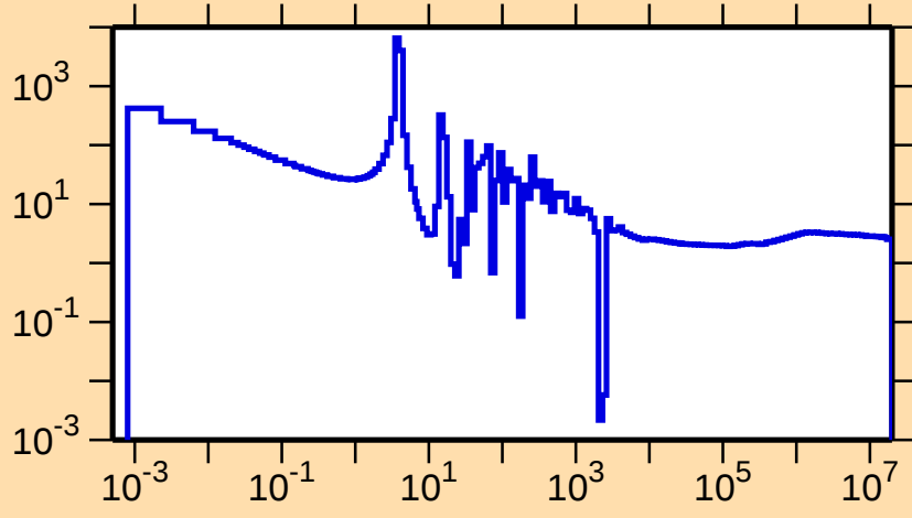
\sigma vs. E for ^{169}\text{Tm}(n,\text{nonel.})
