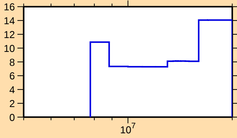
\Delta\sigma/\sigma vs. E for ^{169}\text{Tm}(n,2n)
