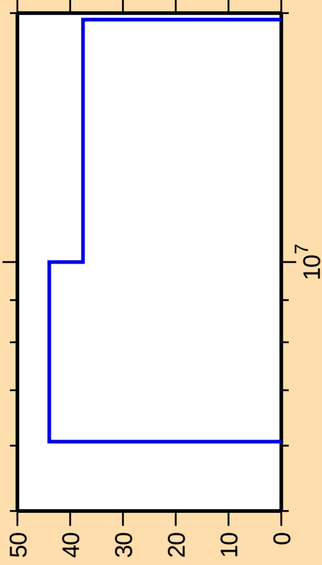
\Delta\sigma/\sigma vs. E for ^{169}\text{Tm}(n,p)
