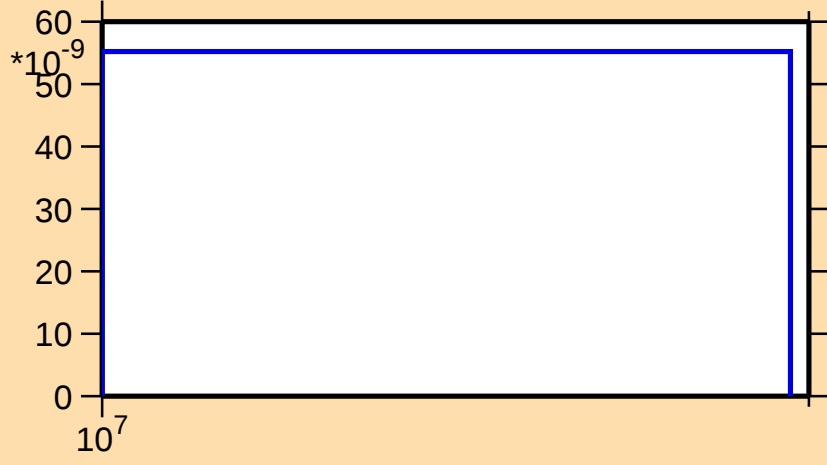
\sigma vs. E for ^{169}\text{Tm}(n,nd)
