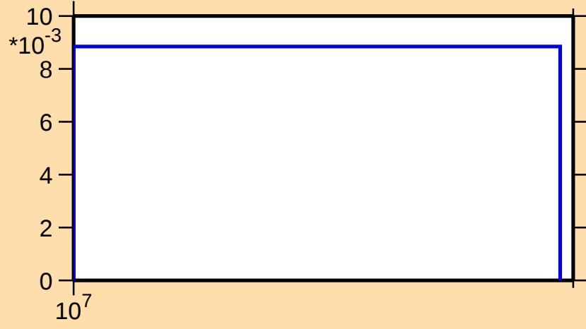
\sigma vs. E for ^{169}\text{Tm}(n,3n)
