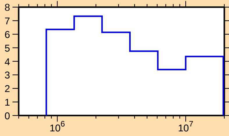
\Delta\sigma/\sigma vs. E for ^{169}\text{Tm}(n,\text{tot.})
