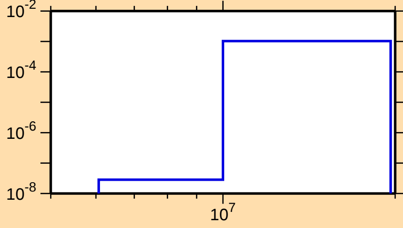
\sigma vs. E for ^{169}\text{Tm}(n,d)
