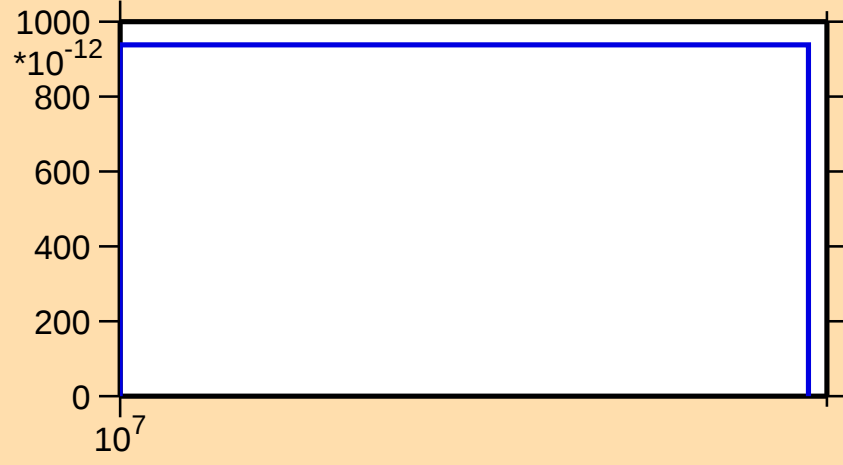
\sigma vs. E for ^{169}\text{Tm}(n,2n\alpha)
