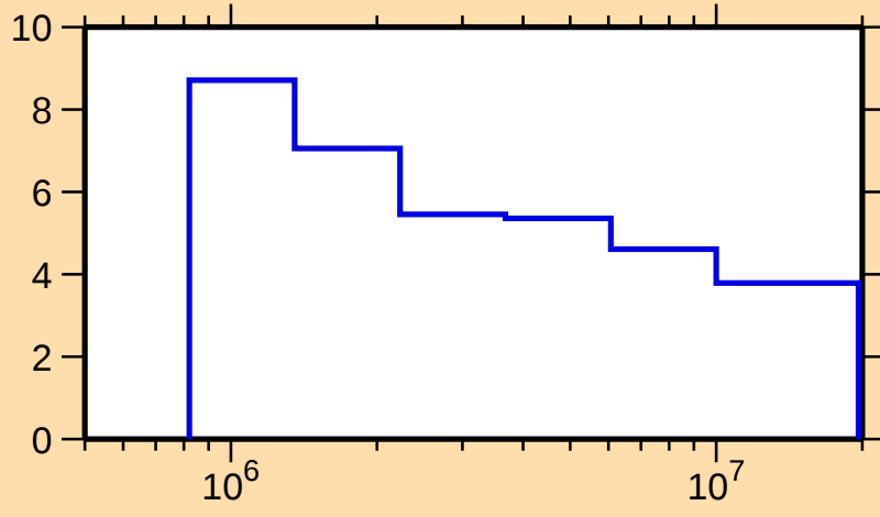
\Delta\sigma/\sigma vs. E for ^{169}\text{Tm}(n,\text{nonel.})
