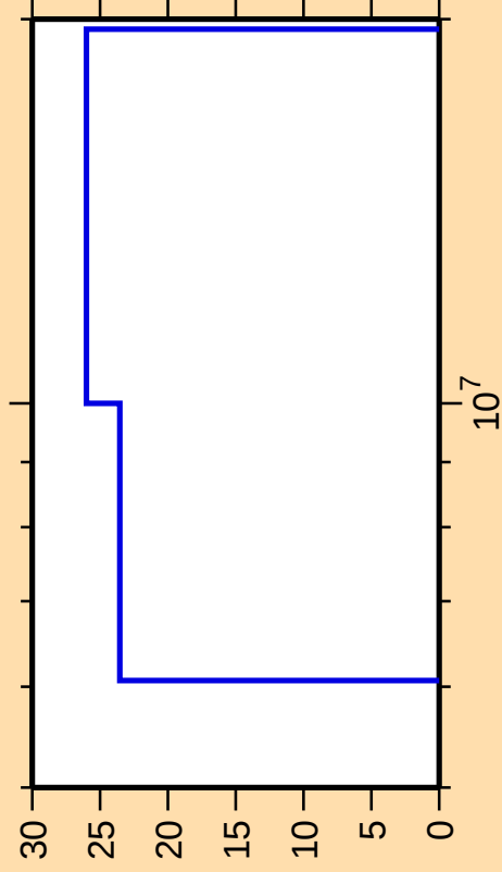
\Delta\sigma/\sigma vs. E for ^{169}\text{Tm}(n,\alpha)
