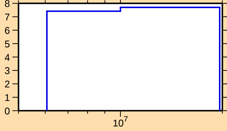
\Delta\sigma/\sigma vs. E for ^{169}\text{Tm}(n,2n)
