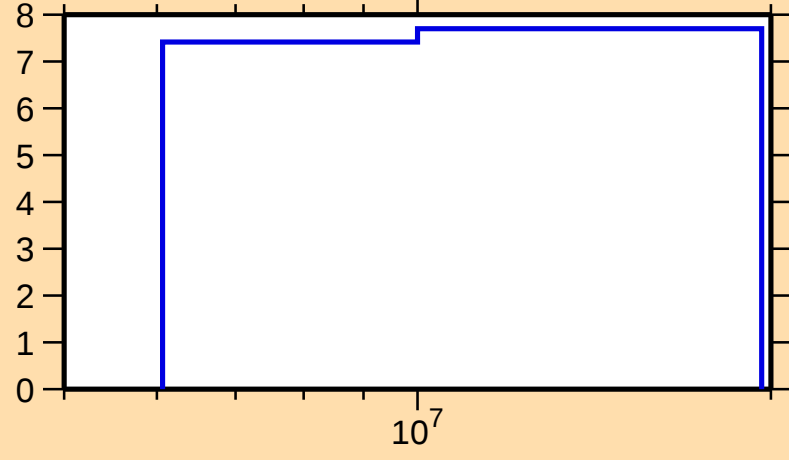
\Delta\sigma/\sigma vs. E for ^{169}\text{Tm}(n,2n)
