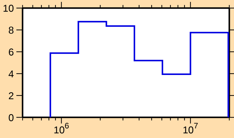
\Delta\sigma/\sigma vs. E for ^{169}\text{Tm}(n,\text{el.})
