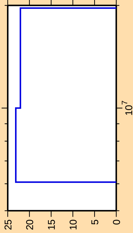
\Delta\sigma/\sigma vs. E for ^{169}\text{Tm}(n,n_1)
