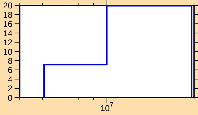
\Delta\sigma/\sigma vs. E for ^{169}\text{Tm}(n,\text{inel.})
