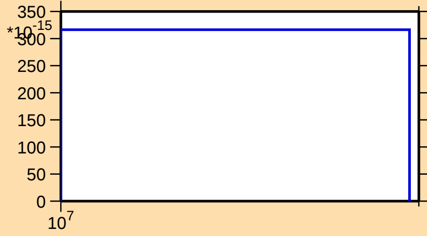
\sigma vs. E for ^{169}\text{Tm}(n,p\alpha)
