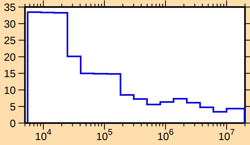
\Delta\sigma/\sigma vs. E for ^{169}\text{Tm}(n,\text{tot.})
