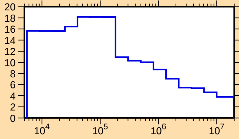
\Delta\sigma/\sigma vs. E for ^{169}\text{Tm}(n,\text{nonel.})
