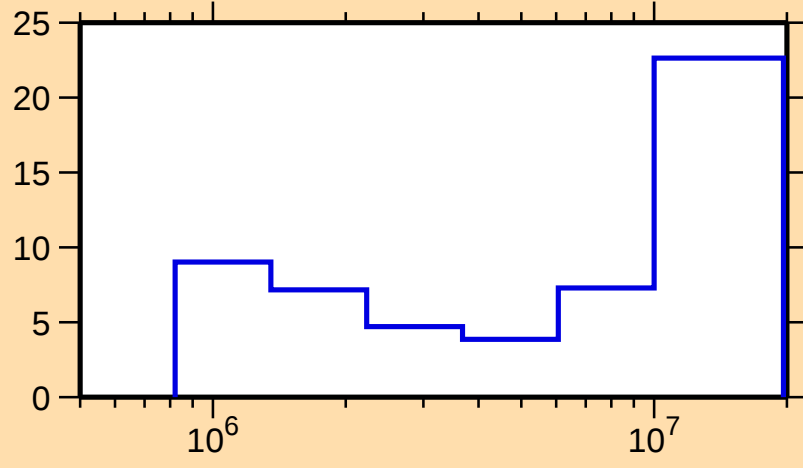
\Delta\sigma/\sigma vs. E for ^{169}\text{Tm}(n,n\text{cont.})
