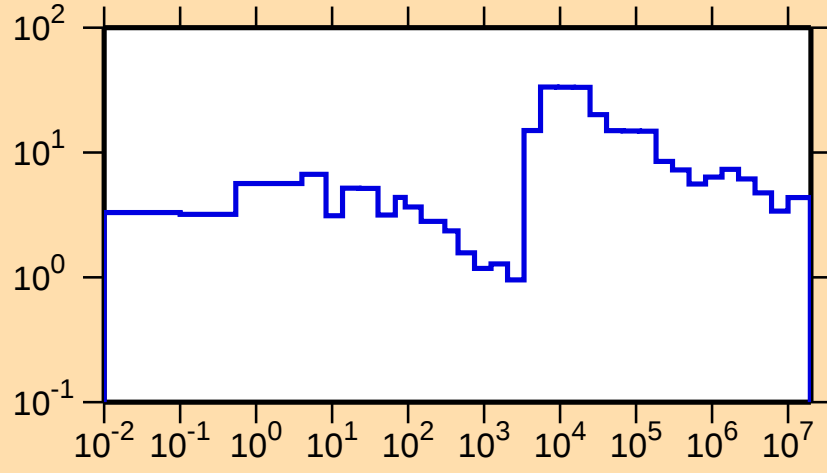
\Delta\sigma/\sigma vs. E for ^{169}\text{Tm}(n,\text{tot.})
