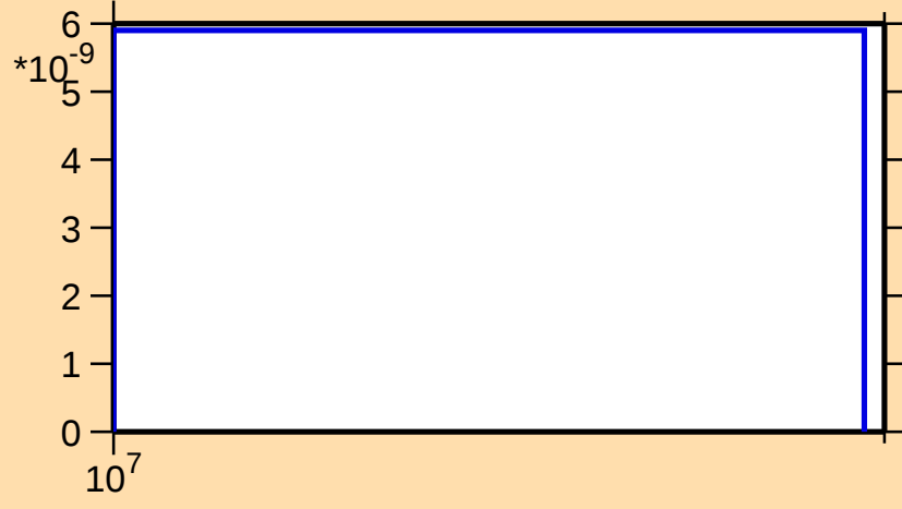
\sigma vs. E for ^{169}\text{Tm}(n,2np)
