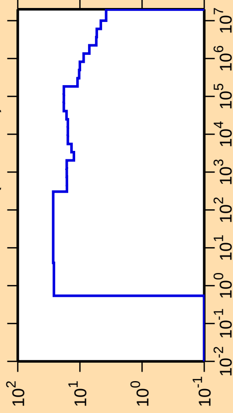
\Delta\sigma/\sigma vs. E for ^{169}\text{Tm}(n,\text{nonel.})
