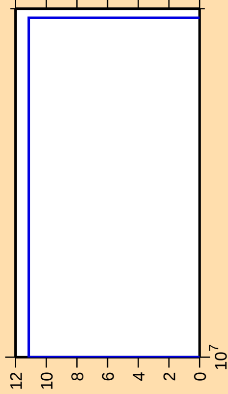
\Delta\sigma/\sigma vs. E for ^{169}\text{Tm}(n,3n)
