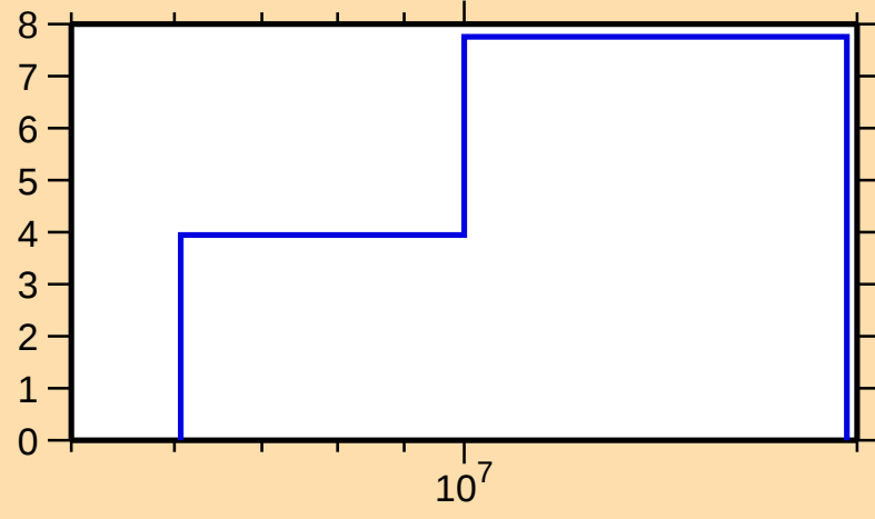
\Delta\sigma/\sigma vs. E for ^{169}\text{Tm}(n,\text{el.})
