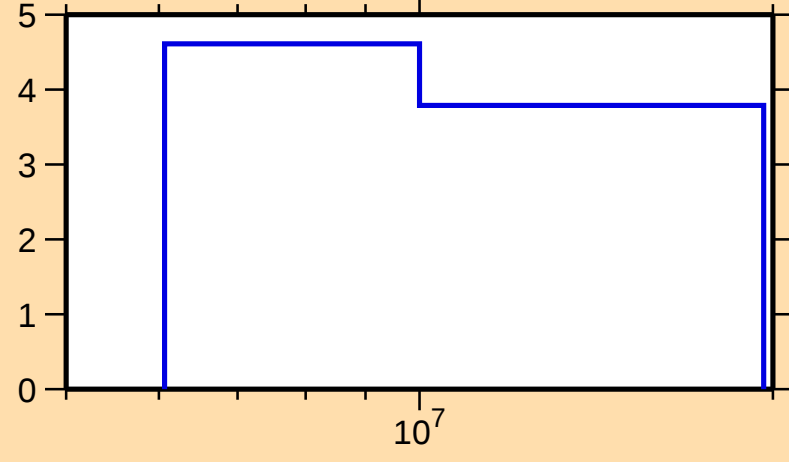
\Delta\sigma/\sigma vs. E for ^{169}\text{Tm}(n,\text{nonel.})
