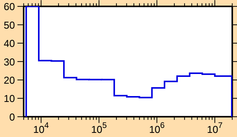
\Delta\sigma/\sigma vs. E for ^{169}\text{Tm}(n, n_1)
