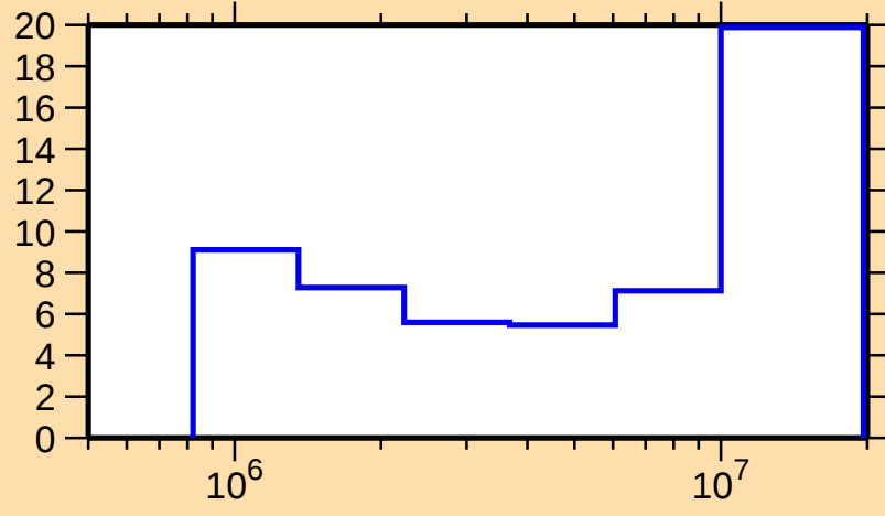
\Delta\sigma/\sigma vs. E for ^{169}\text{Tm}(n,\text{inel.})
