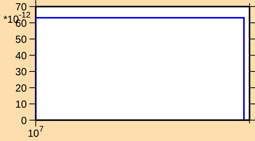
\sigma vs. E for ^{169}\text{Tm}(n,\text{He}3)
