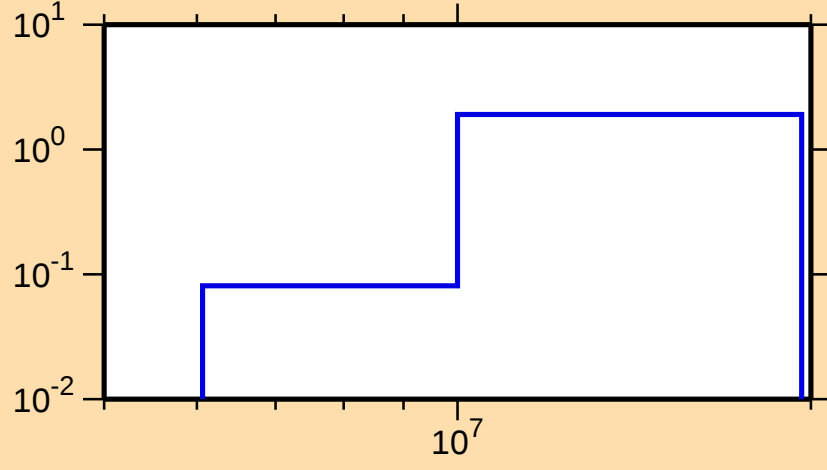
\sigma vs. E for ^{169}\text{Tm}(n,2n)
