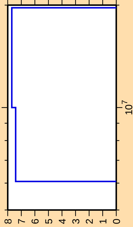
\Delta\sigma/\sigma vs. E for ^{169}\text{Tm}(n,2n)
