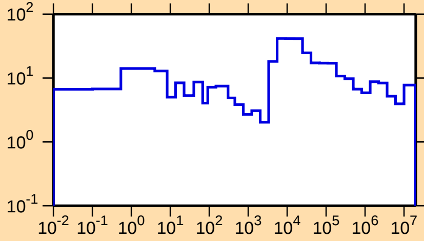
\Delta\sigma/\sigma vs. E for ^{169}\text{Tm}(n,\text{el.})
