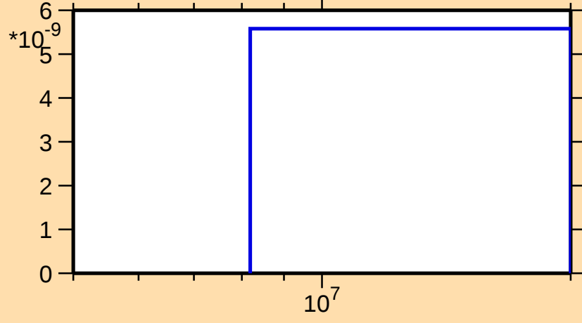
\sigma vs. E for ^{169}\text{Tm}(n,2np)
