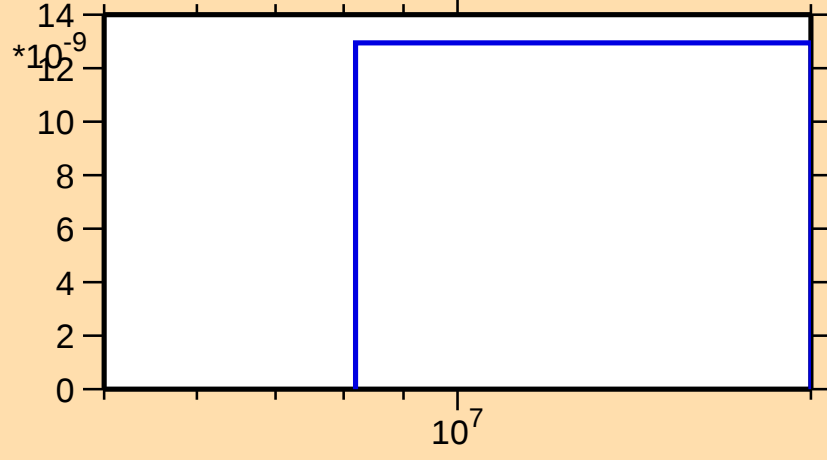
\sigma vs. E for ^{169}\text{Tm}(n,nt)
