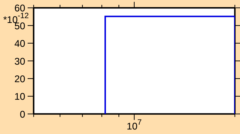
\sigma vs. E for ^{169}\text{Tm}(n,\text{He}3)
