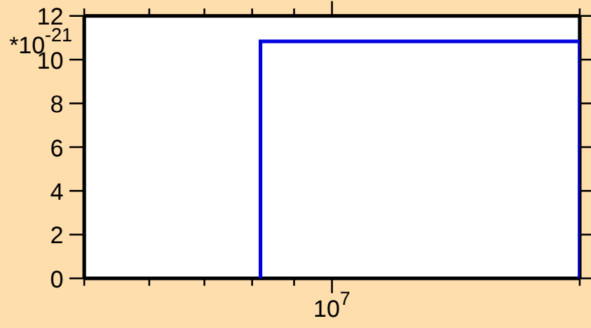
\sigma vs. E for ^{169}\text{Tm} (mt 42)
