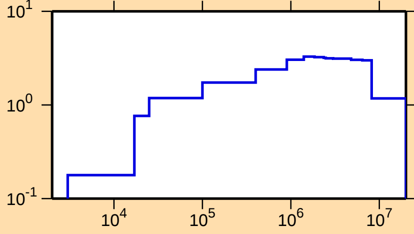
\sigma vs. E for ^{169}\text{Tm}(n,\text{inel.})
