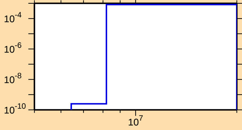
\sigma vs. E for ^{169}\text{Tm}(n,d)
