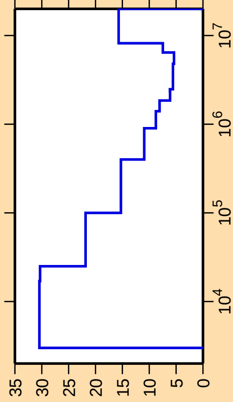
\Delta\sigma/\sigma vs. E for ^{169}\text{Tm}(n,\text{inel.})
