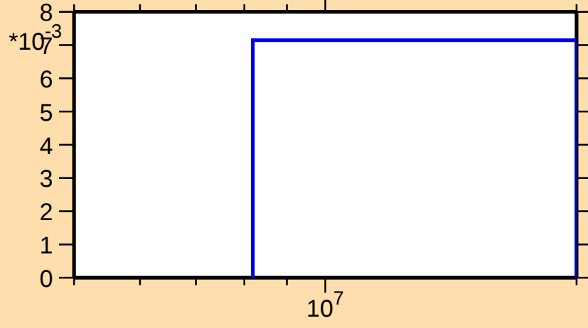
\sigma vs. E for ^{169}\text{Tm}(n,3n)
