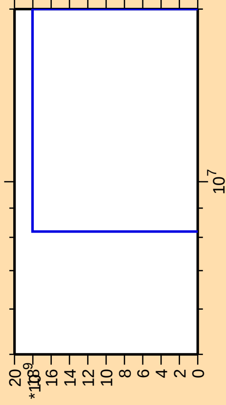
\Delta\sigma/\sigma vs. E for ^{169}\text{Tm} (mt 42)
