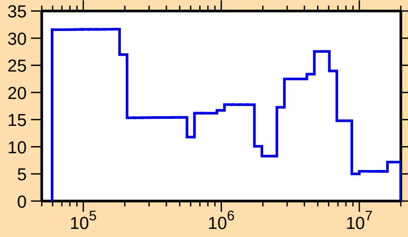
\Delta\sigma/\sigma vs. E for ^{172}\text{Tm}(n,\text{el.})
