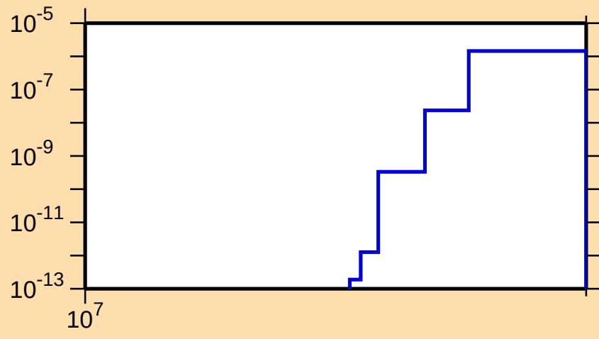
\sigma vs. E for ^{172}\text{Tm}(n,2np)
