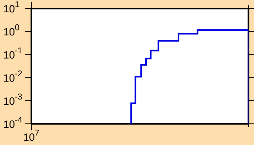
\sigma vs. E for ^{172}\text{Tm}(n,3n)
