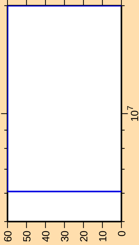
\Delta\sigma/\sigma vs. E for ^{172}\text{Tm}(n,\gamma)
