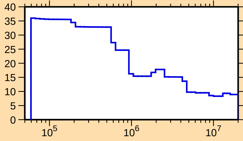
\Delta\sigma/\sigma vs. E for ^{172}\text{Tm}(n,\text{nonel.})
