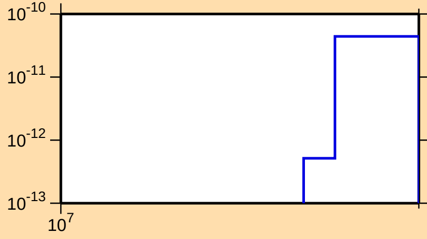
\sigma vs. E for ^{172}\text{Tm}(n,\text{He3})
