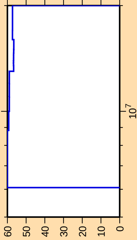
\Delta\sigma/\sigma vs. E for ^{172}\text{Tm}(n,p)
