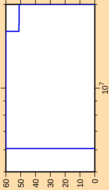
\Delta\sigma/\sigma vs. E for ^{172}\text{Tm}(n,\alpha)
