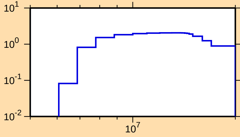
\sigma vs. E for ^{172}\text{Tm}(n,2n)
