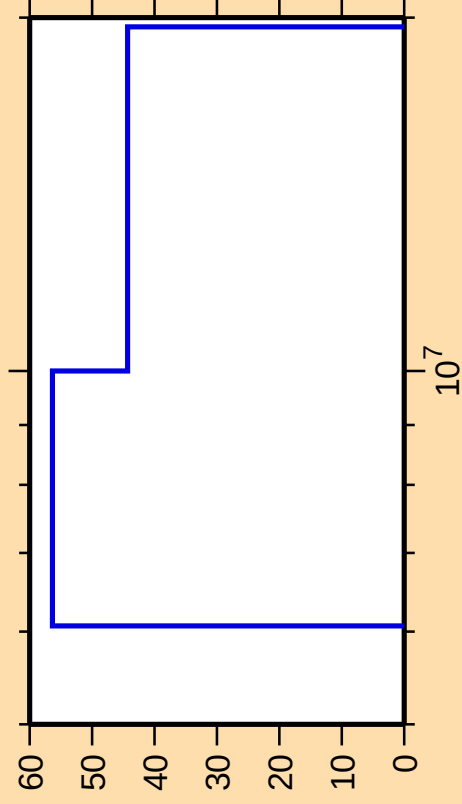
\Delta\sigma/\sigma vs. E for ^{172}\text{Tm}(n,n_1)
