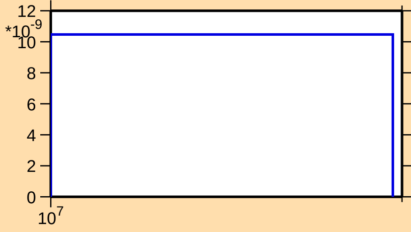
\sigma vs. E for ^{172}\text{Tm}(n,nt)
