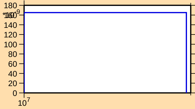
\sigma vs. E for ^{172}\text{Tm}(n,nd)
