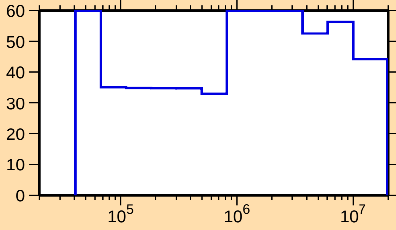
\Delta\sigma/\sigma vs. E for ^{172}\text{Tm}(n,n_1)
