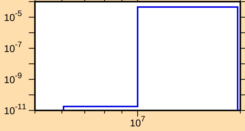
\sigma vs. E for ^{172}\text{Tm}(n,t)
