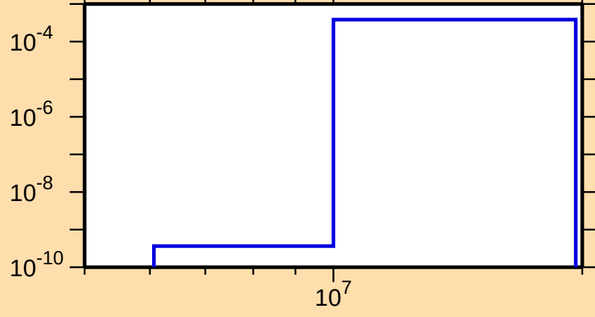
\sigma vs. E for ^{172}\text{Tm}(n,d)
