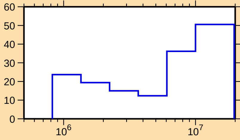
\Delta\sigma/\sigma vs. E for ^{172}\text{Tm}(n,n\text{cont.})
