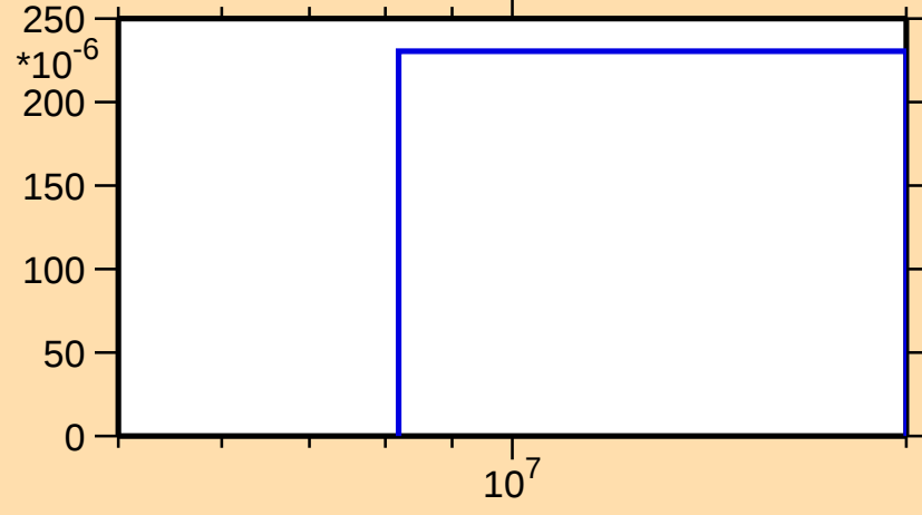
\sigma vs. E for ^{172}\text{Tm}(n,np)
