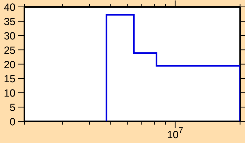
\Delta\sigma/\sigma vs. E for ^{172}\text{Tm}(n,2n)
