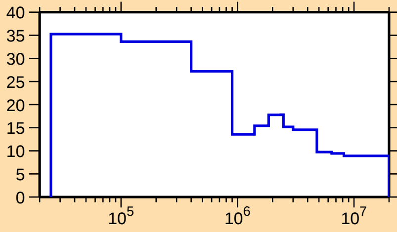
\Delta\sigma/\sigma vs. E for ^{172}\text{Tm}(n,\text{nonel.})
