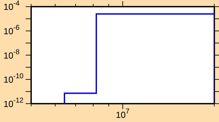
\sigma vs. E for ^{172}\text{Tm}(n,n\alpha)
