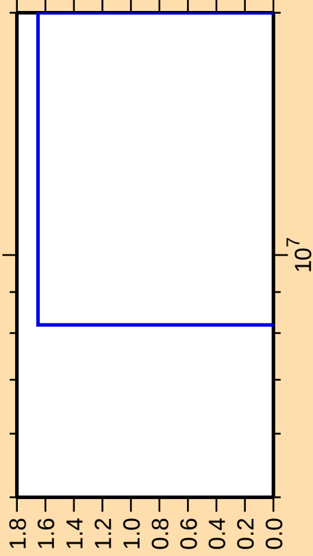
\Delta\sigma/\sigma vs. E for ^{172}\text{Tm}(n,\text{He}3)
