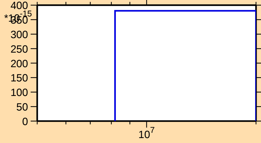
\sigma vs. E for ^{172}\text{Tm}(n,\text{He}3)
