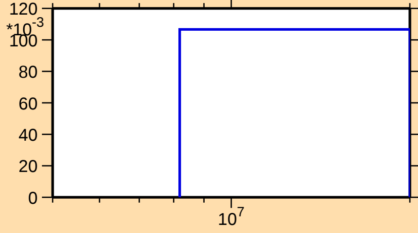
\sigma vs. E for ^{172}\text{Tm}(n,3n)
