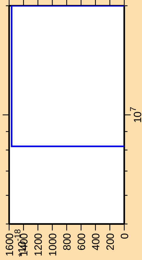
\Delta\sigma/\sigma vs. E for ^{172}\text{Tm} (mt 42)
