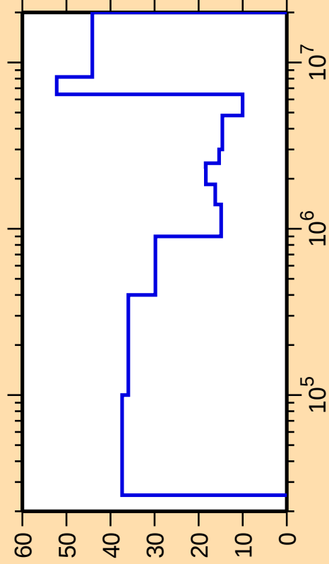
\Delta\sigma/\sigma vs. E for ^{172}\text{Tm}(n,\text{inel.})
