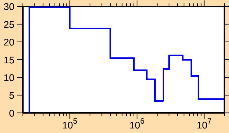
\Delta\sigma/\sigma vs. E for ^{172}\text{Tm}(n,\text{tot.})
