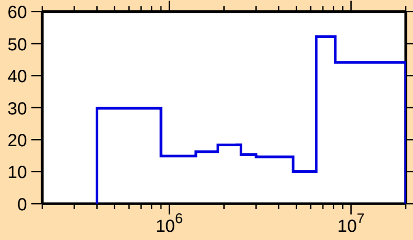
\Delta\sigma/\sigma vs. E for ^{172}\text{Tm}(n,\text{inel.})
