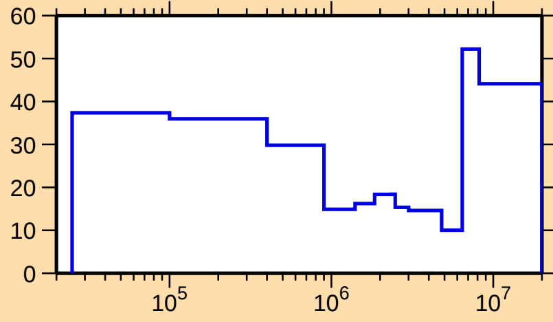
\Delta\sigma/\sigma vs. E for ^{172}\text{Tm}(n,\text{inel.})
