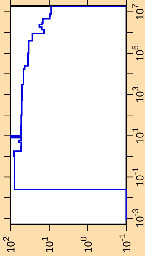
\Delta\sigma/\sigma vs. E for ^{172}\text{Tm}(n,\text{nonel.})
