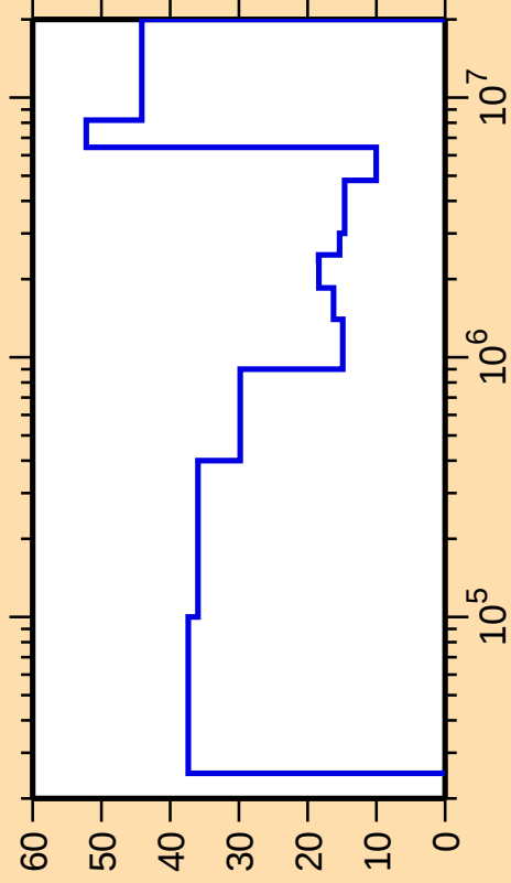
\Delta\sigma/\sigma vs. E for ^{172}\text{Tm}(n,\text{inel.})
