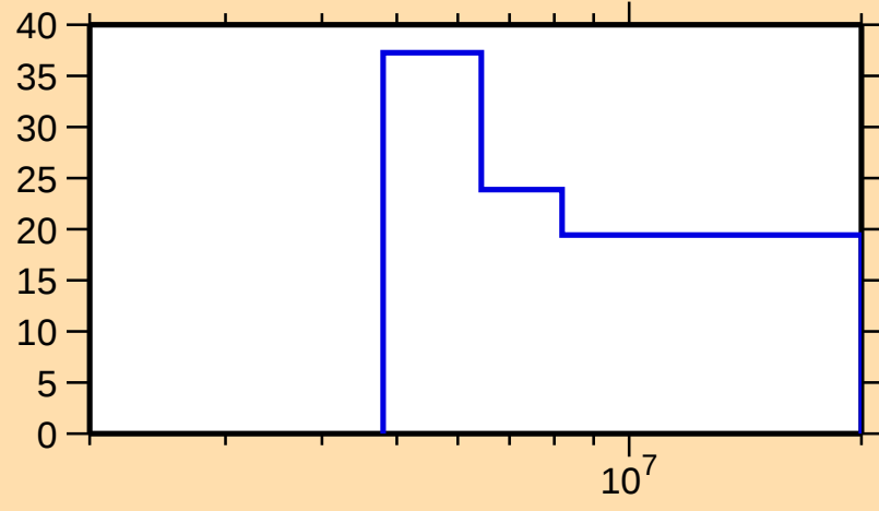
\Delta\sigma/\sigma vs. E for ^{172}\text{Tm}(n,2n)
