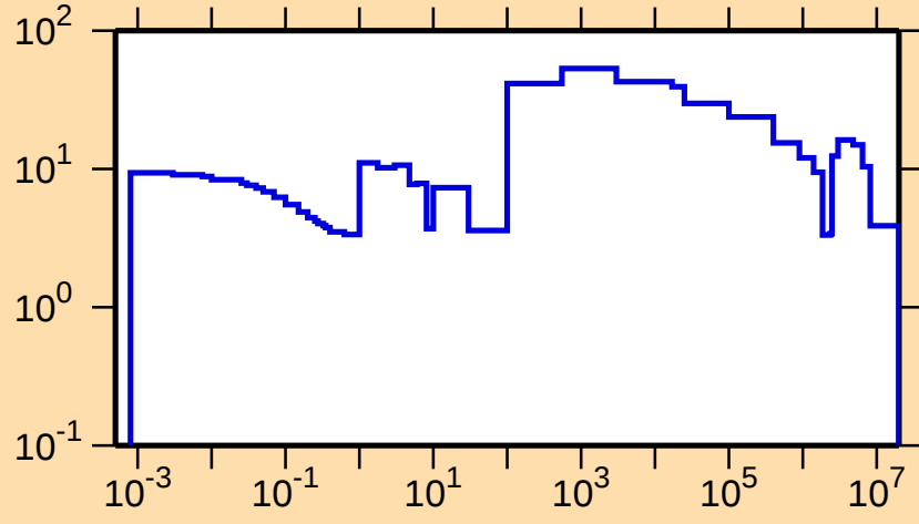
\Delta\sigma/\sigma vs. E for ^{172}\text{Tm}(n,\text{tot.})
