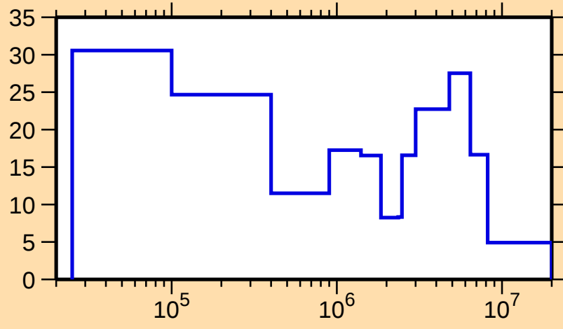
\Delta\sigma/\sigma vs. E for ^{172}\text{Tm}(n,\text{el.})
