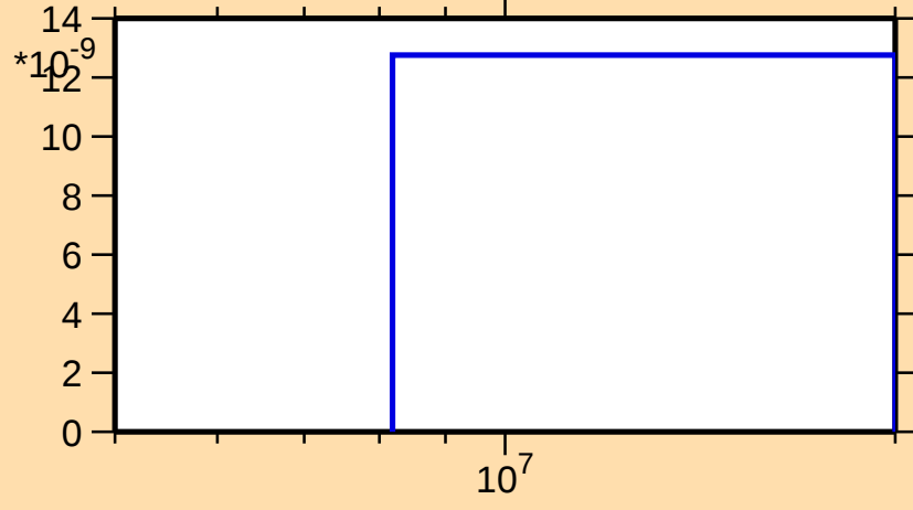
\sigma vs. E for ^{172}\text{Tm}(n,2np)
