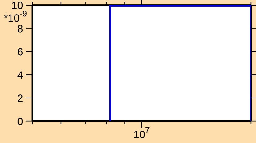
\sigma vs. E for ^{172}\text{Tm}(n,nt)
