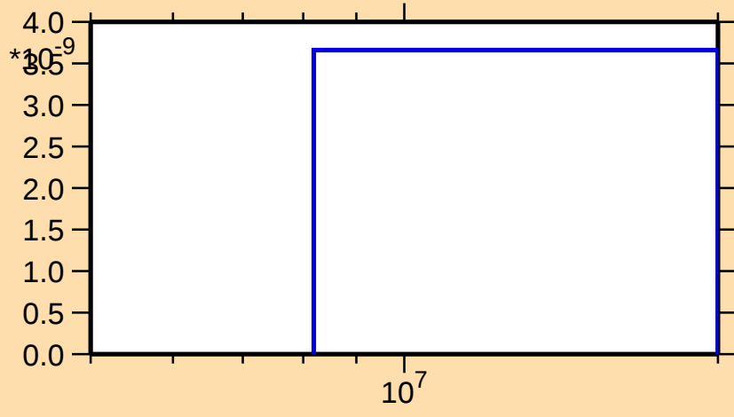
\sigma vs. E for ^{172}\text{Tm}(n,2n\alpha)
