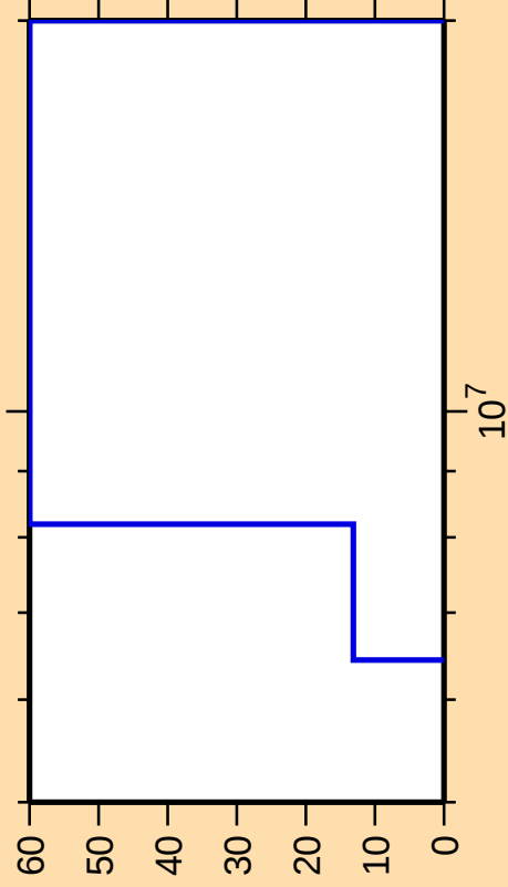
\Delta\sigma/\sigma vs. E for ^{172}\text{Tm}(n,n\alpha)
