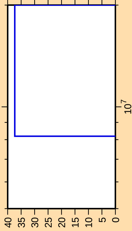
\Delta\sigma/\sigma vs. E for ^{172}\text{Tm}(n,3n)
