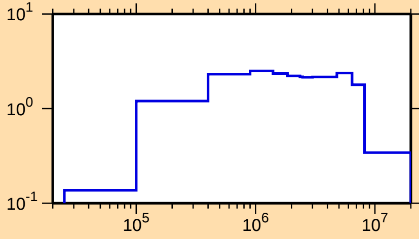
\sigma vs. E for ^{172}\text{Tm}(n,\text{inel.})
