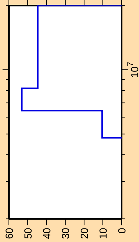
\Delta\sigma/\sigma vs. E for ^{172}\text{Tm}(n,n\text{cont.})
