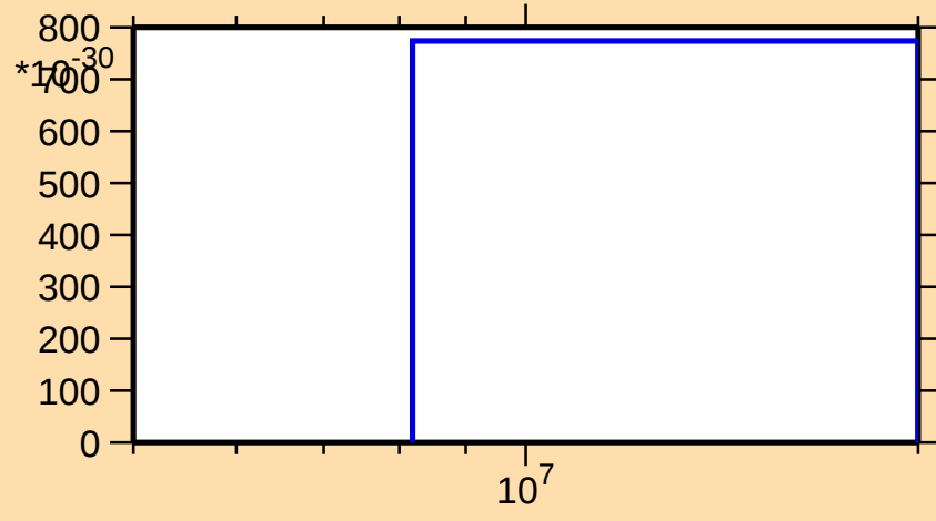
\sigma vs. E for ^{172}\text{Tm} (mt 42)
