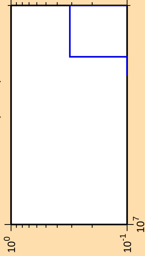
\Delta\sigma/\sigma vs. E for ^{179}\text{Tm}(n,3n\alpha)
