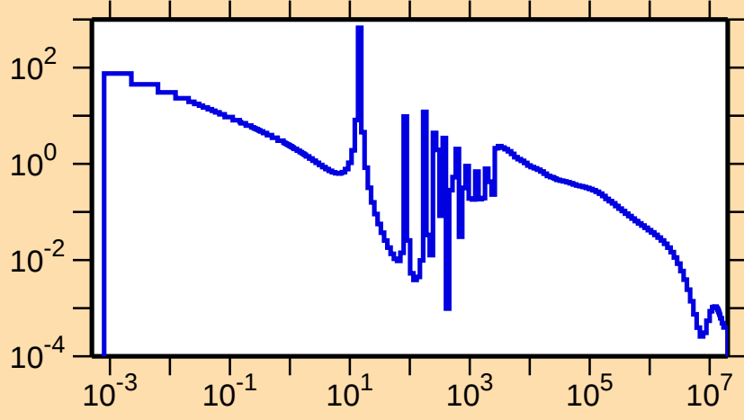
\sigma vs. E for ^{179}\text{Tm}(n,\gamma)
