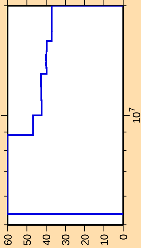
\Delta\sigma/\sigma vs. E for ^{179}\text{Tm}(n,n\text{cont.})
