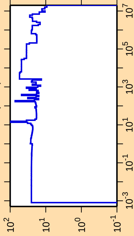
\Delta\sigma/\sigma vs. E for ^{179}\text{Tm}(n,\text{el.})
