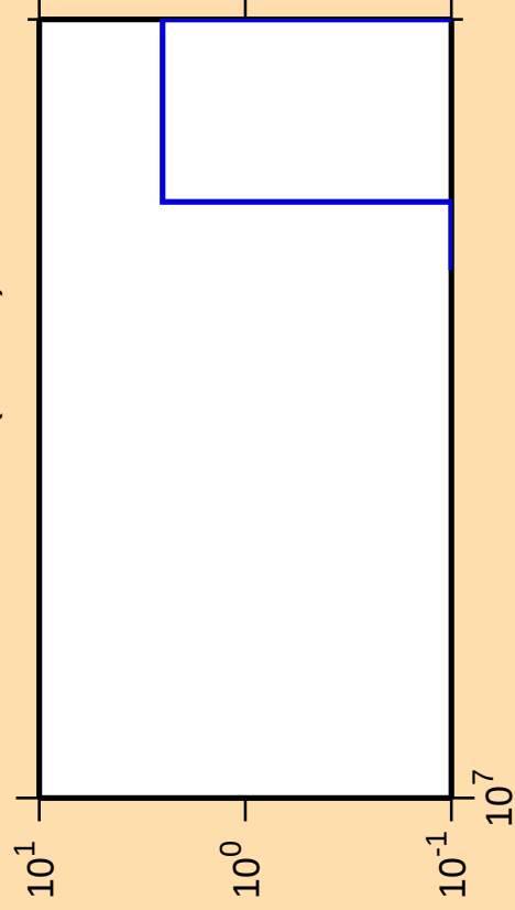
\Delta\sigma/\sigma vs. E for ^{179}\text{Tm}(\text{mt } 11)
