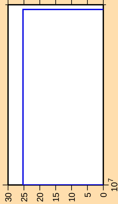
\Delta\sigma/\sigma vs. E for ^{179}\text{Tm}(n,3n)
