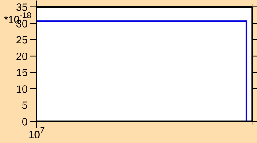
\sigma vs. E for ^{179}\text{Tm} (mt 42)
