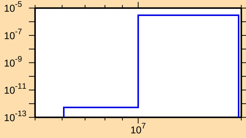
\sigma vs. E for ^{179}\text{Tm}(n,\alpha)
