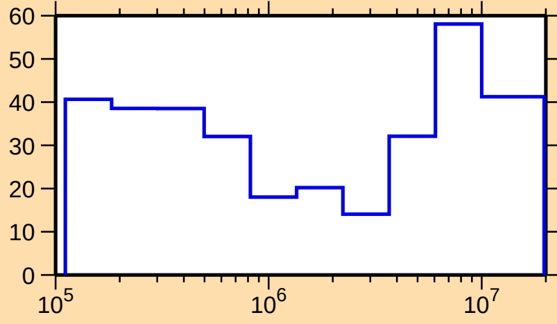
\Delta\sigma/\sigma vs. E for ^{179}\text{Tm}(n,\text{inel.})
