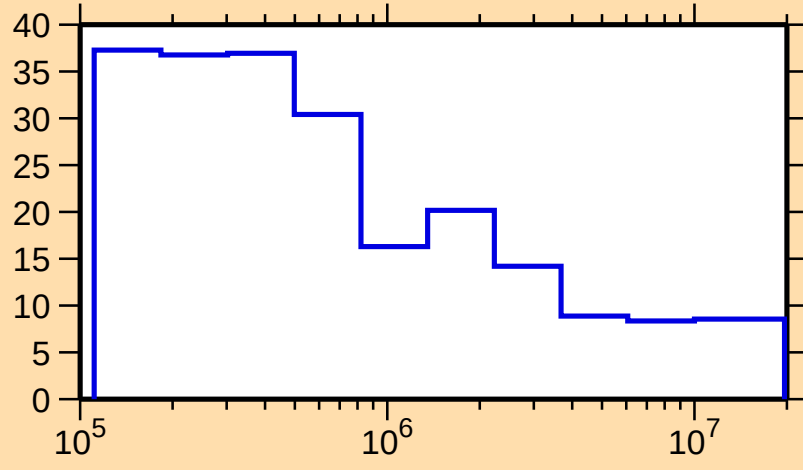
\Delta\sigma/\sigma vs. E for ^{179}\text{Tm}(n,\text{nonel.})
