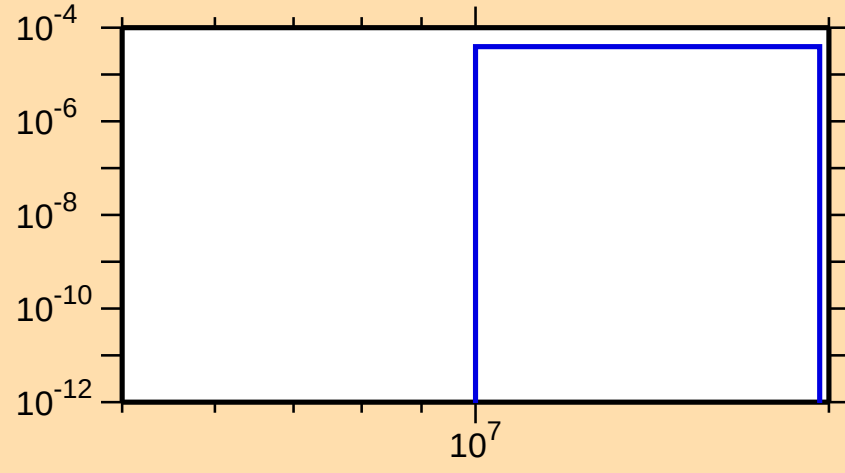
\sigma vs. E for ^{179}\text{Tm}(n,np)
