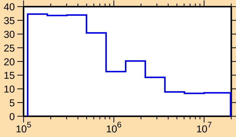
\Delta\sigma/\sigma vs. E for ^{179}\text{Tm}(n,n\text{oncl.})
