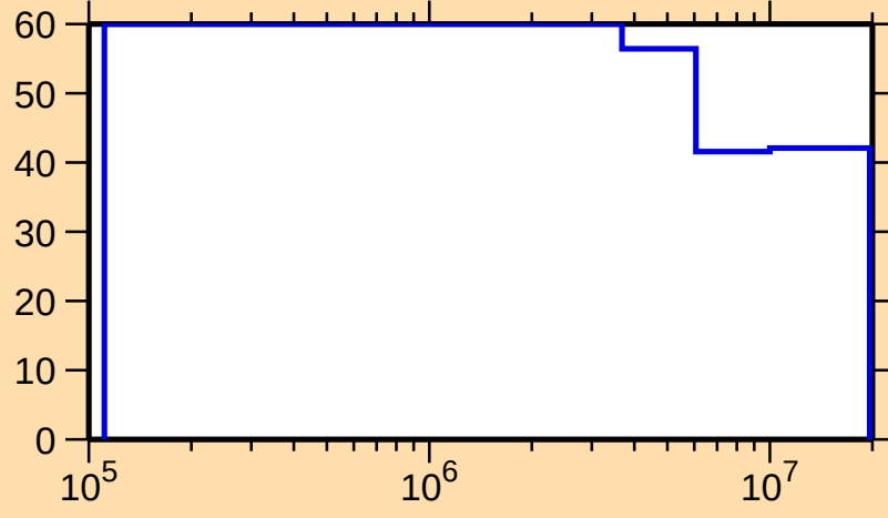
\Delta\sigma/\sigma vs. E for ^{179}\text{Tm}(n,n_1)
