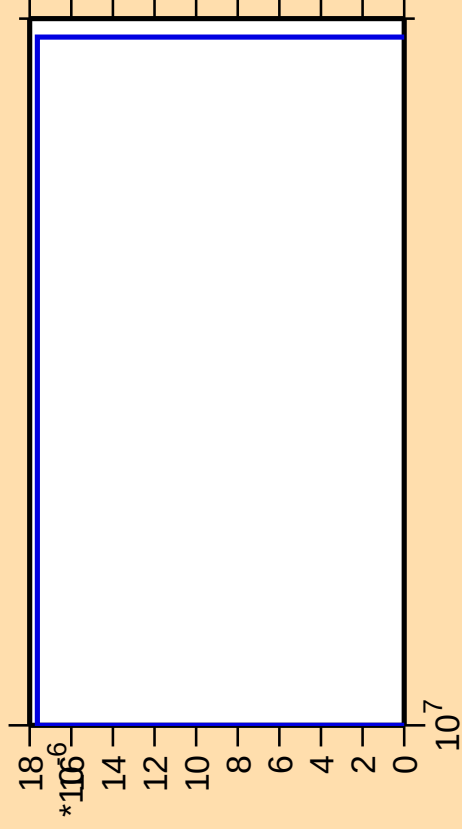
\Delta\sigma/\sigma vs. E for ^{179}\text{Tm} (mt 42)
