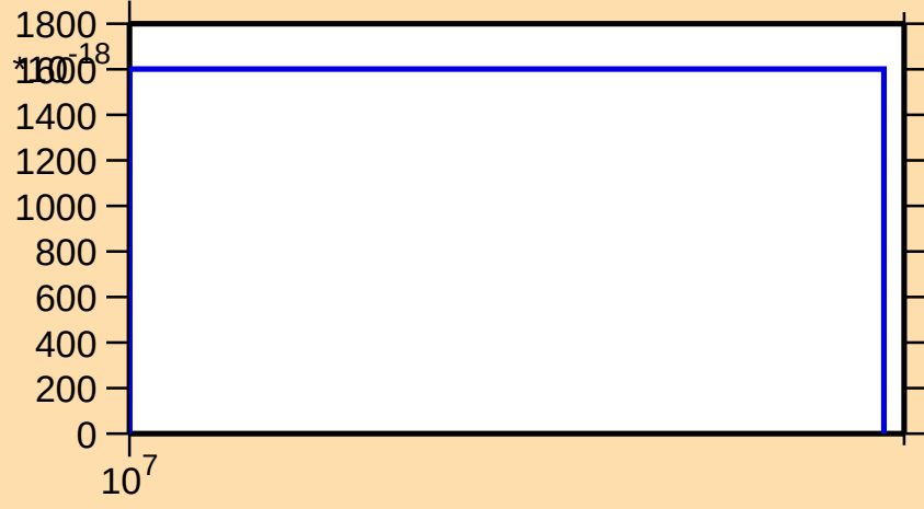
\sigma vs. E for ^{179}\text{Tm}(n,3n\alpha)
