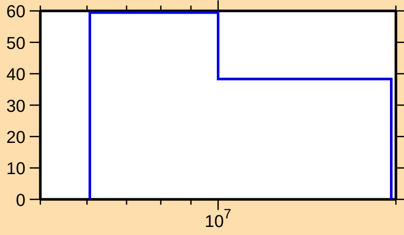
\Delta\sigma/\sigma vs. E for ^{179}\text{Tm}(n,p)
