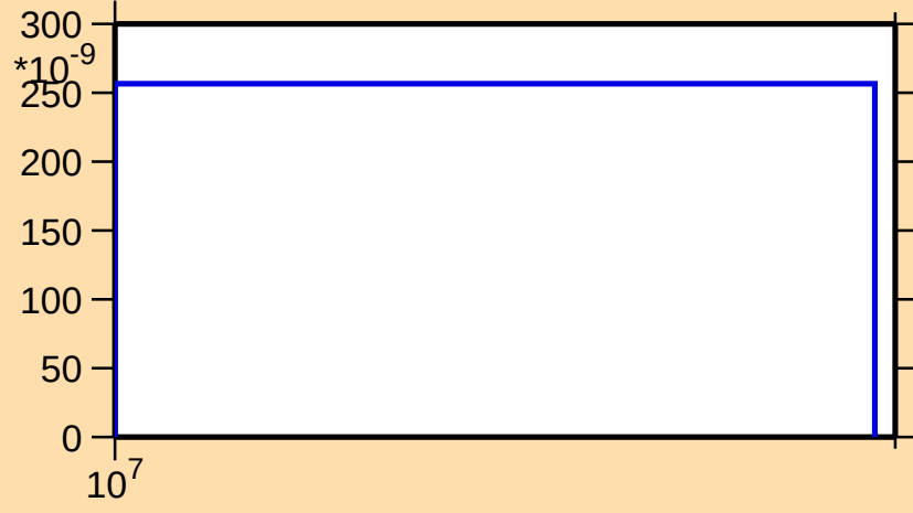
\sigma vs. E for ^{179}\text{Tm}(n,nt)
