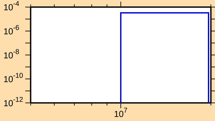
\sigma vs. E for ^{179}\text{Tm}(n,d)
