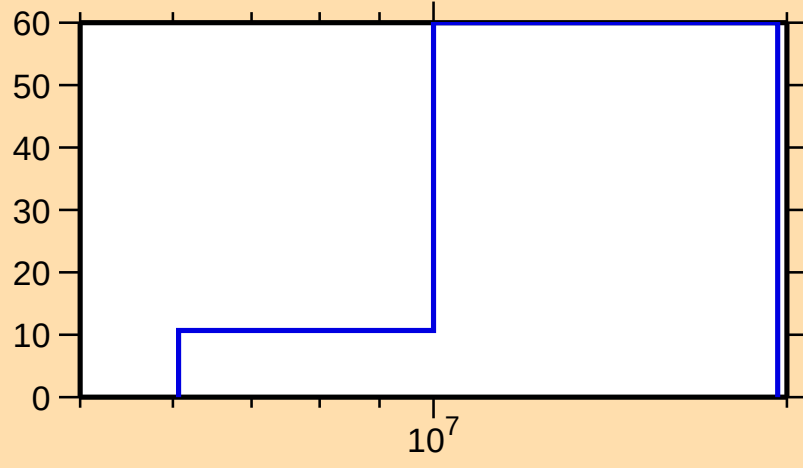
\Delta\sigma/\sigma vs. E for ^{179}\text{Tm}(n,2n)
