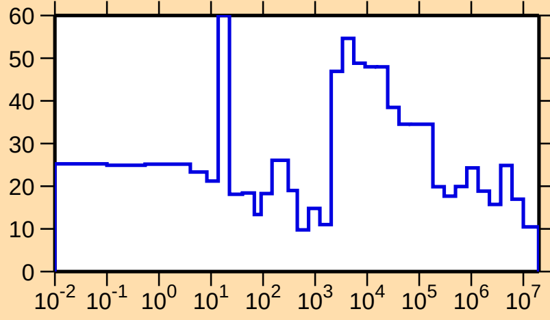
\Delta\sigma/\sigma vs. E for ^{179}\text{Tm}(n,\text{el.})
