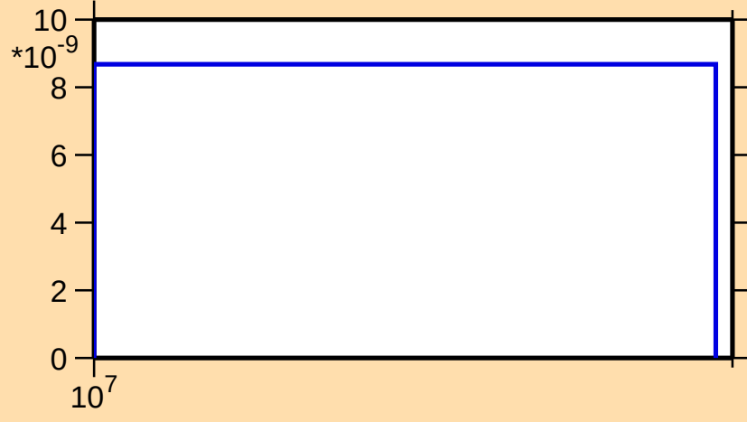
\sigma vs. E for ^{179}\text{Tm}(n,\text{nd})
