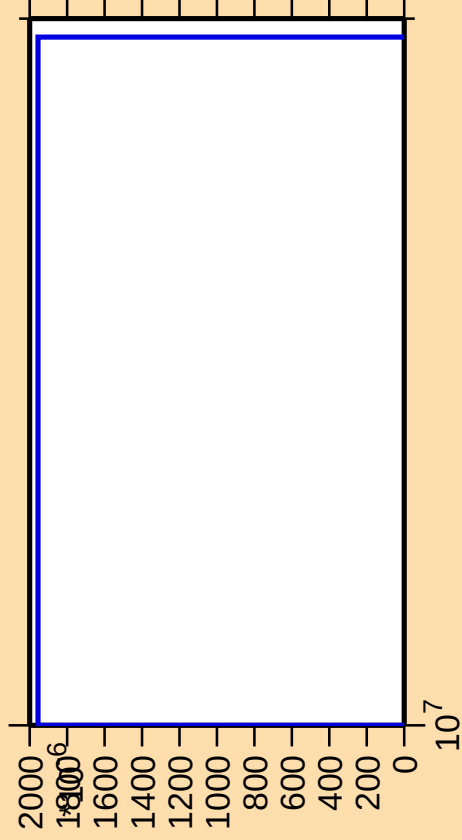
\Delta\sigma/\sigma vs. E for ^{179}\text{Tm}(n,3n\alpha)
