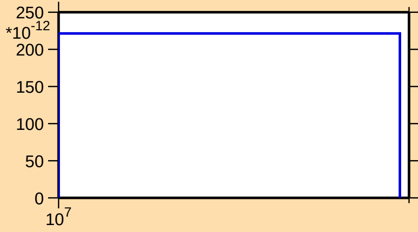
\sigma vs. E for ^{179}\text{Tm}(n,2n\alpha)
