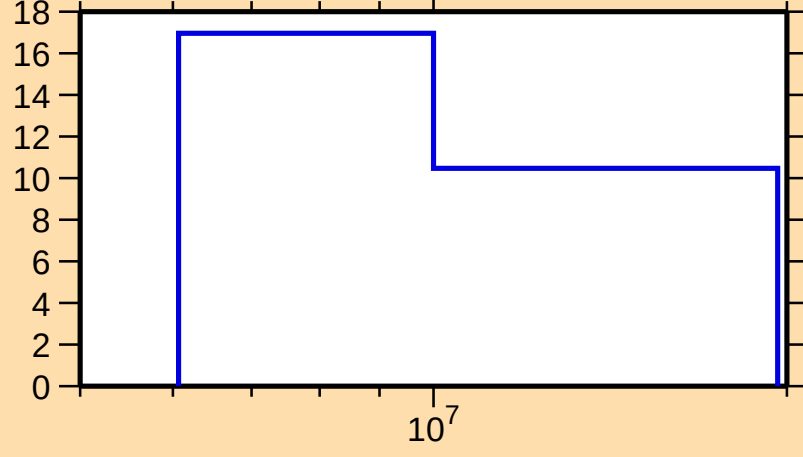
\Delta\sigma/\sigma vs. E for ^{179}\text{Tm}(n,\text{el.})
