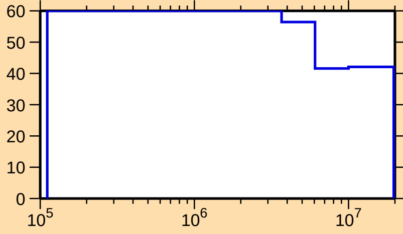
\Delta\sigma/\sigma vs. E for ^{179}\text{Tm}(n,n_1)
