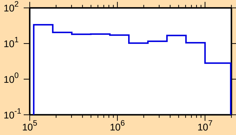
\Delta\sigma/\sigma vs. E for ^{179}\text{Tm}(n,\text{tot.})
