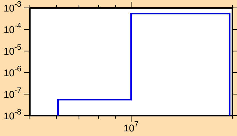
\sigma vs. E for ^{179}\text{Tm}(n,p)
