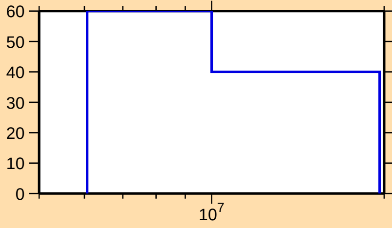
\Delta\sigma/\sigma vs. E for ^{179}\text{Tm}(n,n\text{cont.})
