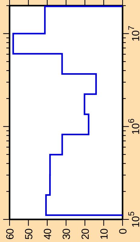
\Delta\sigma/\sigma vs. E for ^{179}\text{Tm}(n,\text{inel.})
