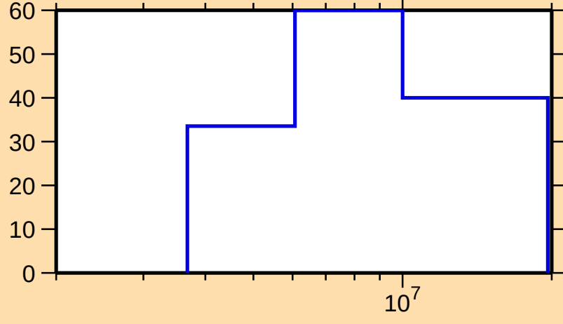
\Delta\sigma/\sigma vs. E for ^{179}\text{Tm}(n,n\text{cont.})
