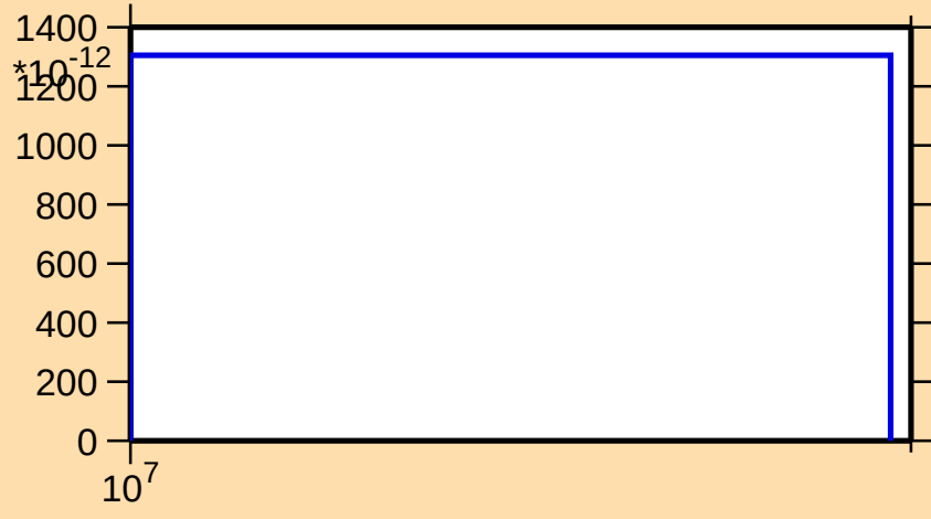
\sigma vs. E for ^{179}\text{Tm}(n,2np)
