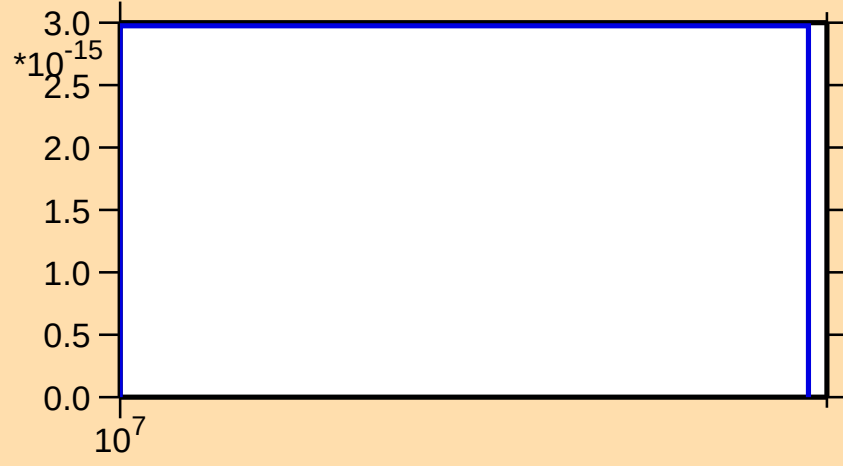
\sigma vs. E for ^{179}\text{Tm}(\text{mt 11})
