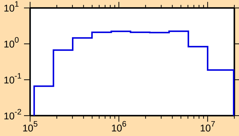
\sigma vs. E for ^{179}\text{Tm}(n,\text{inel.})
