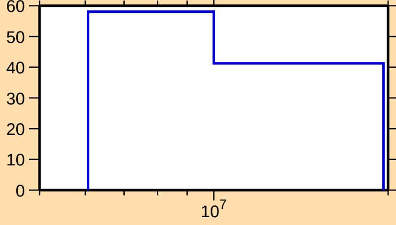
\Delta\sigma/\sigma vs. E for ^{179}\text{Tm}(n,\text{inel.})
