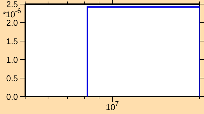
\sigma vs. E for ^{179}\text{Tm}(n,n\alpha)
