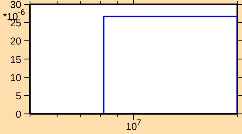
\sigma vs. E for ^{179}\text{Tm}(n,d)
