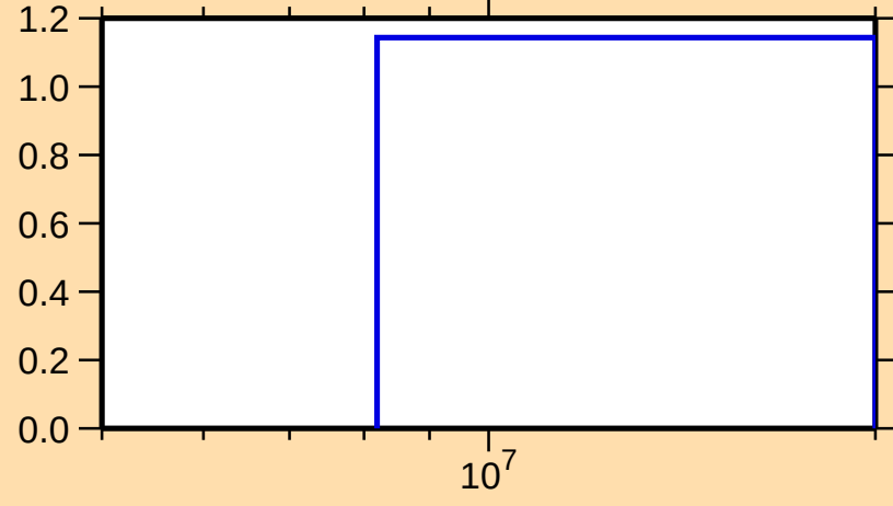
\sigma vs. E for ^{179}\text{Tm}(n,3n)
