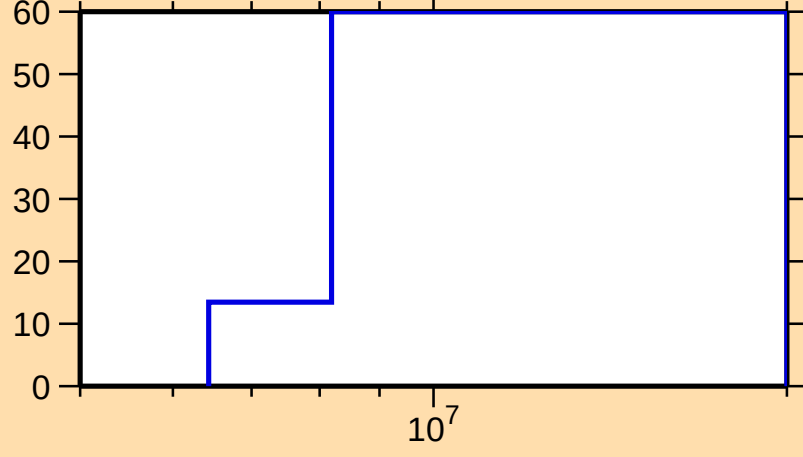
\Delta\sigma/\sigma vs. E for ^{179}\text{Tm}(n,2n)
