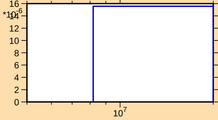
\sigma vs. E for ^{179}\text{Tm}(n,t)
