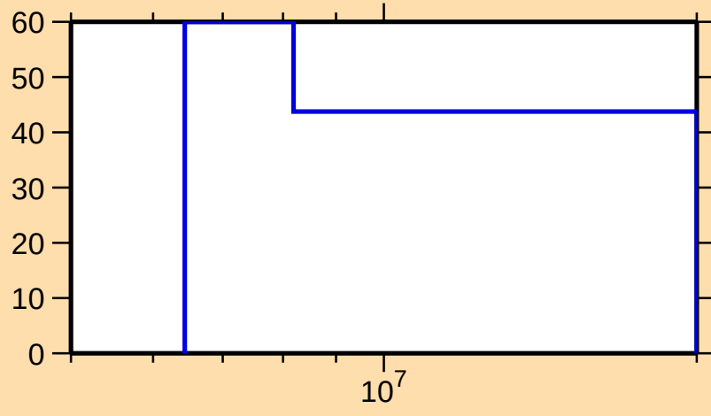
\Delta\sigma/\sigma vs. E for ^{179}\text{Tm}(n,ncont.)
