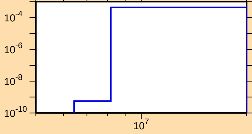
\sigma vs. E for ^{179}\text{Tm}(n,p)
