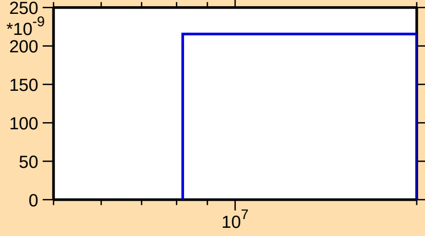
\sigma vs. E for ^{179}\text{Tm}(n,nt)
