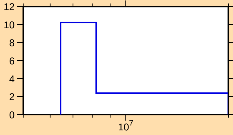
\Delta\sigma/\sigma vs. E for ^{179}\text{Tm}(n,\text{tot.})
