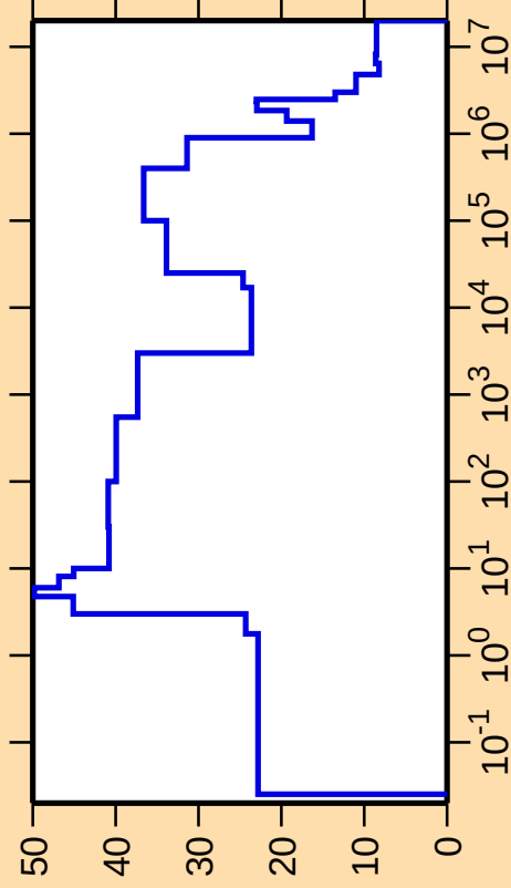
\Delta\sigma/\sigma vs. E for ^{179}\text{Tm}(n,\text{nonel.})
