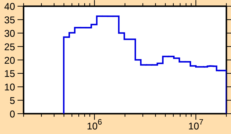
\Delta\sigma/\sigma vs. E for ^{229}\text{U}(\text{n},\text{nonel.})
