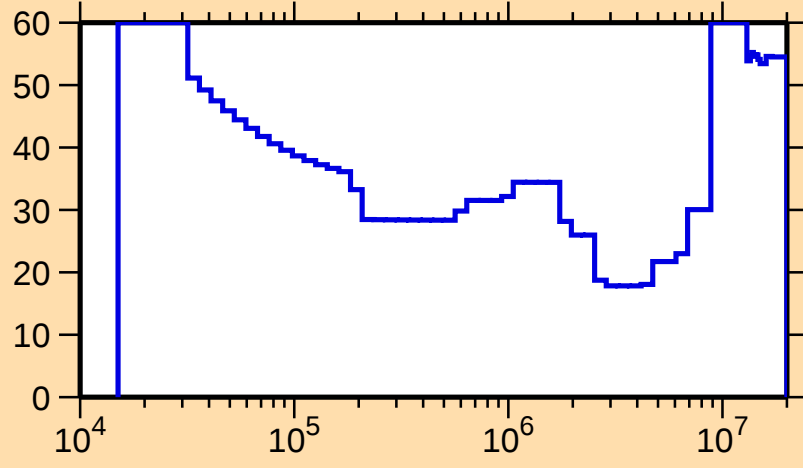
\Delta\sigma/\sigma vs. E for ^{229}\text{U}(n,f)
