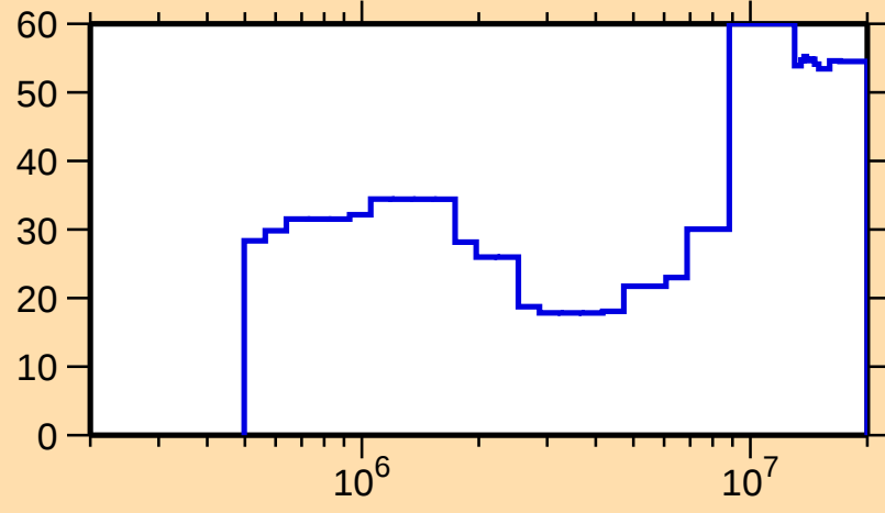
\Delta\sigma/\sigma vs. E for ^{229}\text{U}(\text{n},\text{f})
