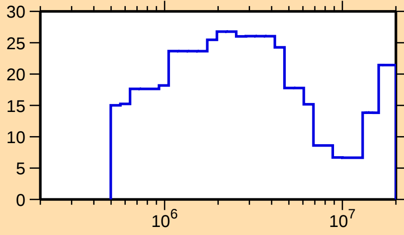
\Delta\sigma/\sigma vs. E for ^{229}\text{U}(\text{n},\text{tot.})
