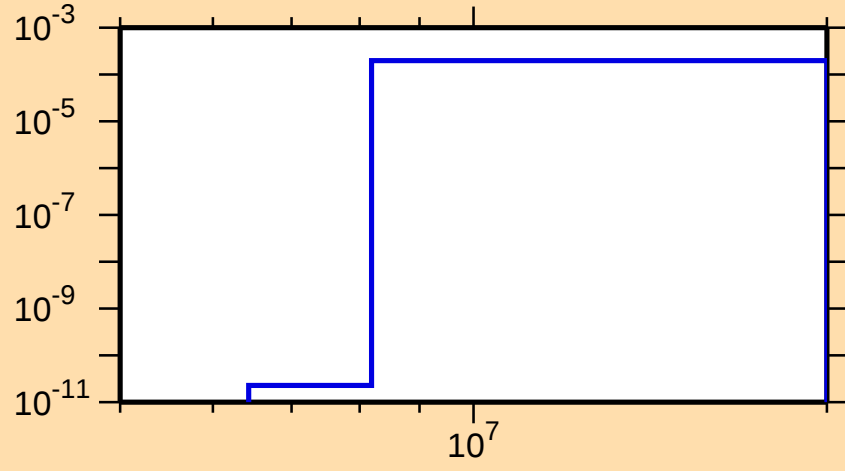
\sigma vs. E for ^{229}\text{U}(n,d)
