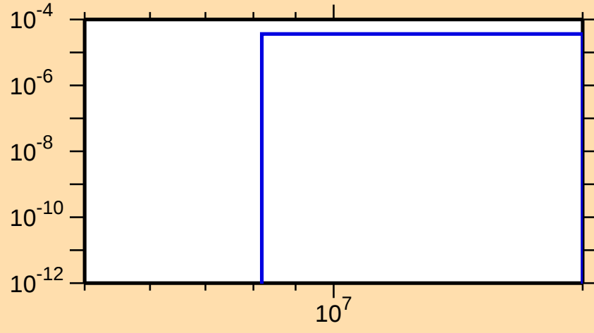
\sigma vs. E for ^{229}\text{U}(n,np)
