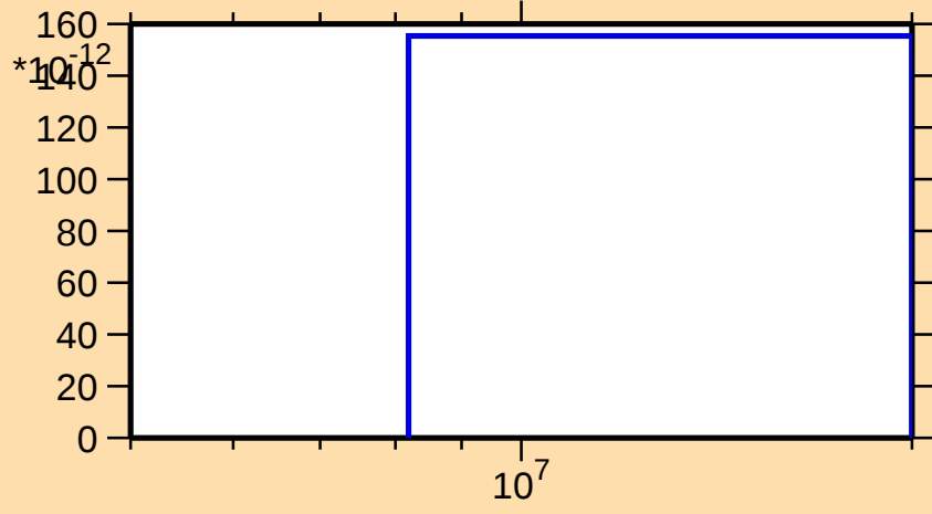
\sigma vs. E for ^{229}\text{U}(\text{n},\text{He3})
