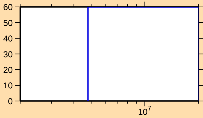
\Delta\sigma/\sigma vs. E for ^{229}\text{U}(\text{n},2\text{n})
