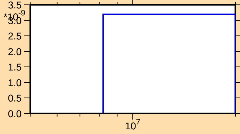
\sigma vs. E for ^{229}\text{U}(\text{n},\text{nt})
