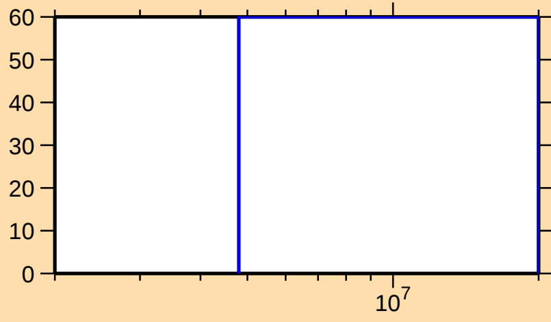
\Delta\sigma/\sigma vs. E for ^{229}\text{U}(n,2n)
