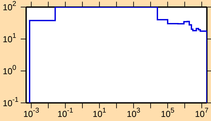
\Delta\sigma/\sigma vs. E for ^{229}\text{U}(\text{n,nonel.})
