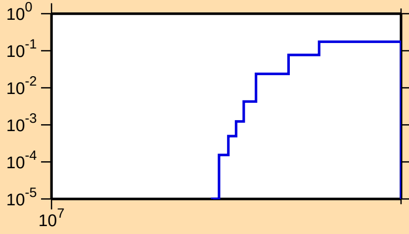
\sigma vs. E for ^{230}\text{U}(n,3n)
