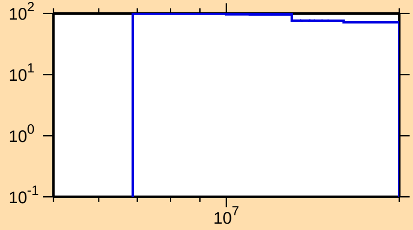
\Delta\sigma/\sigma vs. E for ^{230}\text{U}(n,2n)
