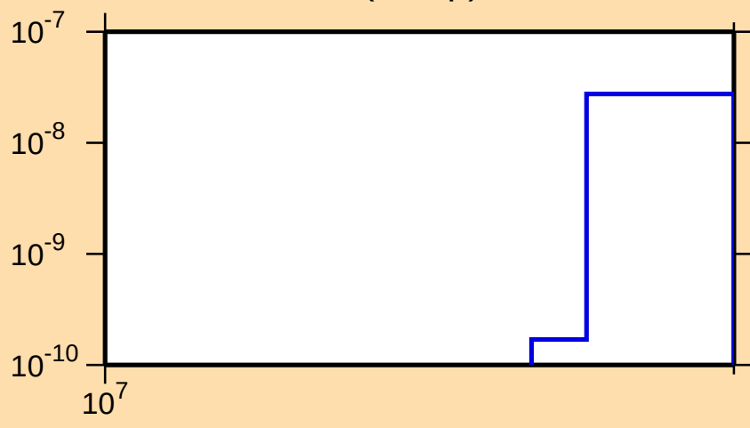
\sigma vs. E for ^{230}\text{U}(n,2np)
