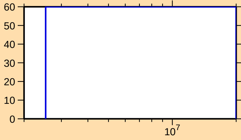
\Delta\sigma/\sigma vs. E for ^{230}\text{U}(n,ncont.)
