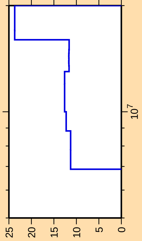
\Delta\sigma/\sigma vs. E for ^{230}\text{U}(n,f)
