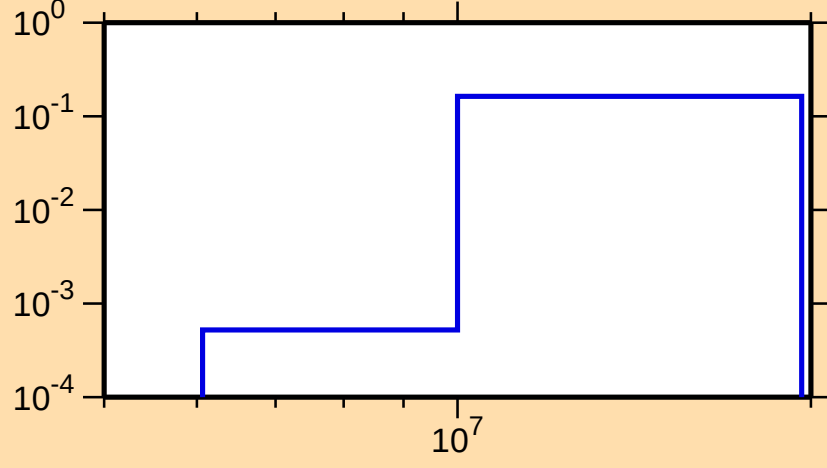
\sigma vs. E for ^{230}\text{U}(n,2n)
