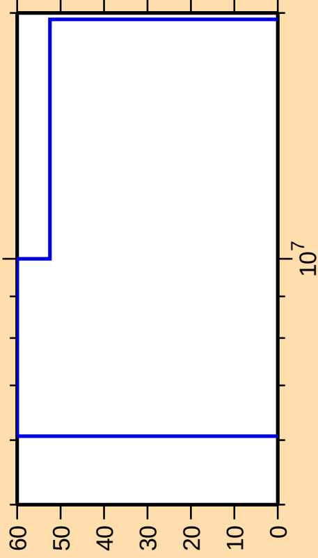
\Delta\sigma/\sigma vs. E for ^{230}\text{U}(n,n_1)
