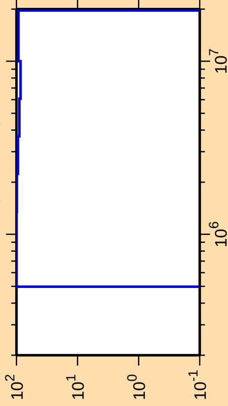
\Delta\sigma/\sigma vs. E for ^{230}\text{U}(\text{n},\text{ncont.})
