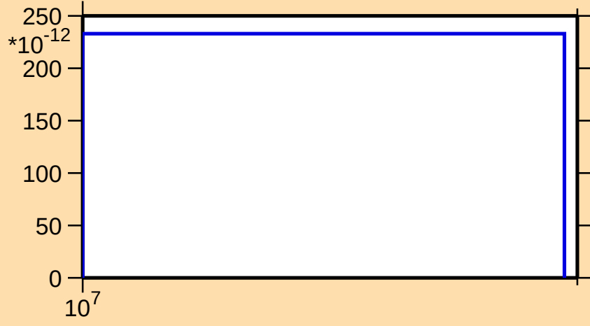
\sigma vs. E for ^{230}\text{U}(n,2np)
