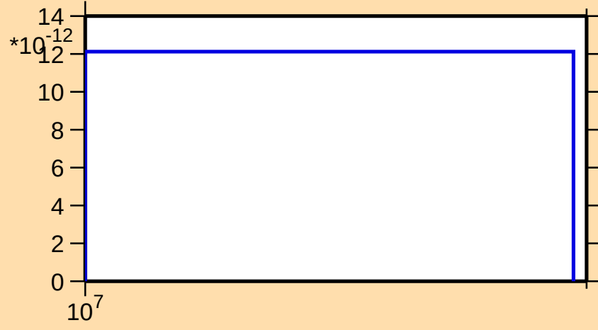
\sigma vs. E for ^{230}\text{U}(n,\text{He}3)
