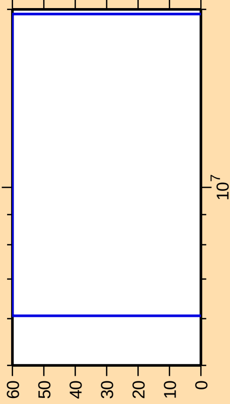
\Delta\sigma/\sigma vs. E for ^{230}\text{U}(n,np)
