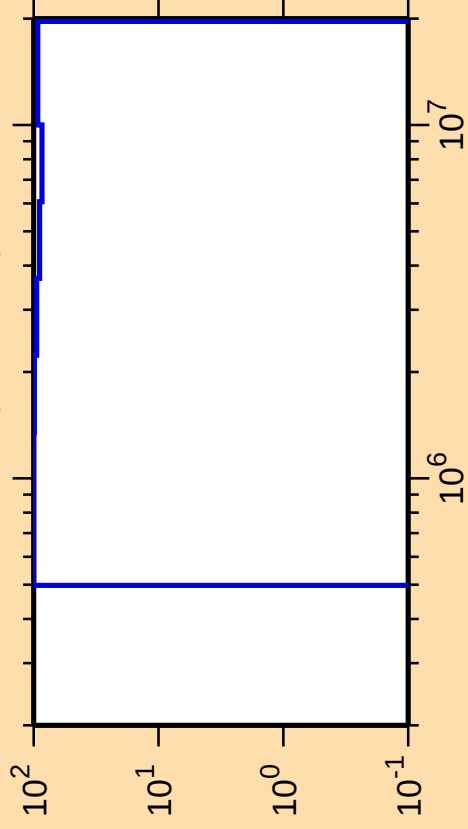
\Delta\sigma/\sigma vs. E for ^{230}\text{U}(\text{n,ncont.})
