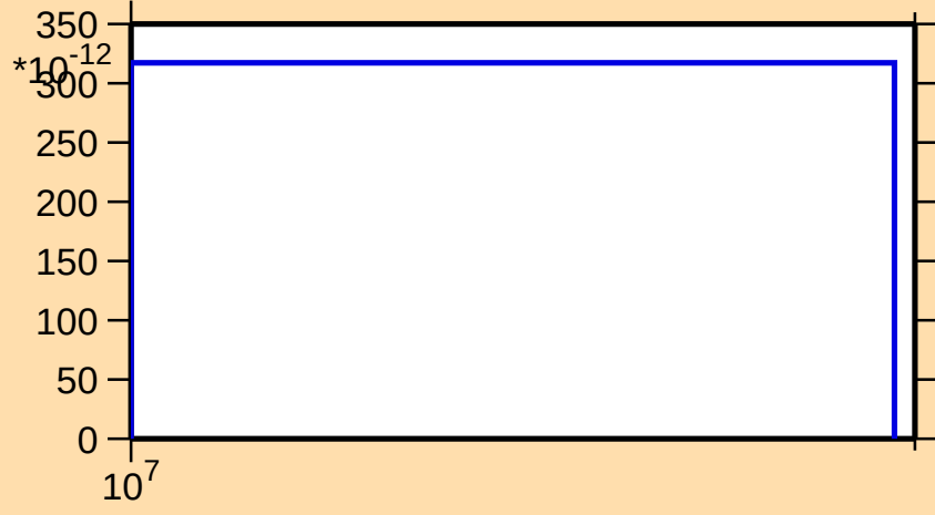
\sigma vs. E for ^{230}\text{U}(\text{n},\text{nd})
