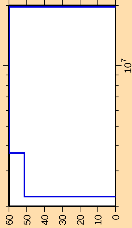
\Delta\sigma/\sigma vs. E for ^{230}\text{U}(\text{n,p})
