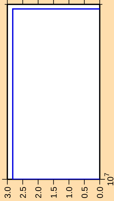
\Delta\sigma/\sigma vs. E for ^{230}\text{U}(n,p\alpha)
