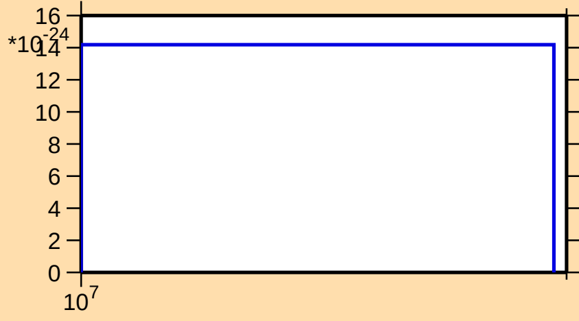
\sigma vs. E for ^{230}\text{U} (mt 42)
