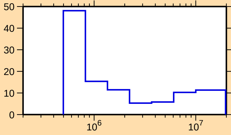
\Delta\sigma/\sigma vs. E for ^{230}\text{U}(\text{n},\text{f})
