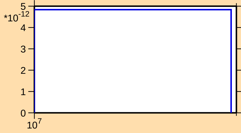
\sigma vs. E for ^{230}\text{U}(n,3n\alpha)
