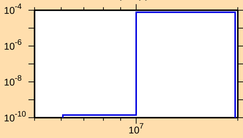
\sigma vs. E for ^{230}\text{U}(n,np)
