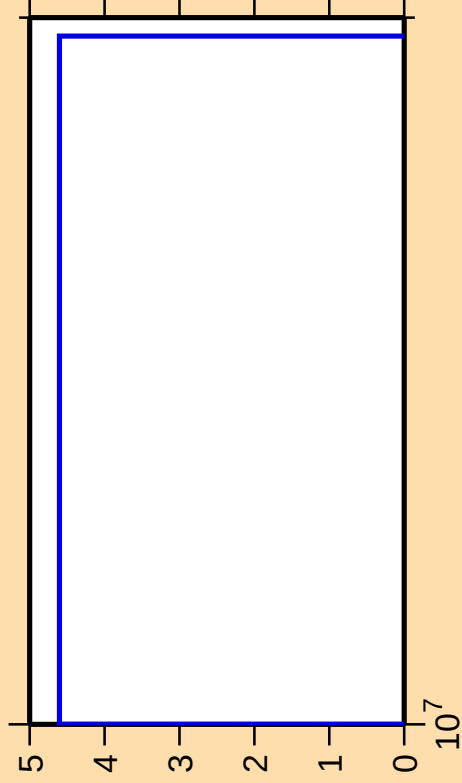
\Delta\sigma/\sigma vs. E for ^{230}\text{U}(\text{n},\text{nt})
