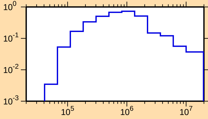
\sigma vs. E for ^{230}\text{U}(\text{n,inel.})
