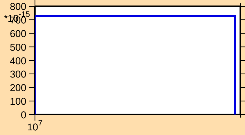
\sigma vs. E for ^{230}\text{U}(n,p\alpha)
