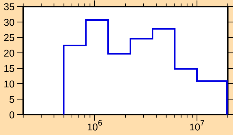
\Delta\sigma/\sigma vs. E for ^{230}\text{U}(\text{n},\text{el.})
