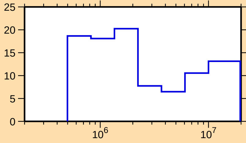
\Delta\sigma/\sigma vs. E for ^{230}\text{U}(\text{n},\text{nonel.})
