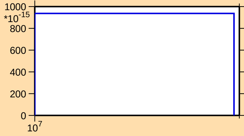
\sigma vs. E for ^{230}\text{U}(\text{n},\text{nt})
