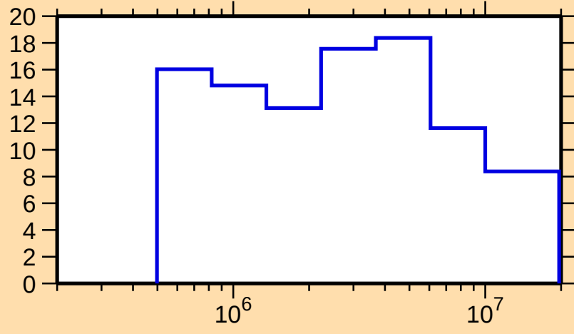
\Delta\sigma/\sigma vs. E for ^{230}\text{U}(\text{n,tot.})
