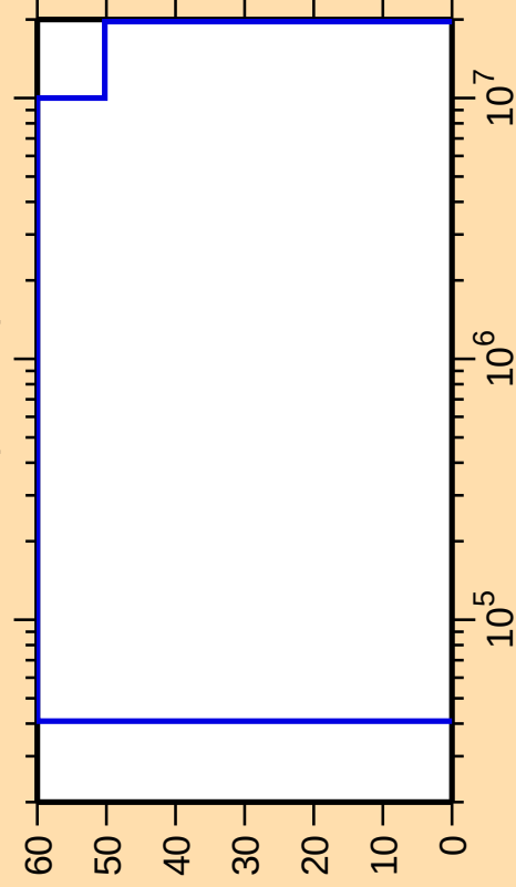
\Delta\sigma/\sigma vs. E for ^{230}\text{U}(\text{n,inel.})
