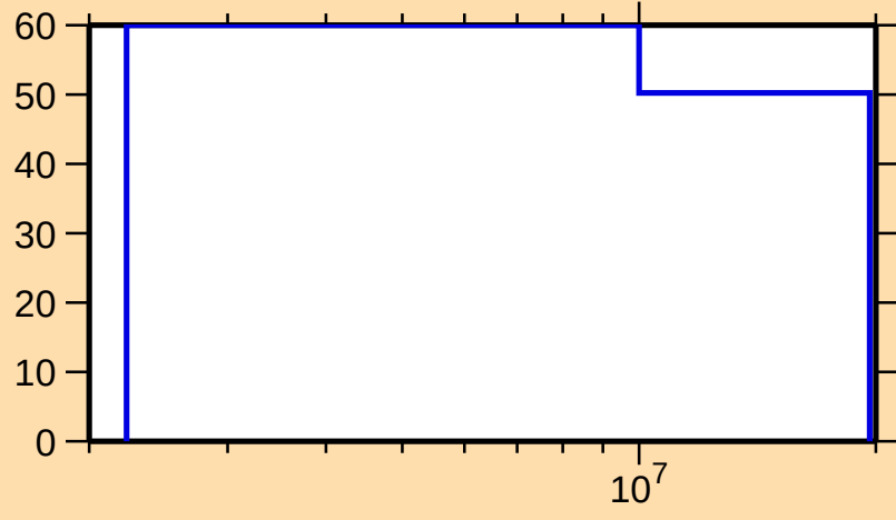
\Delta\sigma/\sigma vs. E for ^{230}\text{U}(\text{n,inel.})
