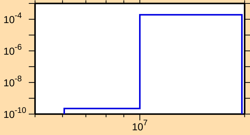
\sigma vs. E for ^{230}\text{U}(n,d)
