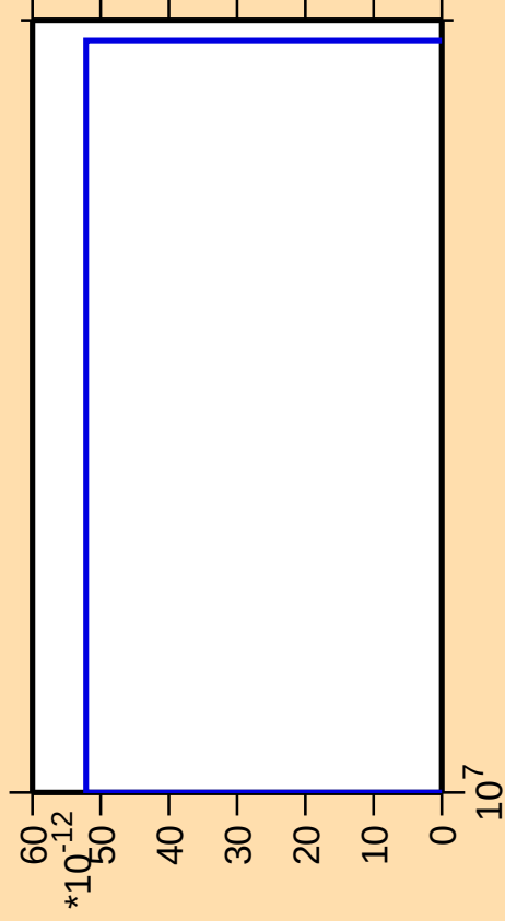
\Delta\sigma/\sigma vs. E for ^{230}\text{U} (mt 42)
