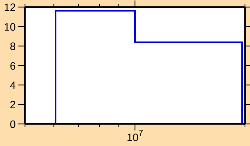
\Delta\sigma/\sigma vs. E for ^{230}\text{U}(n,\text{tot.})
