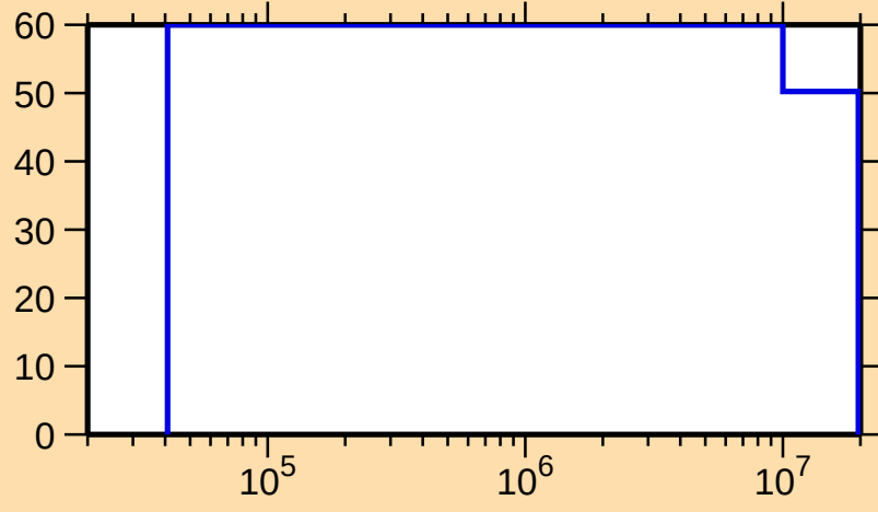
\Delta\sigma/\sigma vs. E for ^{230}\text{U}(n,\text{inel.})
