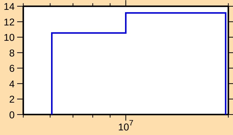
\Delta\sigma/\sigma vs. E for ^{230}\text{U}(n,\text{nonel.})
