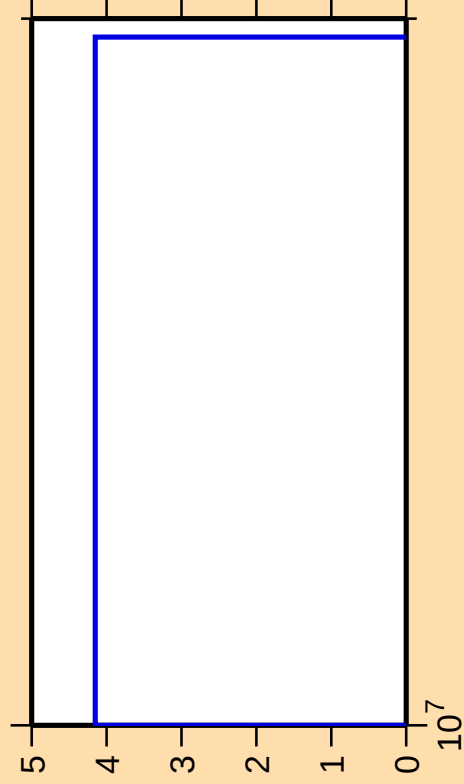
\Delta\sigma/\sigma vs. E for ^{230}\text{U}(n,3n\alpha)
