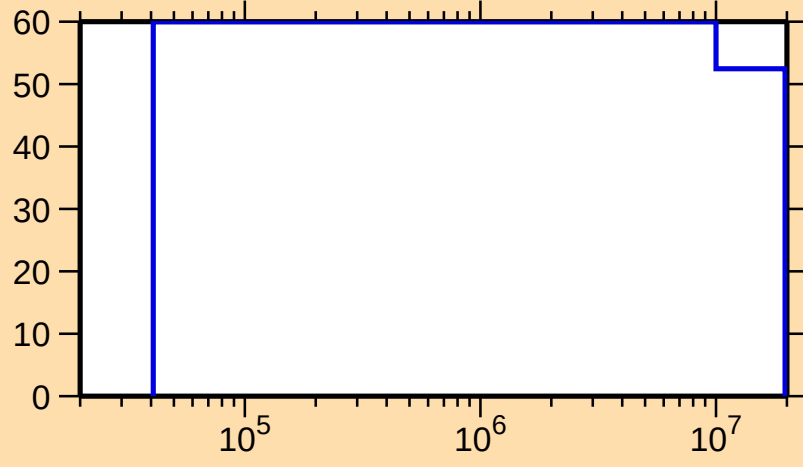
\Delta\sigma/\sigma vs. E for ^{230}\text{U}(n,n_1)
