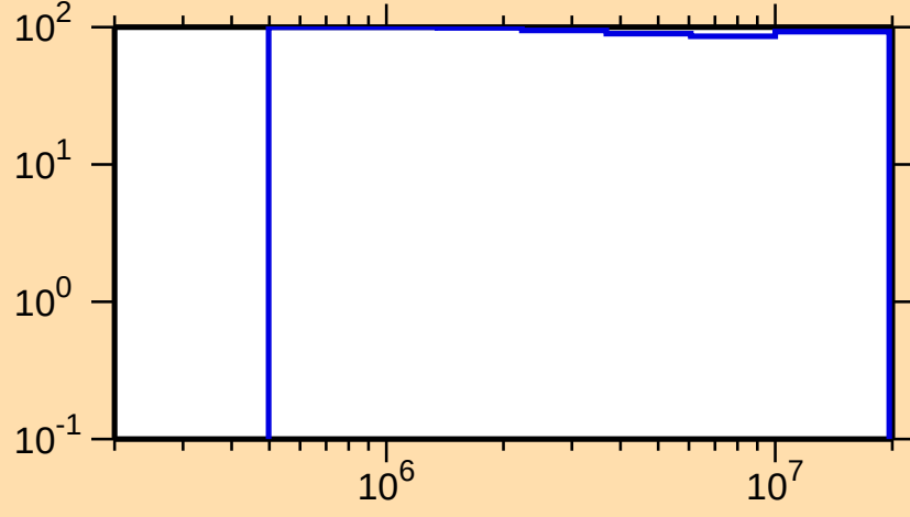
\Delta\sigma/\sigma vs. E for ^{230}\text{U}(n,n\text{cont.})
