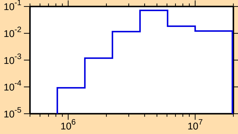
\sigma vs. E for ^{230}\text{U}(n,n\text{cont.})
