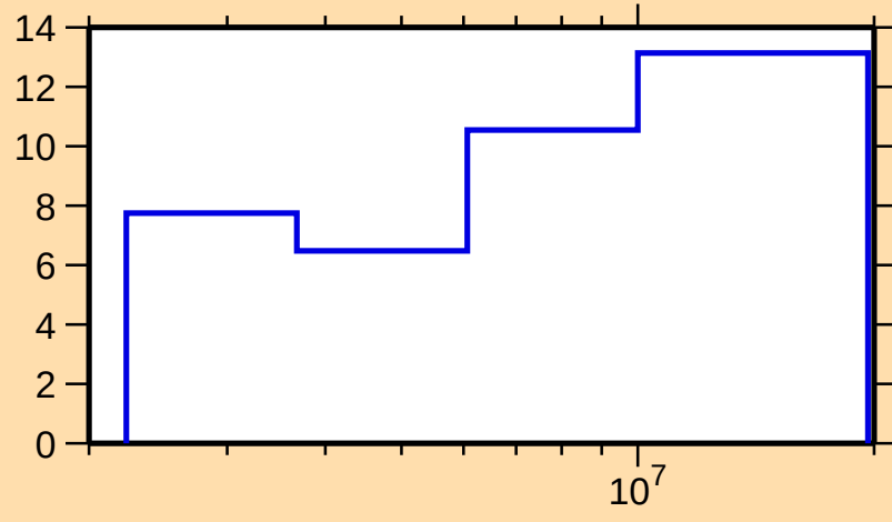
\Delta\sigma/\sigma vs. E for ^{230}\text{U}(\text{n,nonel.})
