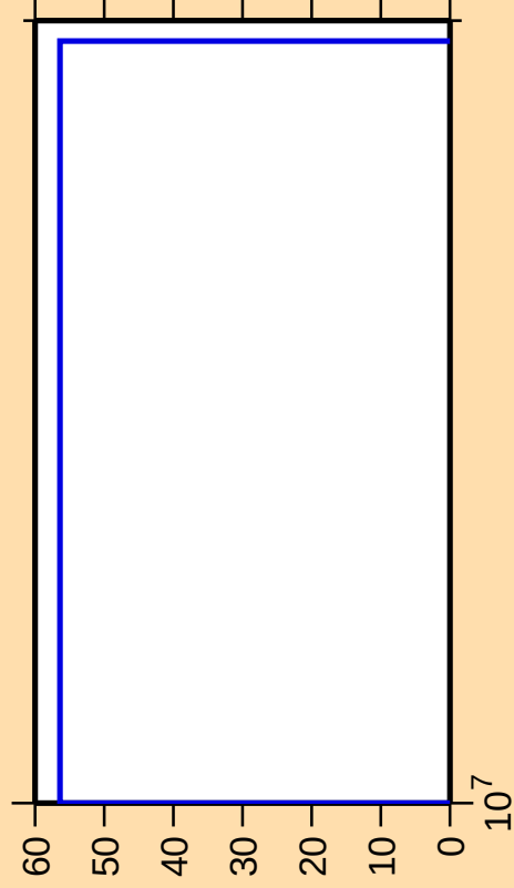
\Delta\sigma/\sigma vs. E for ^{230}\text{U}(n,\text{He}3)
