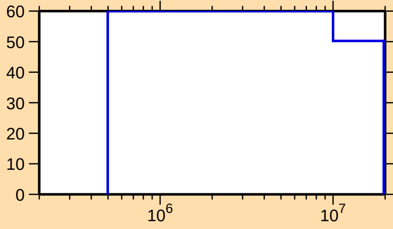
\Delta\sigma/\sigma vs. E for ^{230}\text{U}(\text{n},\text{inel.})
