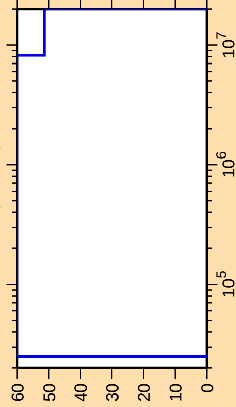
\Delta\sigma/\sigma vs. E for ^{230}\text{U}(n,\text{inel.})
