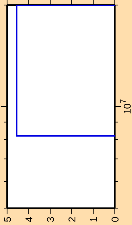
\Delta\sigma/\sigma vs. E for ^{230}\text{U}(n,nt)
