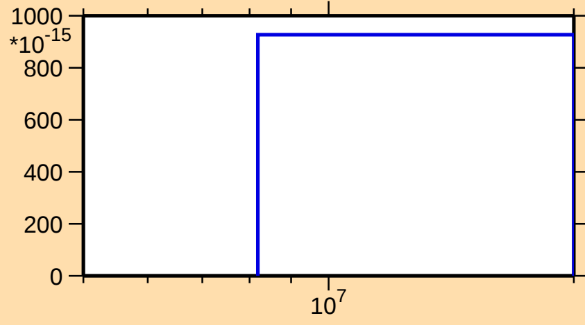
\sigma vs. E for ^{230}\text{U}(n,nt)
