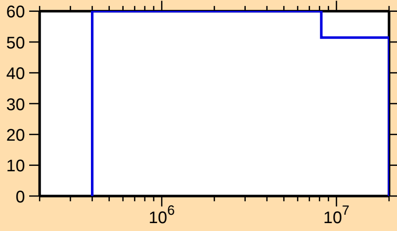
\Delta\sigma/\sigma vs. E for ^{230}\text{U}(\text{n,inel.})
