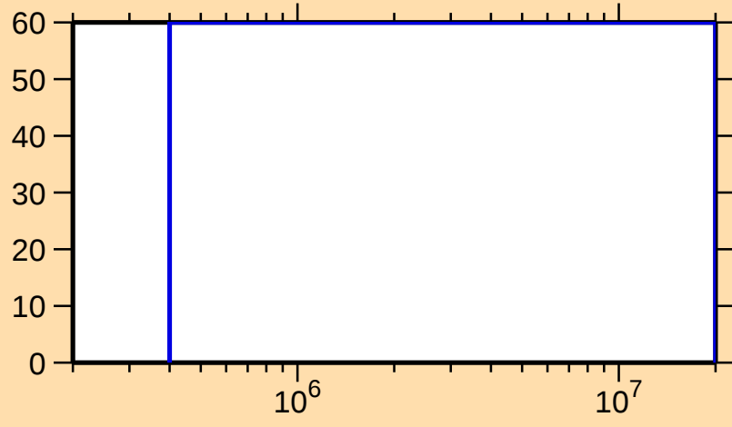
\Delta\sigma/\sigma vs. E for ^{230}\text{U}(n,n\text{cont.})
