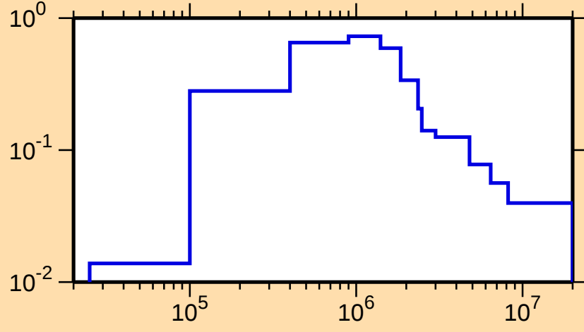
\sigma vs. E for ^{230}\text{U}(n,\text{inel.})
