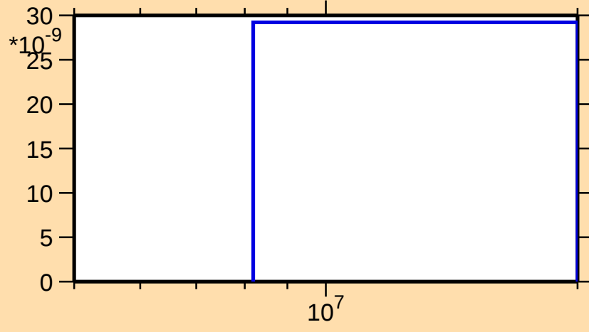
\sigma vs. E for ^{230}\text{U}(n,2n\alpha)
