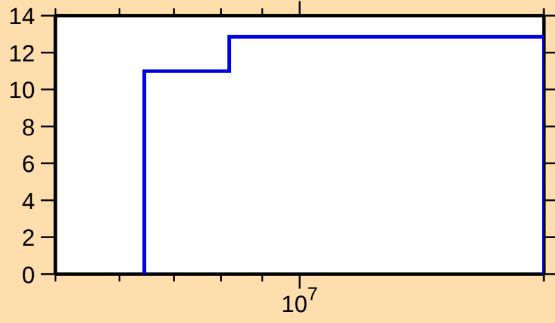
\Delta\sigma/\sigma vs. E for ^{230}\text{U}(n,\text{nonel.})
