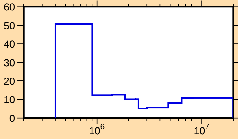
\Delta\sigma/\sigma vs. E for ^{230}\text{U}(n,f)
