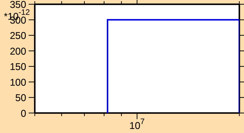
\sigma vs. E for ^{230}\text{U}(n,\text{nd})
