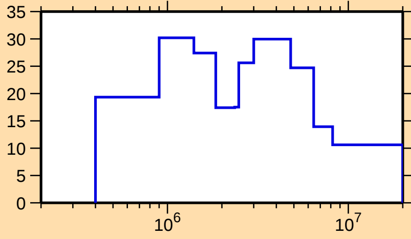
\Delta\sigma/\sigma vs. E for ^{230}\text{U}(\text{n},\text{el.})
