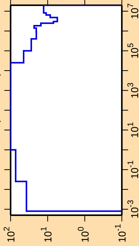
\Delta\sigma/\sigma vs. E for ^{230}\text{U}(\text{n,nonel.})
