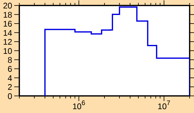
\Delta\sigma/\sigma vs. E for ^{230}\text{U}(\text{n},\text{tot.})
