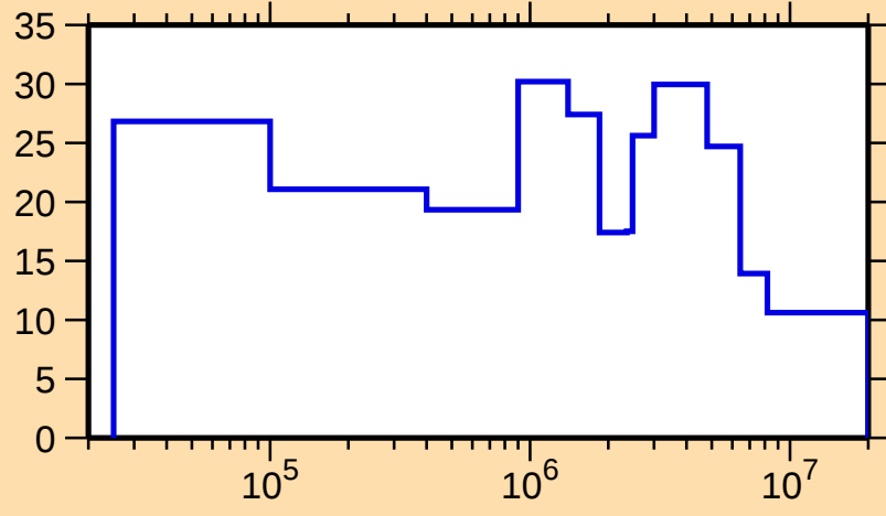
\Delta\sigma/\sigma vs. E for ^{230}\text{U}(n,\text{el.})
