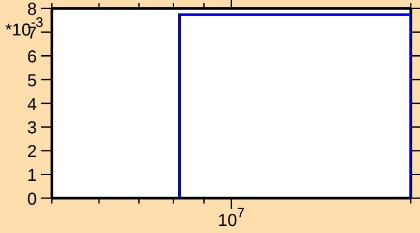
\sigma vs. E for ^{230}\text{U}(n,3n)
