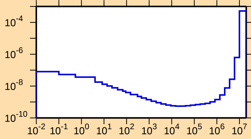
\sigma vs. E for ^{233}\text{U}(n,\alpha)
