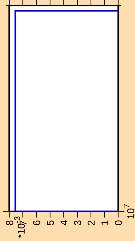
\Delta\sigma/\sigma vs. E for ^{233}\text{U}(\text{n},\text{He3})
