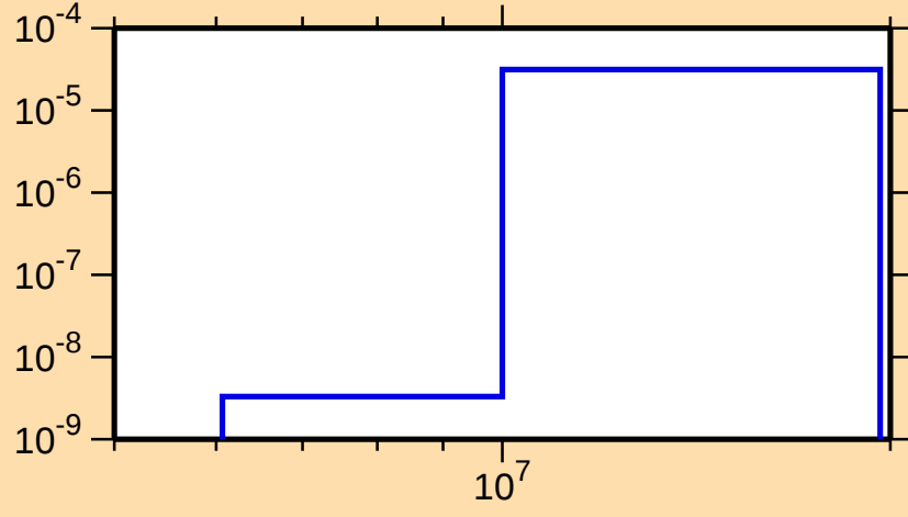
\sigma vs. E for ^{233}\text{U}(n,n\alpha)
