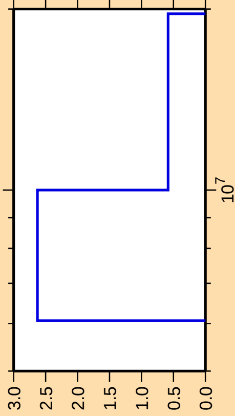
\Delta\sigma/\sigma vs. E for ^{233}\text{U}(n,n\alpha)
