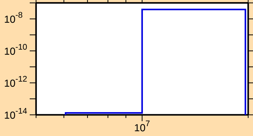
\sigma vs. E for ^{233}\text{U}(n,2n\alpha)
