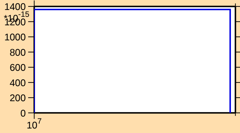
\sigma vs. E for ^{233}\text{U}(\text{n},\text{He3})
