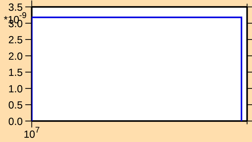
\sigma vs. E for ^{233}\text{U}(\text{n},2\text{np})
