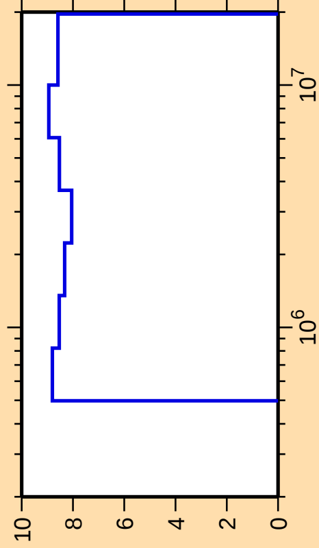
\Delta\sigma/\sigma vs. E for ^{233}\text{U}(\text{n,ncont.})
