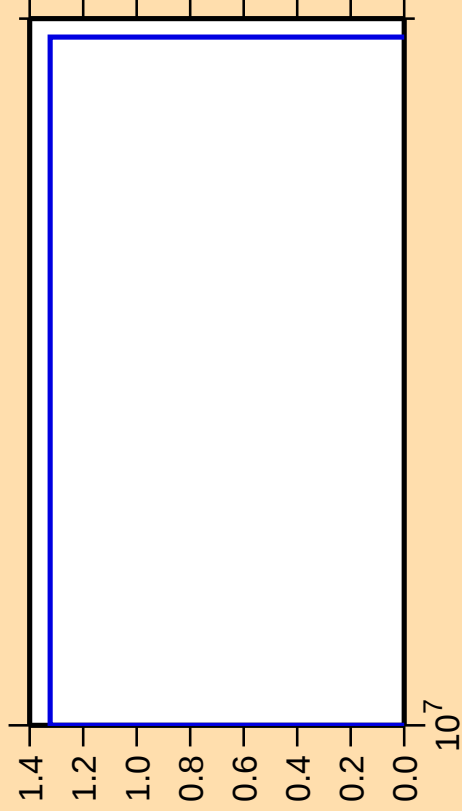
\Delta\sigma/\sigma vs. E for ^{233}\text{U}(\text{n},2\text{np})
