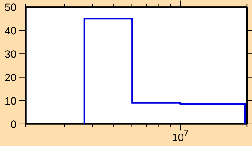
\Delta\sigma/\sigma vs. E for ^{233}\text{U}(\text{n,2n})
