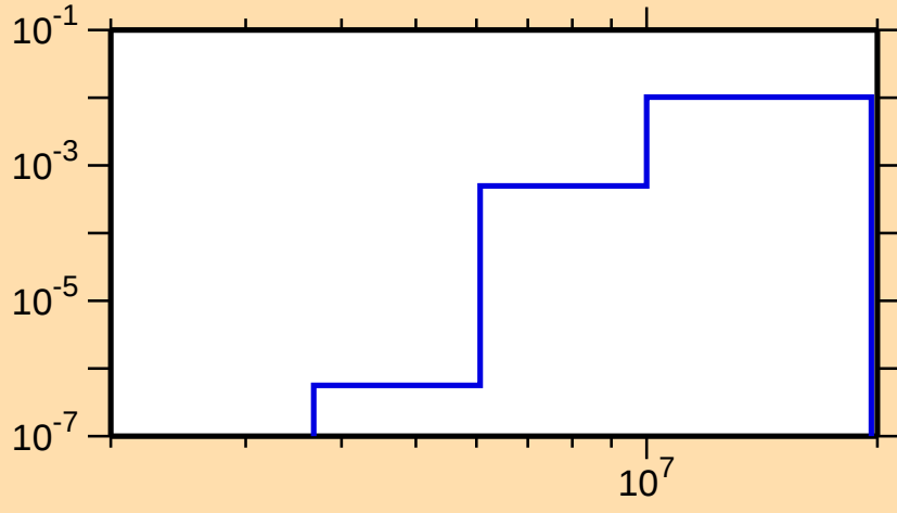
\sigma vs. E for ^{53}\text{V}(n,p)
