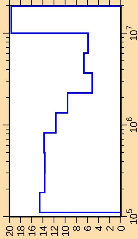
\Delta\sigma/\sigma vs. E for ^{53}\text{V}(\text{n,inel.})
