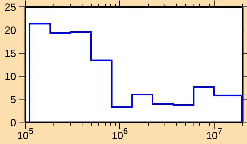
\Delta\sigma/\sigma vs. E for ^{53}\text{V}(\text{n,tot.})
