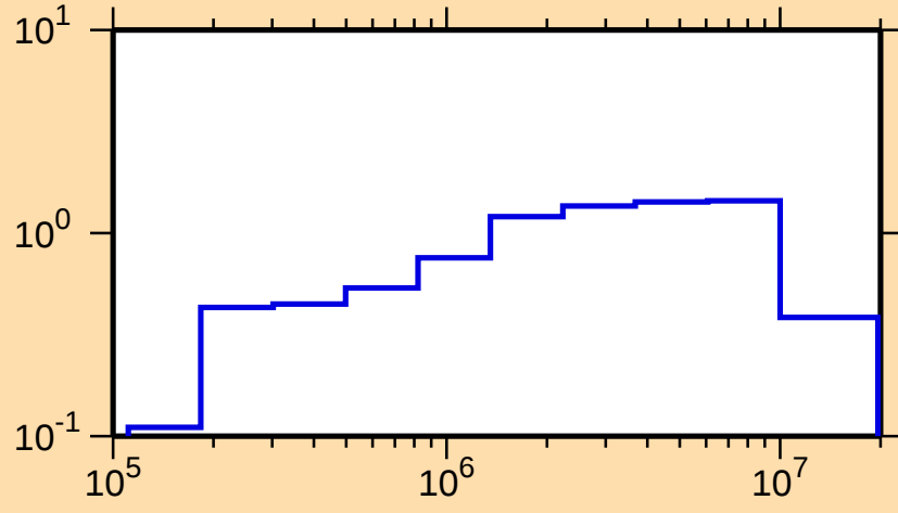
\sigma vs. E for ^{53}\text{V}(\text{n,inel.})
