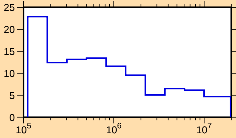
\Delta\sigma/\sigma vs. E for ^{53}\text{V}(\text{n,nonel.})
