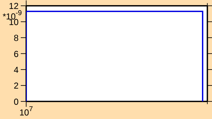
\sigma vs. E for ^{53}\text{V}(\text{n},\text{nt})
