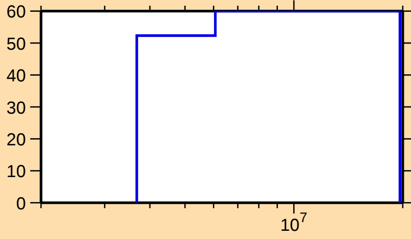
\Delta\sigma/\sigma vs. E for ^{53}\text{V}(n,p)
