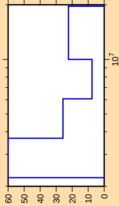
\Delta\sigma/\sigma vs. E for ^{53}\text{V}(\text{n,ncont.})
