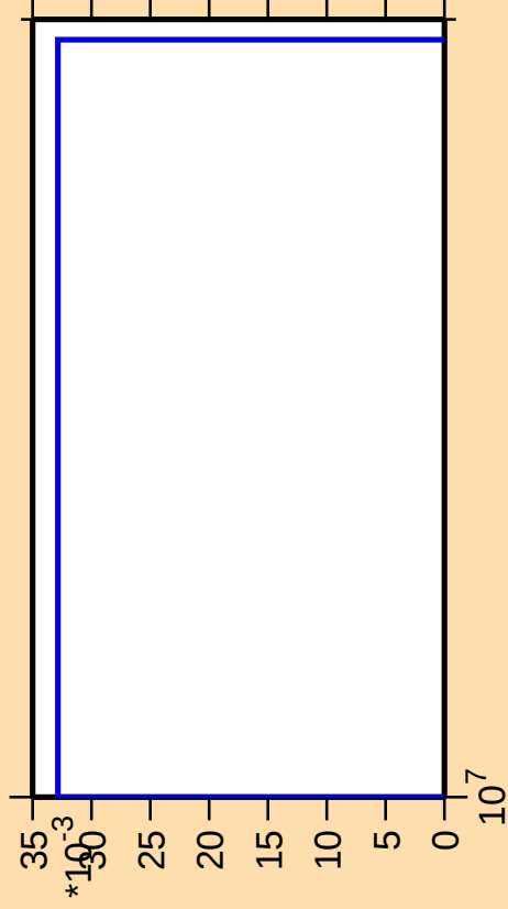
\Delta\sigma/\sigma vs. E for ^{53}\text{V}(\text{n},\text{He3})
