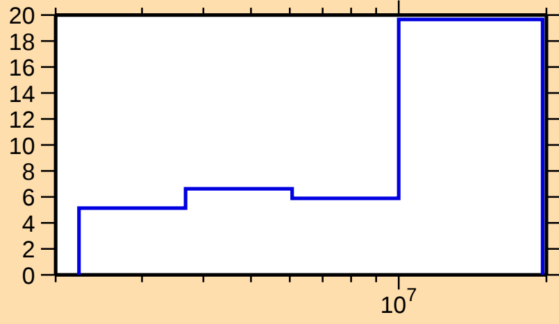
\Delta\sigma/\sigma vs. E for ^{53}\text{V}(\text{n,inel.})
