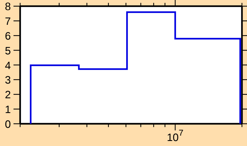
\Delta\sigma/\sigma vs. E for ^{53}\text{V}(\text{n,tot.})
