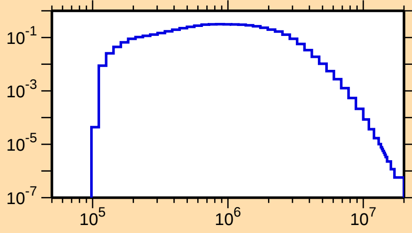
\sigma vs. E for ^{54}\text{V}(n,n_1)
