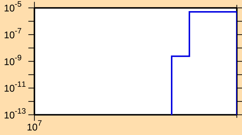
\sigma vs. E for ^{54}\text{V}(\text{n},\text{nt})
