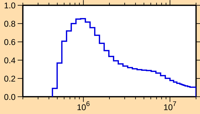
\sigma vs. E for ^{162}\text{W}(n,n_1)
