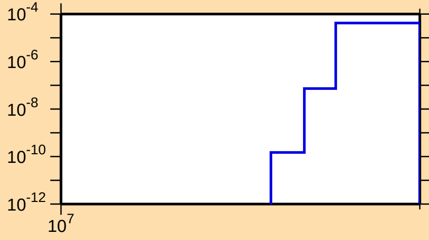
\sigma vs. E for ^{162}\text{W}(n,2np)
