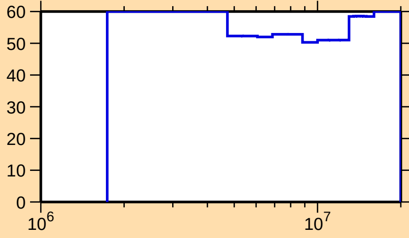
\Delta\sigma/\sigma vs. E for ^{162}\text{W}(n,n\text{cont.})
