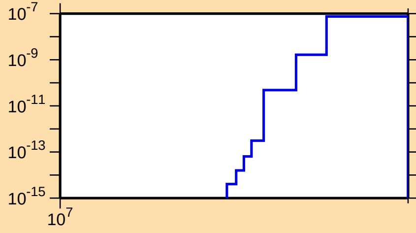
\sigma vs. E for ^{162}\text{W}(n,\text{nd})
