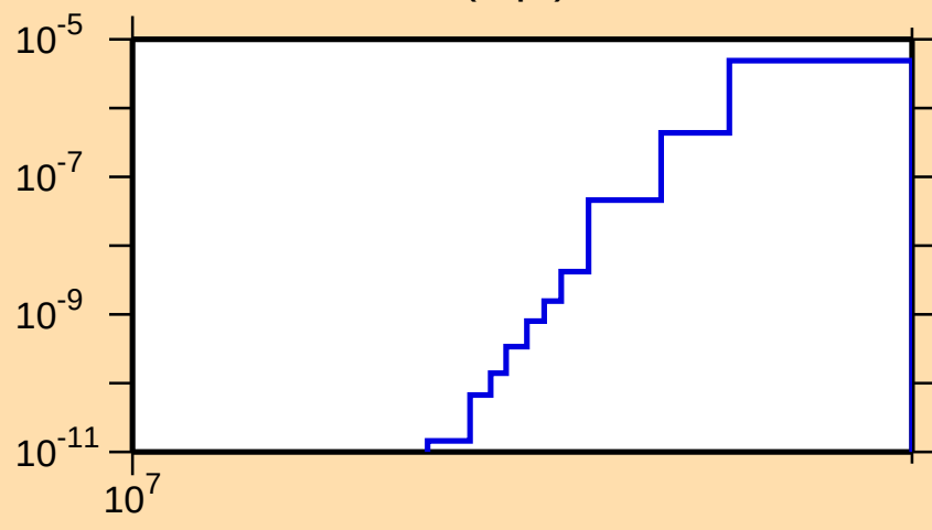
\sigma vs. E for ^{162}\text{W}(n,\text{pt})
