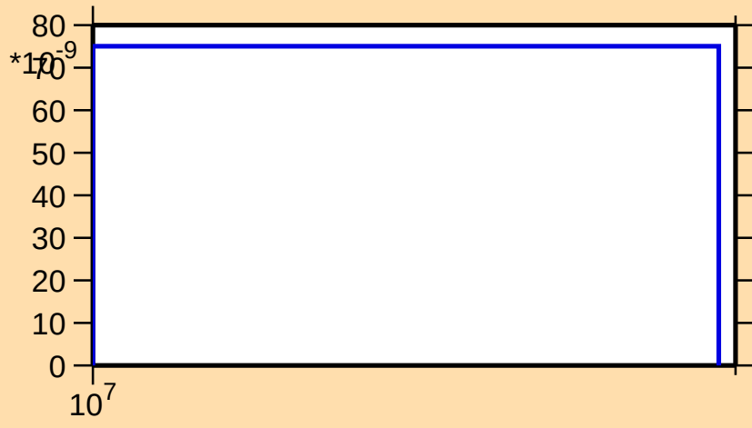
\sigma vs. E for ^{162}\text{W}(\text{n},\text{pt})
