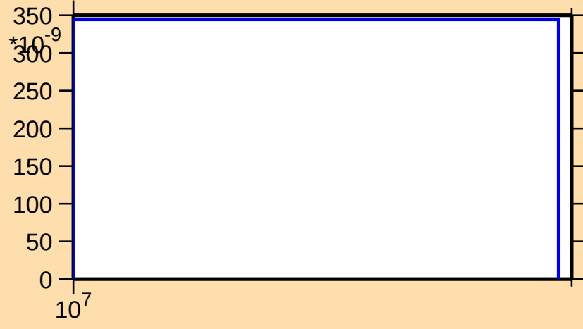
\sigma vs. E for ^{162}\text{W}(n,2np)
