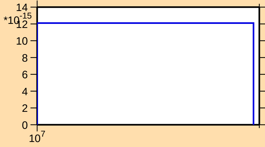
\sigma vs. E for ^{162}\text{W}(n,nt)
