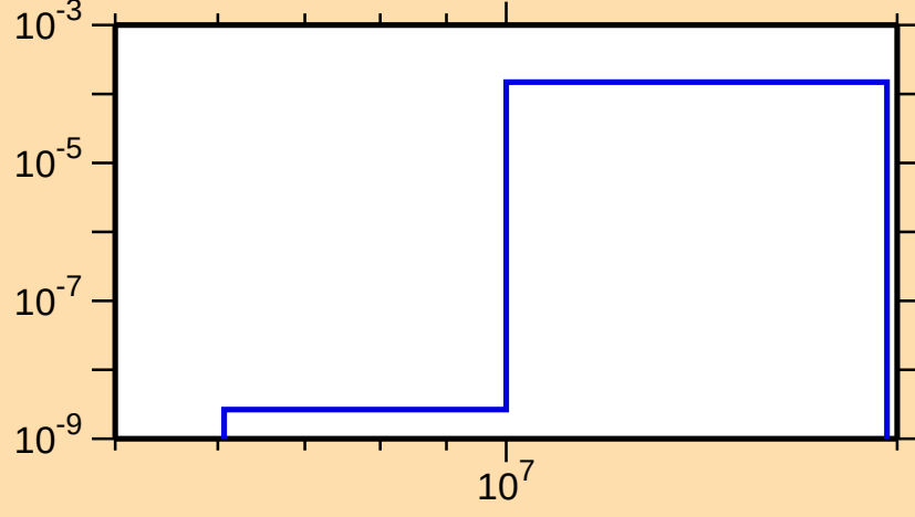
\sigma vs. E for ^{162}\text{W}(n,\text{pd})
