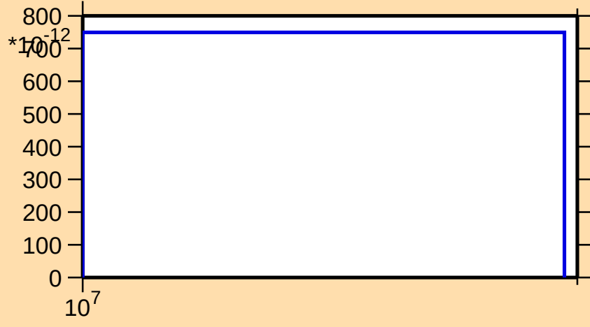
\sigma vs. E for ^{162}\text{W}(\text{n},\text{nd})
