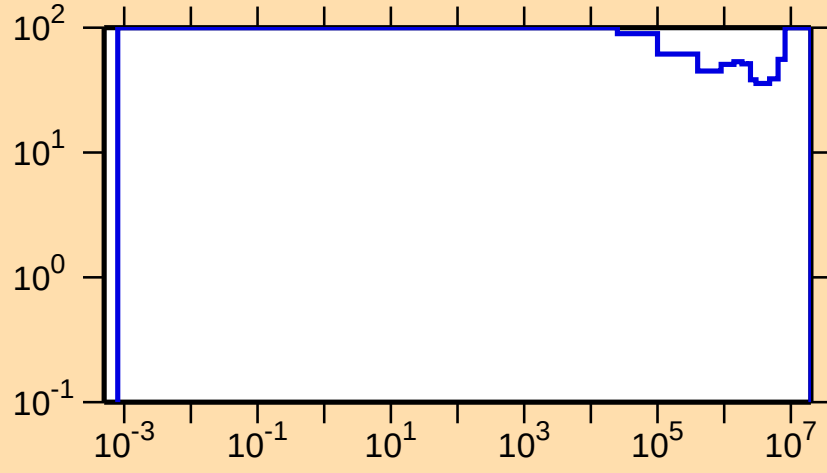
\Delta\sigma/\sigma vs. E for ^{162}\text{W}(n,p)
