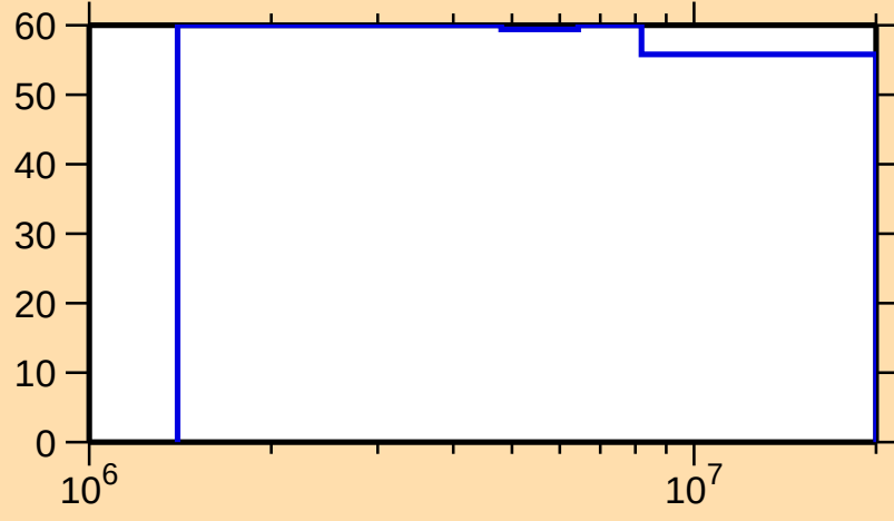
\Delta\sigma/\sigma vs. E for ^{162}\text{W}(n,n_1)
