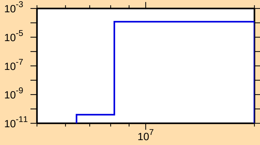
\sigma vs. E for ^{162}\text{W}(n,\text{pd})
