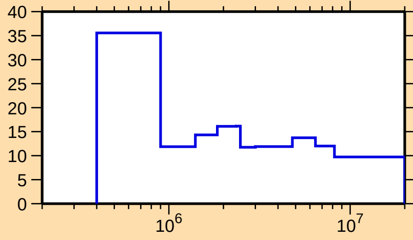
\Delta\sigma/\sigma vs. E for ^{162}\text{W}(n,\text{nonel.})
