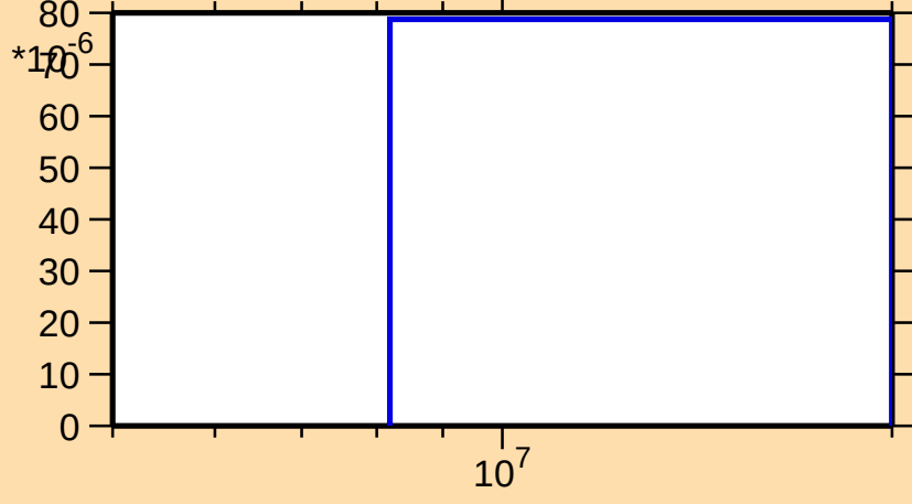
\sigma vs. E for ^{162}\text{W}(n,t)
