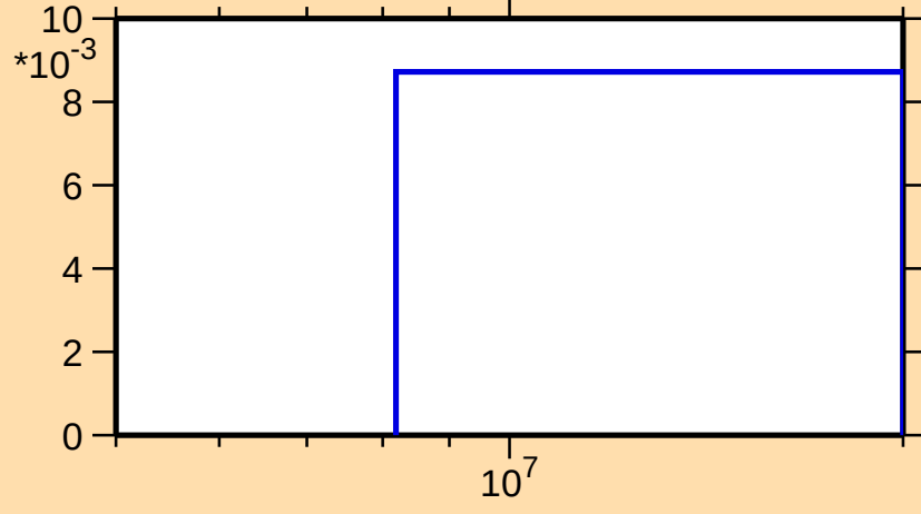
\sigma vs. E for ^{162}\text{W}(n,2n)
