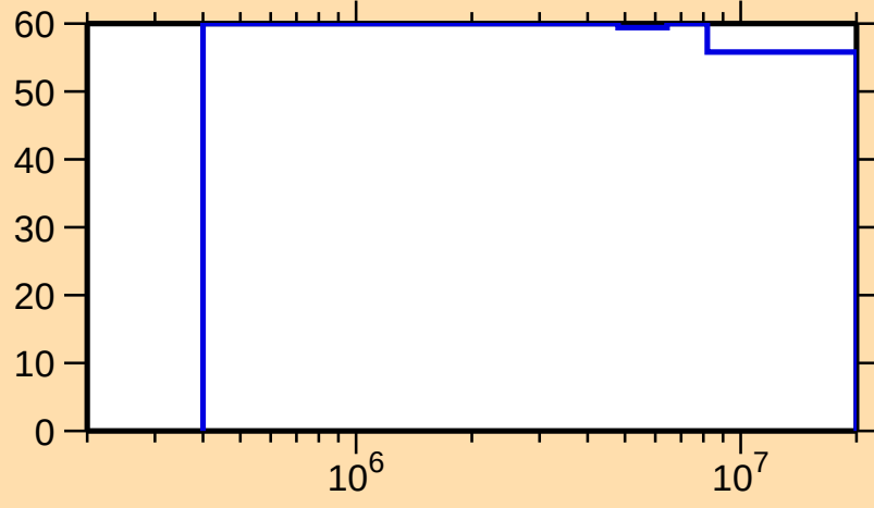
\Delta\sigma/\sigma vs. E for ^{162}\text{W}(n,n_1)
