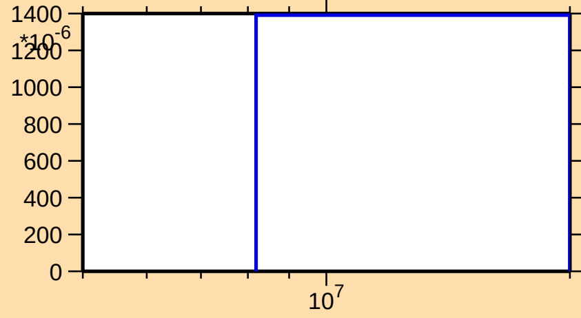
\sigma vs. E for ^{162}\text{W}(n,2n\alpha)
