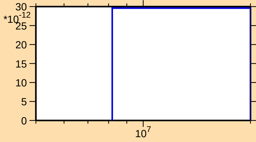
\sigma vs. E for ^{162}\text{W}(\text{mt } 34)
