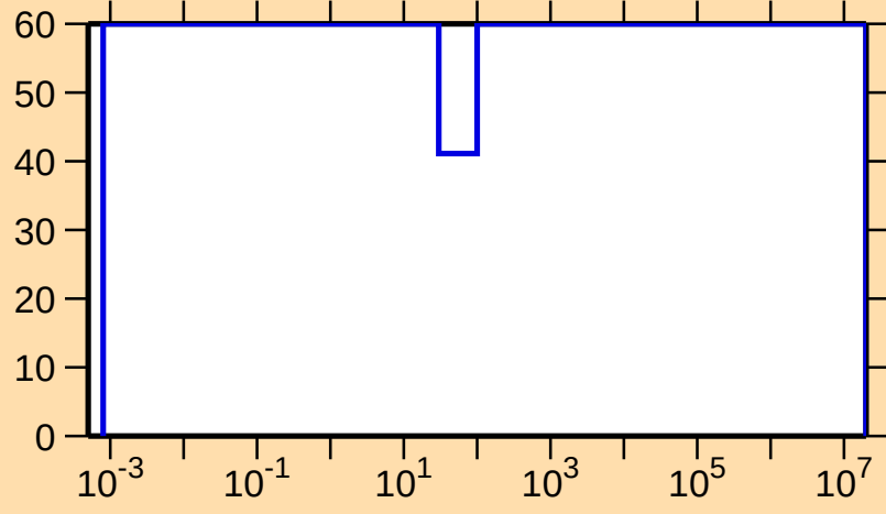
\Delta\sigma/\sigma vs. E for ^{162}\text{W}(n,\gamma)
