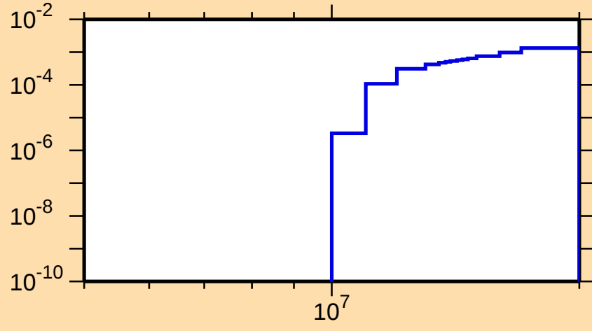
\sigma vs. E for ^{163}\text{W}(n,2n\alpha)
