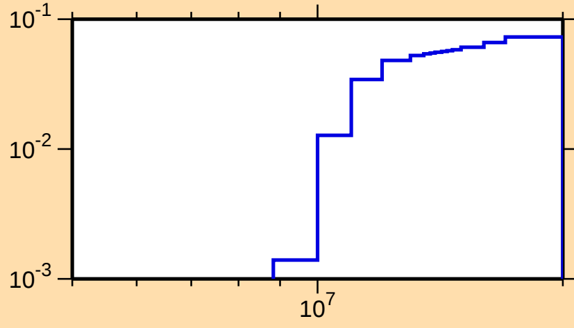
\sigma vs. E for ^{163}\text{W}(n,2n)
