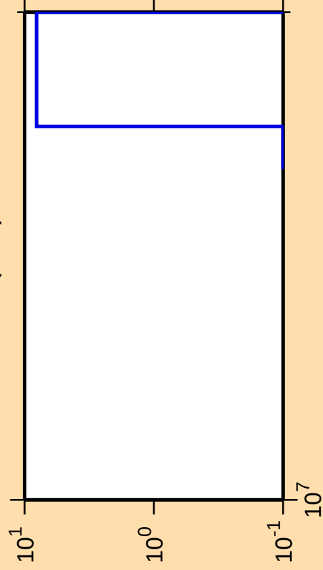
\Delta\sigma/\sigma vs. E for ^{163}\text{W}(n,nt)
