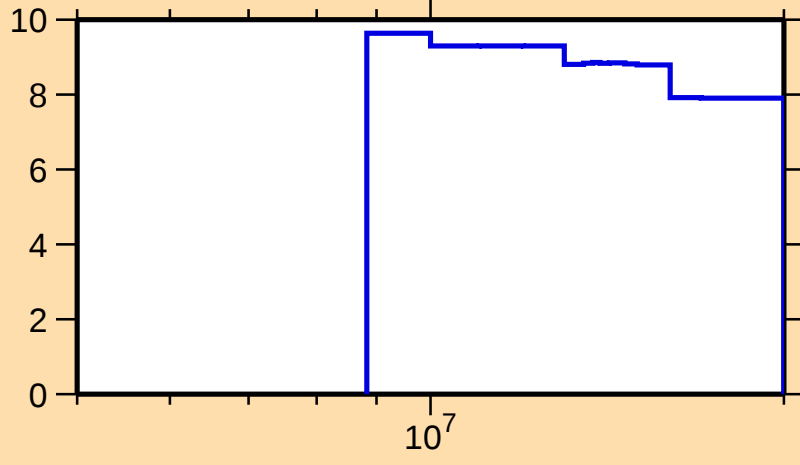
\Delta\sigma/\sigma vs. E for ^{163}\text{W}(n,\text{nonel.})
