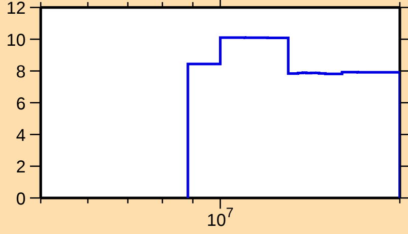
\Delta\sigma/\sigma vs. E for ^{163}\text{W}(n,\text{el.})
