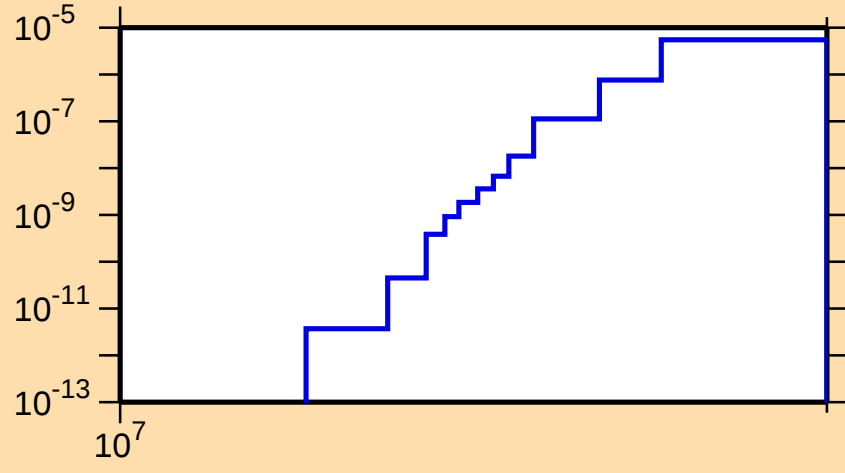
\sigma vs. E for ^{163}\text{W}(n,\text{nd})
