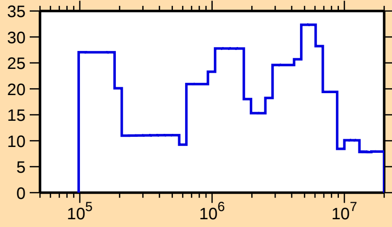
\Delta\sigma/\sigma vs. E for ^{163}\text{W}(\text{n,el.})
