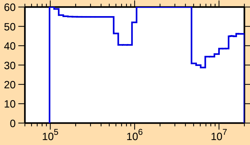
\Delta\sigma/\sigma vs. E for ^{163}\text{W}(n,\text{inel.})
