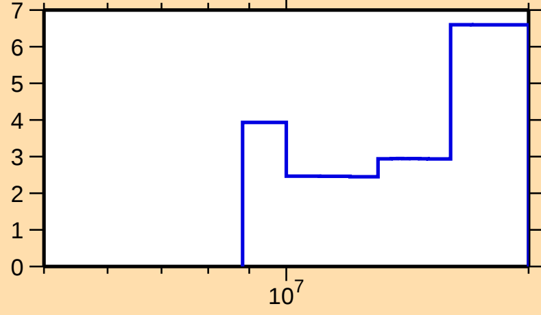
\Delta\sigma/\sigma vs. E for ^{163}\text{W}(n,\text{tot.})
