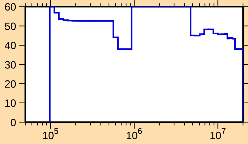
\Delta\sigma/\sigma vs. E for ^{163}\text{W}(n,n_1)
