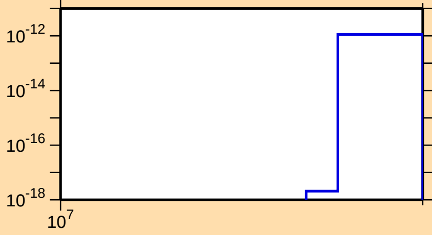
\sigma vs. E for ^{163}\text{W}(n,nt)
