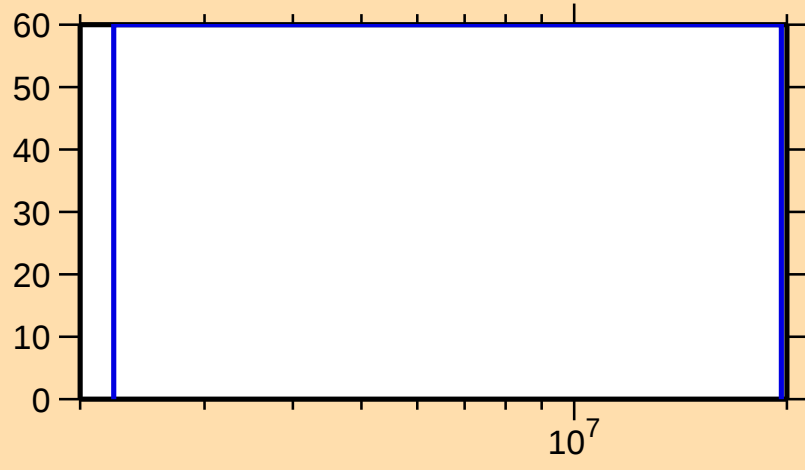
\Delta\sigma/\sigma vs. E for ^{163}\text{W}(n,ncont.)
