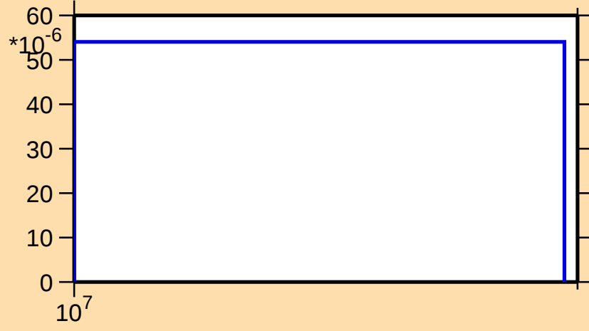
\sigma vs. E for ^{163}\text{W}(n,2np)
