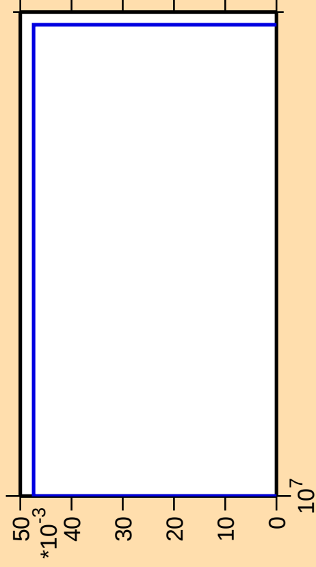
\Delta\sigma/\sigma vs. E for ^{163}\text{W}(n,nt)
