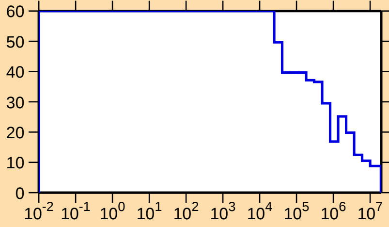
\Delta\sigma/\sigma vs. E for ^{163}\text{W}(n,\text{nonel.})
