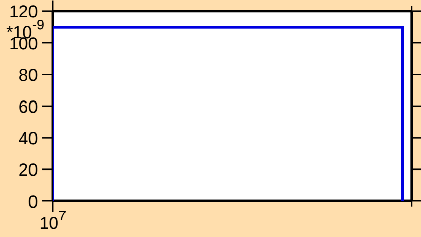
\sigma vs. E for ^{163}\text{W}(\text{n},\text{nd})
