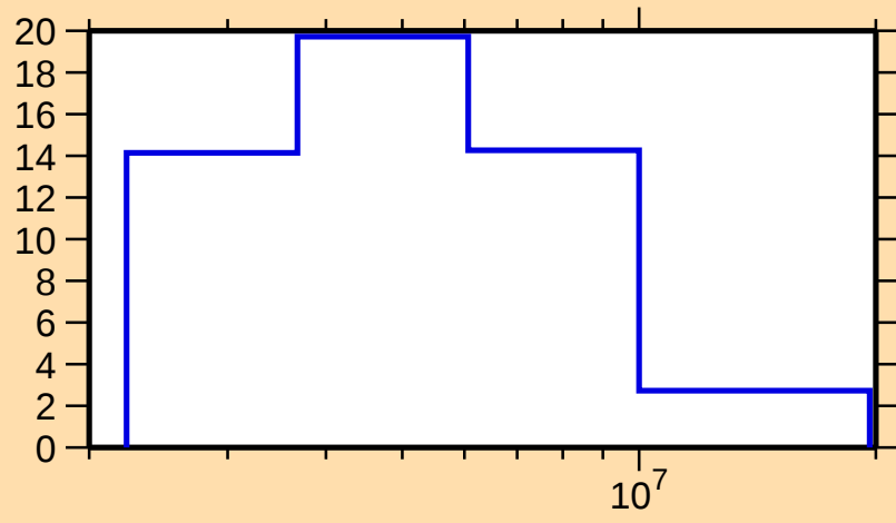
\Delta\sigma/\sigma vs. E for ^{163}\text{W}(\text{n,tot.})
