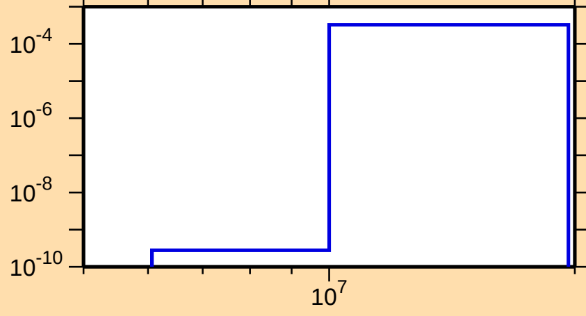
\sigma vs. E for ^{163}\text{W}(n,t)
