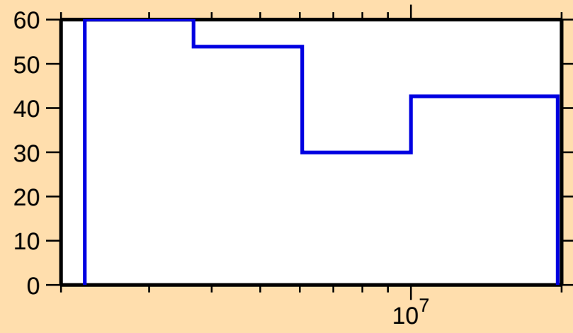
\Delta\sigma/\sigma vs. E for ^{163}\text{W}(\text{n},\text{inel.})
