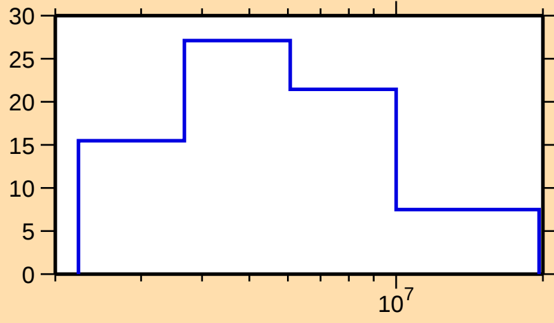
\Delta\sigma/\sigma vs. E for ^{163}\text{W}(\text{n},\text{el.})
