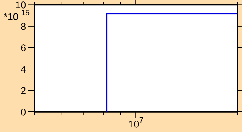
\sigma vs. E for ^{163}\text{W}(\text{n},\text{nt})
