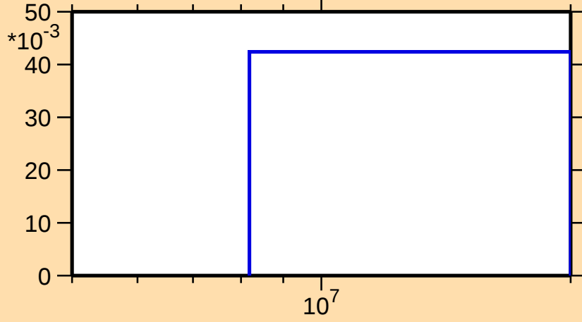
\sigma vs. E for ^{163}\text{W}(n,2n)
