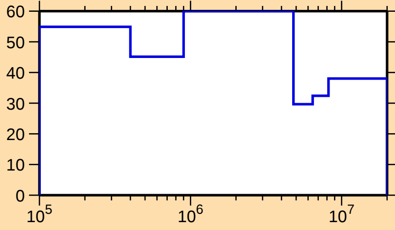
\Delta\sigma/\sigma vs. E for ^{163}\text{W}(n,\text{inel.})
