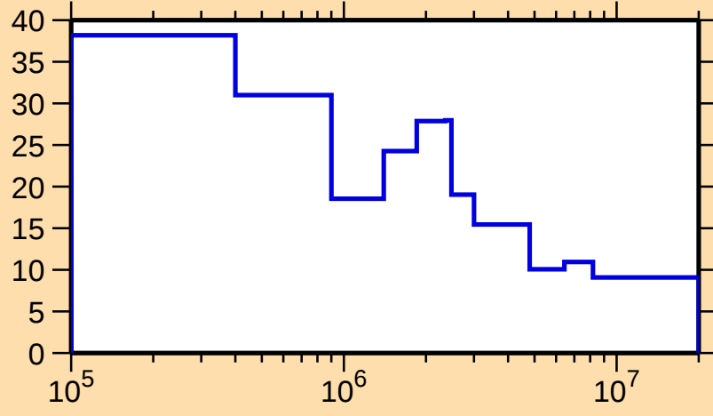
\Delta\sigma/\sigma vs. E for ^{163}\text{W}(\text{n,nonel.})
