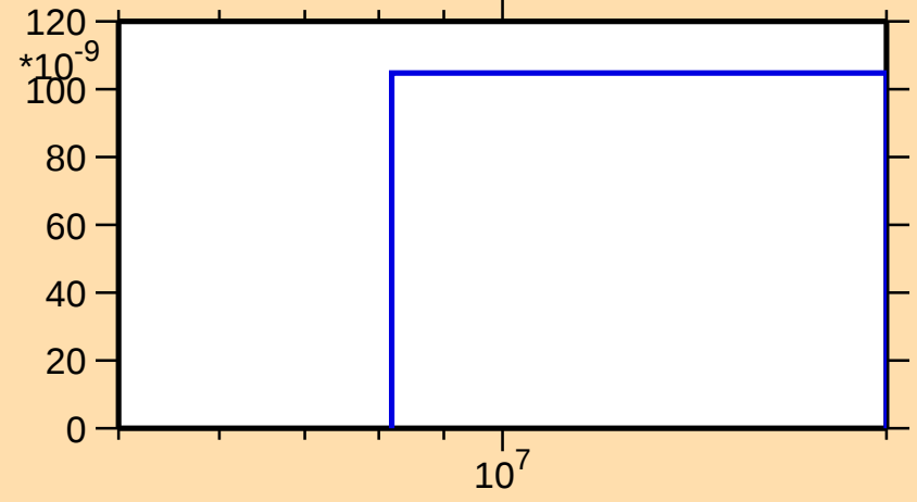
\sigma vs. E for ^{163}\text{W}(\text{mt117})
