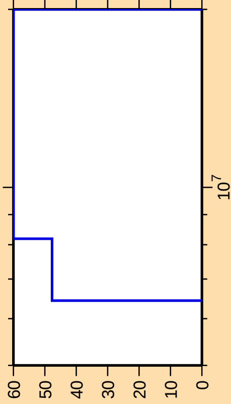
\Delta\sigma/\sigma vs. E for ^{163}\text{W}(\text{mt } 45)
