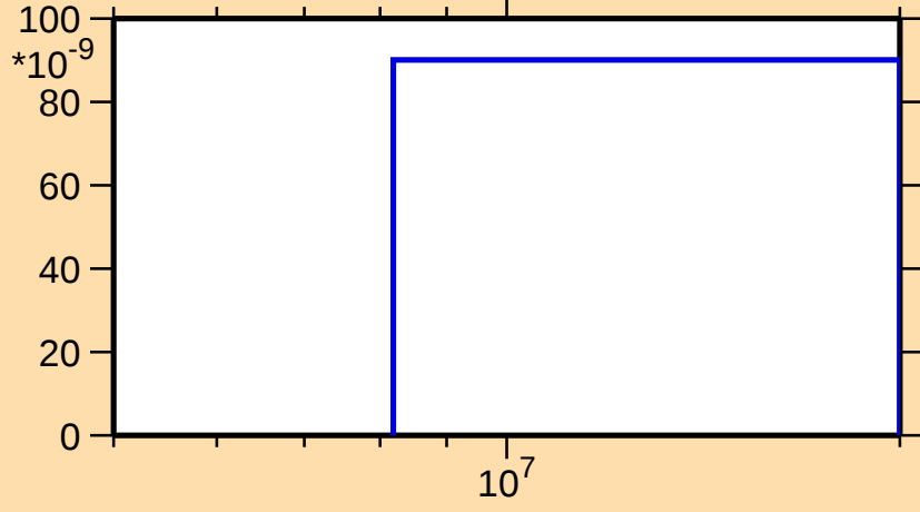
\sigma vs. E for ^{163}\text{W}(\text{n},\text{nd})
