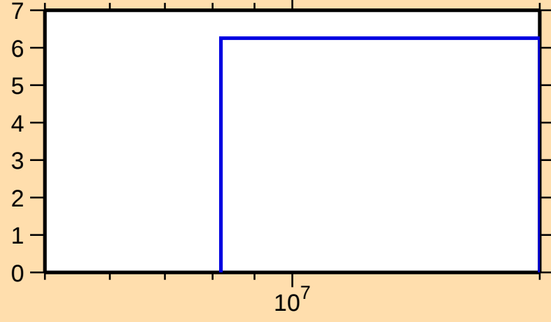
\Delta\sigma/\sigma vs. E for ^{163}\text{W}(n,\text{el.})
