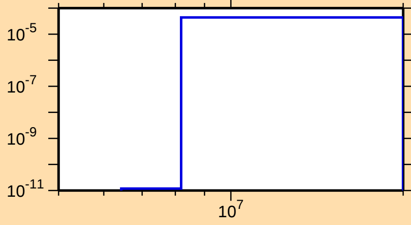
\sigma vs. E for ^{163}\text{W}(\text{mt } 45)
