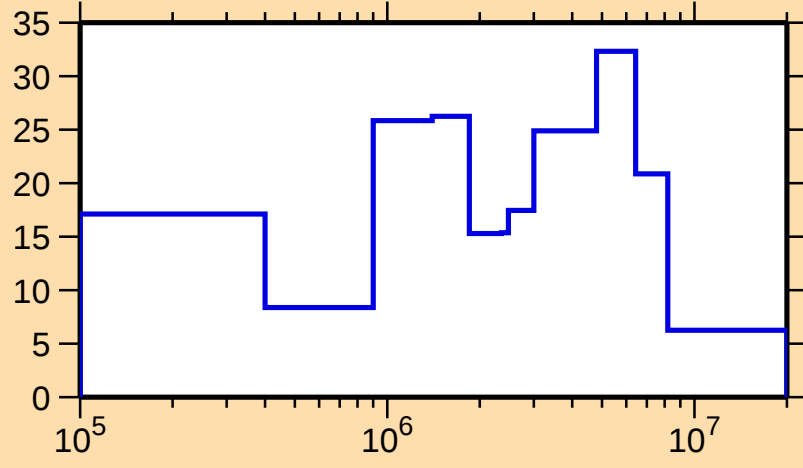
\Delta\sigma/\sigma vs. E for ^{163}\text{W}(n,\text{el.})
