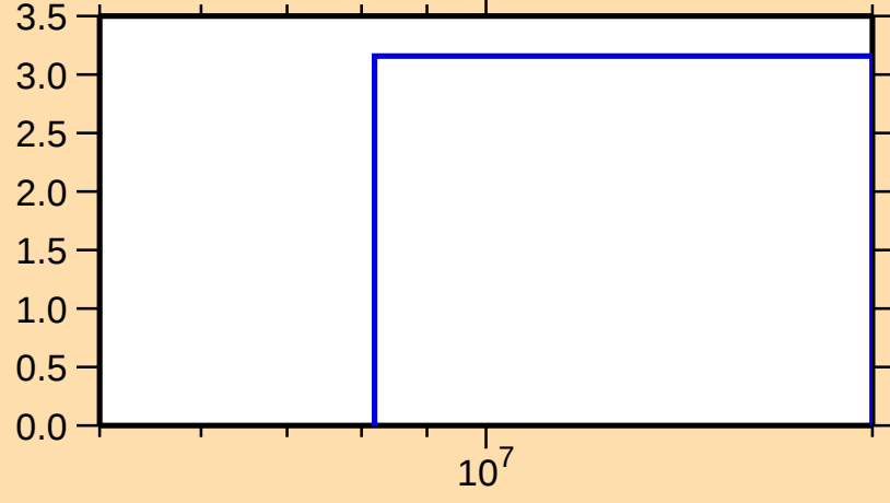
\Delta\sigma/\sigma vs. E for ^{163}\text{W}(n,\text{tot.})
