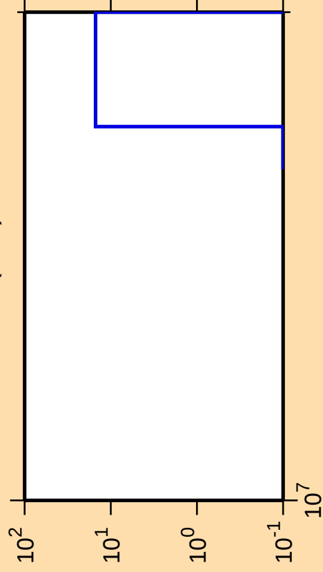
\Delta\sigma/\sigma vs. E for ^{164}\text{W}(n,nt)
