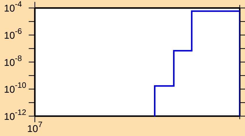
\sigma vs. E for ^{164}\text{W}(n,2np)
