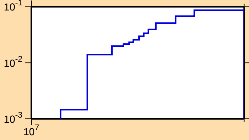
\sigma vs. E for ^{164}\text{W}(n,2n)
