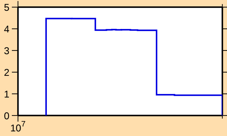
\Delta\sigma/\sigma vs. E for ^{164}\text{W}(n,\text{tot.})
