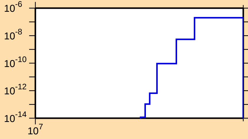
\sigma vs. E for ^{164}\text{W}(n,\text{nd})
