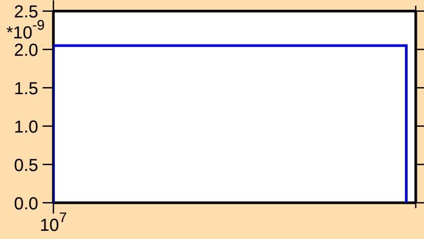
\sigma vs. E for ^{164}\text{W}(\text{n},\text{nd})
