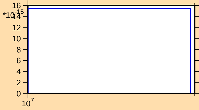
\sigma vs. E for ^{164}\text{W}(n,nt)
