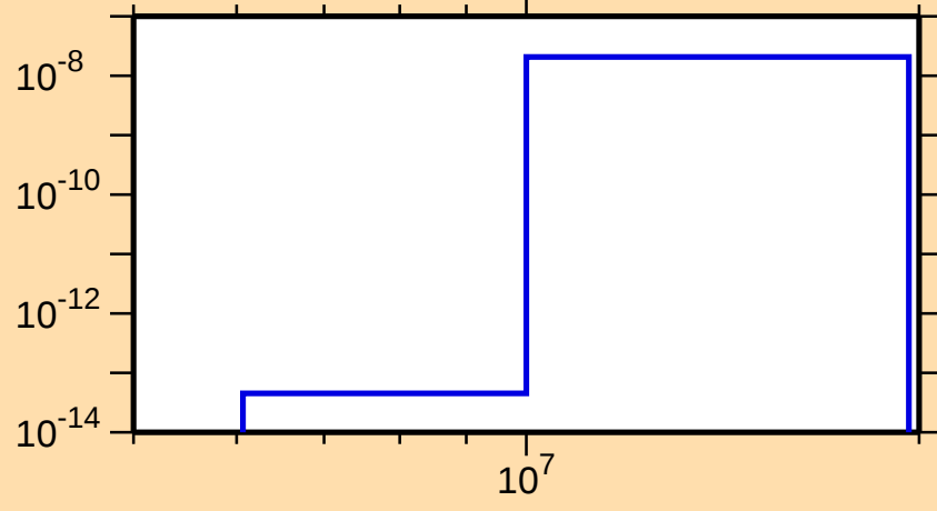
\sigma vs. E for ^{164}\text{W}(\text{mt117})
