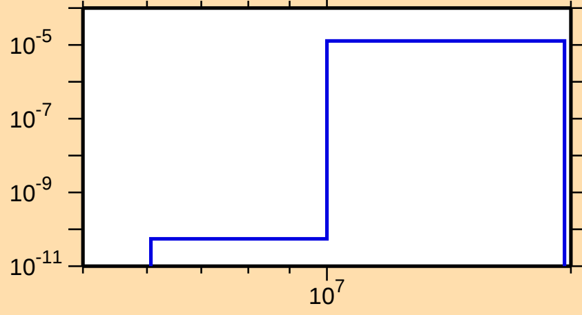
\sigma vs. E for ^{164}\text{W}(\text{mt } 45)
