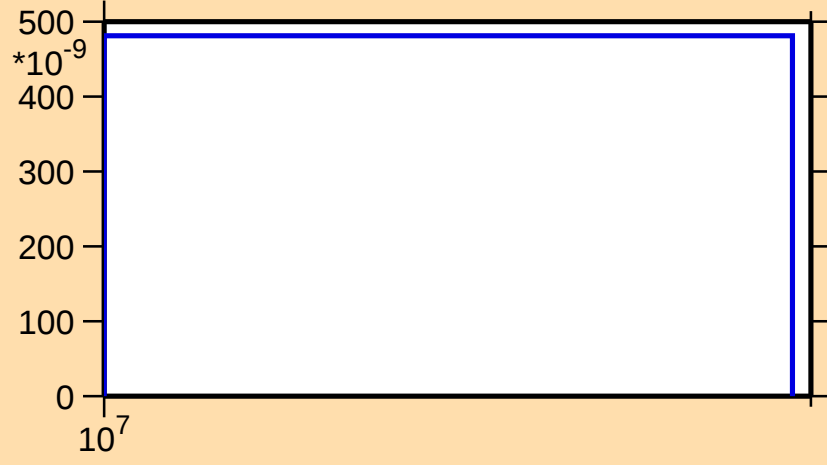
\sigma vs. E for ^{164}\text{W}(n,2np)
