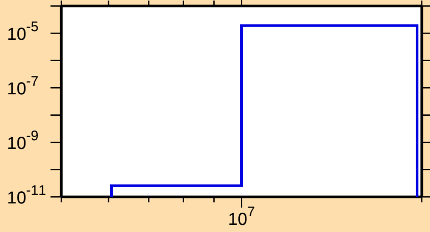
\sigma vs. E for ^{164}\text{W}(n,\text{pd})
