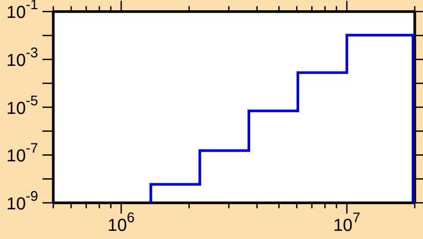
\sigma vs. E for ^{164}\text{W}(n,p\alpha)
