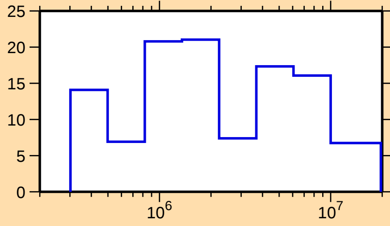
\Delta\sigma/\sigma vs. E for ^{164}\text{W}(n,\text{el.})
