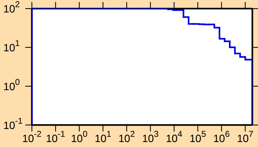
\Delta\sigma/\sigma vs. E for ^{164}\text{W}(n,\text{nonel.})
