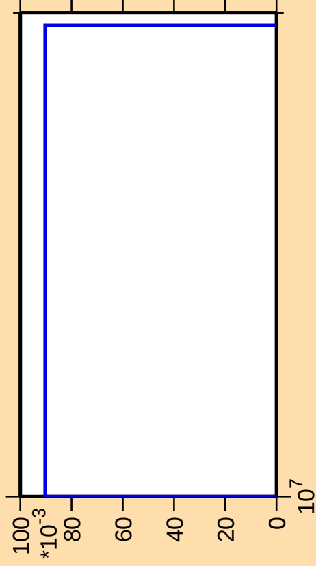
\Delta\sigma/\sigma vs. E for ^{164}\text{W}(n,nt)
