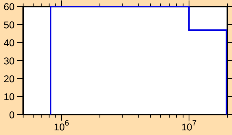
\Delta\sigma/\sigma vs. E for ^{164}\text{W}(n,n\text{cont.})
