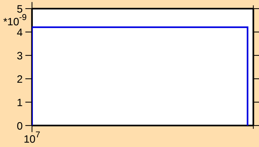
\sigma vs. E for ^{164}\text{W}(\text{n},\text{pt})
