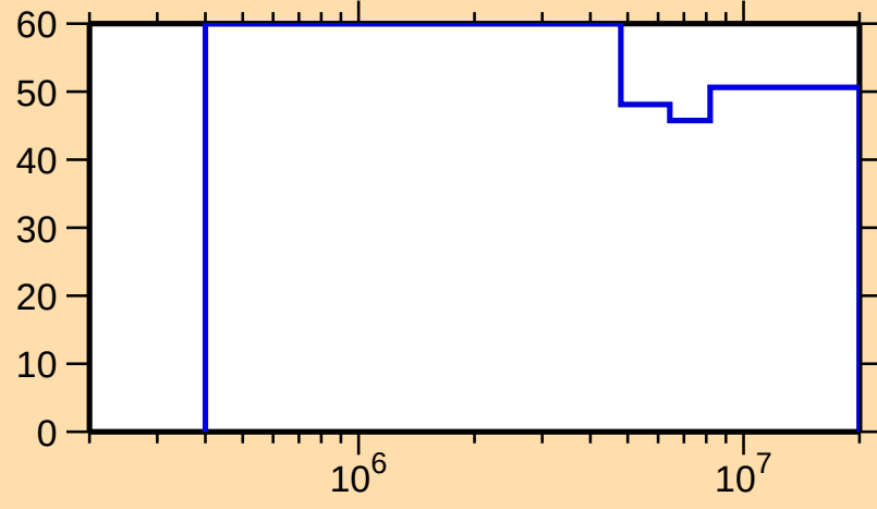
\Delta\sigma/\sigma vs. E for ^{164}\text{W}(\text{n},\text{inel.})
