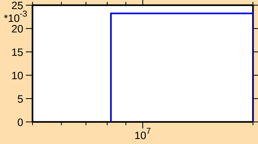
\sigma vs. E for ^{164}\text{W}(n,2n)
