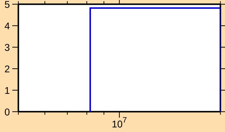
\Delta\sigma/\sigma vs. E for ^{164}\text{W}(n,\text{nonel.})
