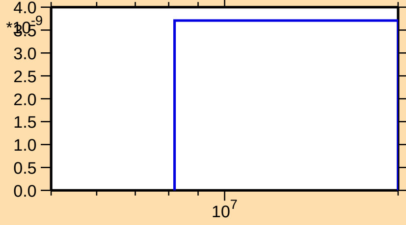
\sigma vs. E for ^{164}\text{W}(n,\text{pt})
