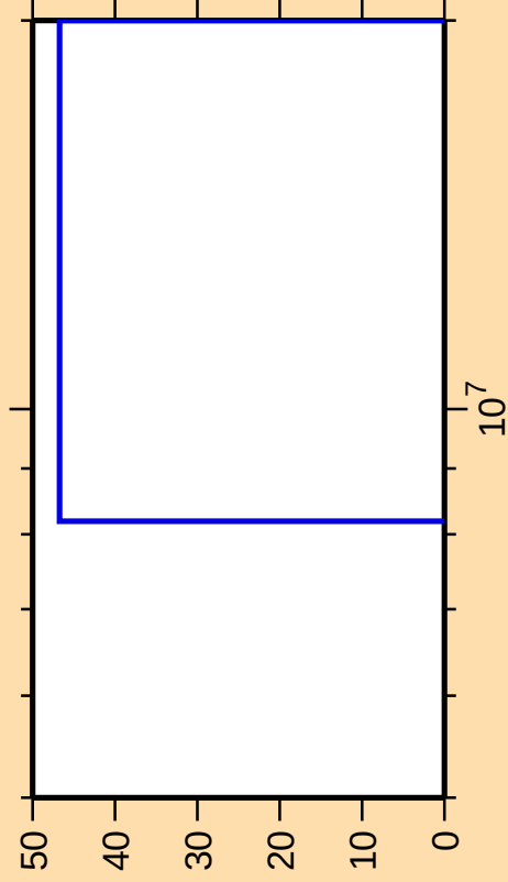
\Delta\sigma/\sigma vs. E for ^{164}\text{W}(\text{n},\text{ncont.})
