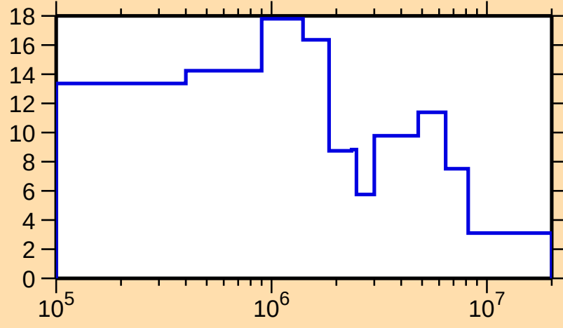
\Delta\sigma/\sigma vs. E for ^{164}\text{W}(n,\text{tot.})
