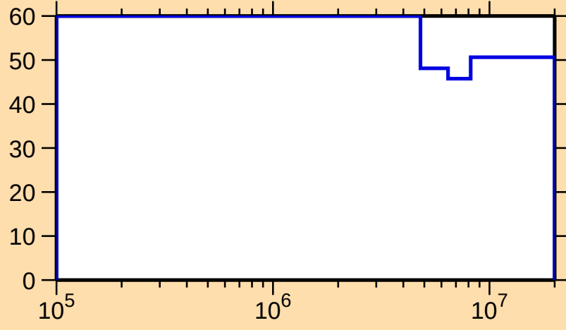
\Delta\sigma/\sigma vs. E for ^{164}\text{W}(n,\text{inel.})
