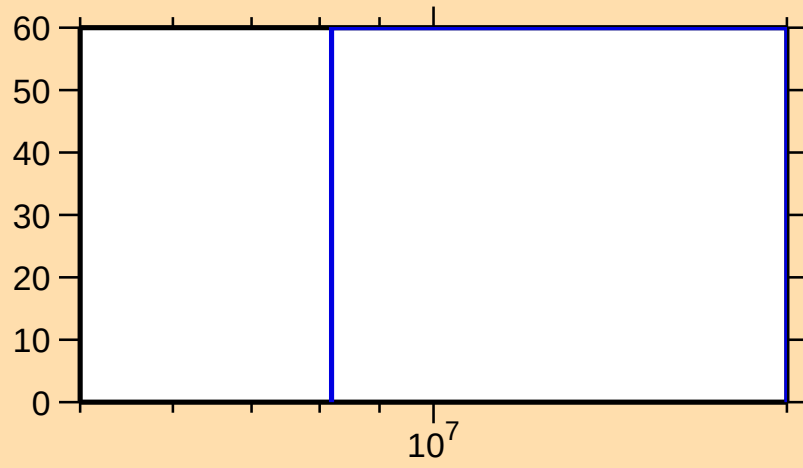
\Delta\sigma/\sigma vs. E for ^{164}\text{W}(n,2n)
