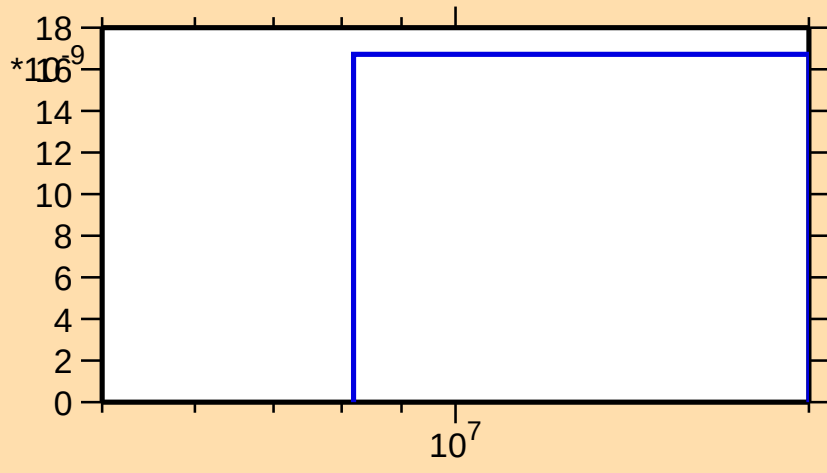
\sigma vs. E for ^{164}\text{W}(\text{mt117})
