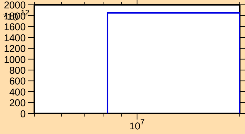
\sigma vs. E for ^{164}\text{W}(n,\text{nd})
