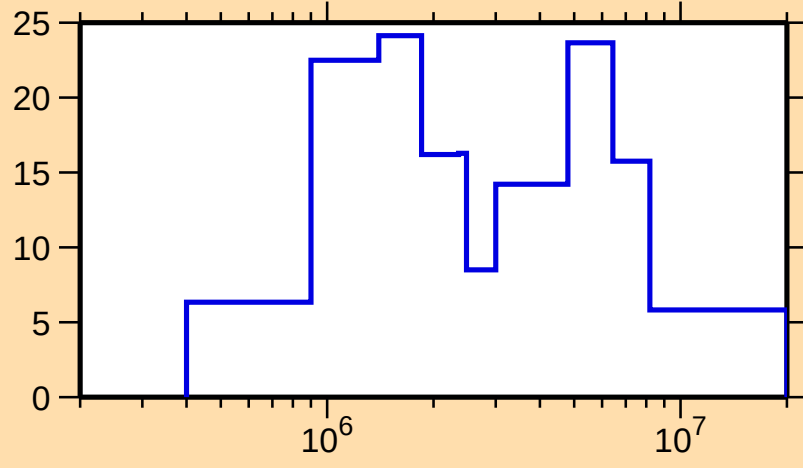
\Delta\sigma/\sigma vs. E for ^{164}\text{W}(\text{n},\text{el.})
