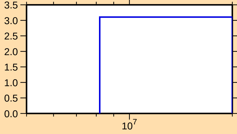
\Delta\sigma/\sigma vs. E for ^{164}\text{W}(n,\text{tot.})
