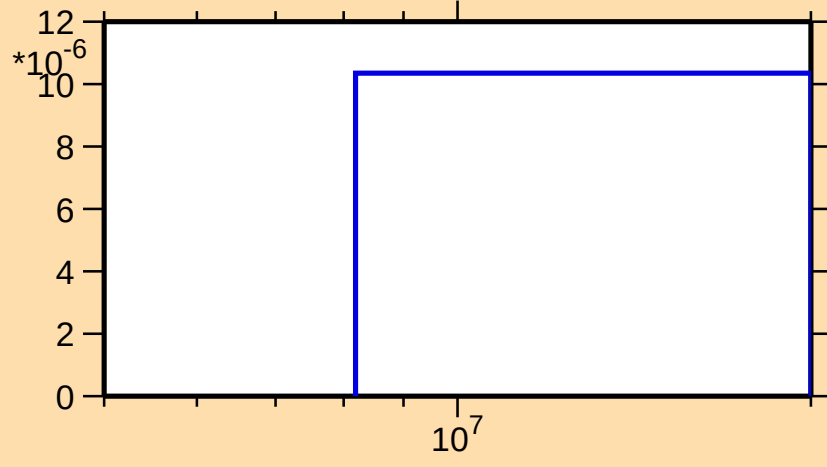
\sigma vs. E for ^{164}\text{W}(\text{mt 45})
