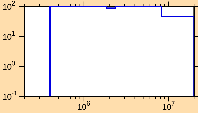
\Delta\sigma/\sigma vs. E for ^{164}\text{W}(n,n\text{cont.})
