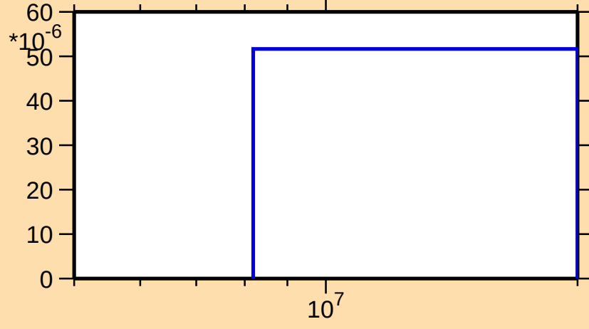
\sigma vs. E for ^{164}\text{W}(n,t)
