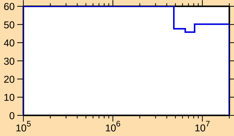
\Delta\sigma/\sigma vs. E for ^{164}\text{W}(n,n_1)
