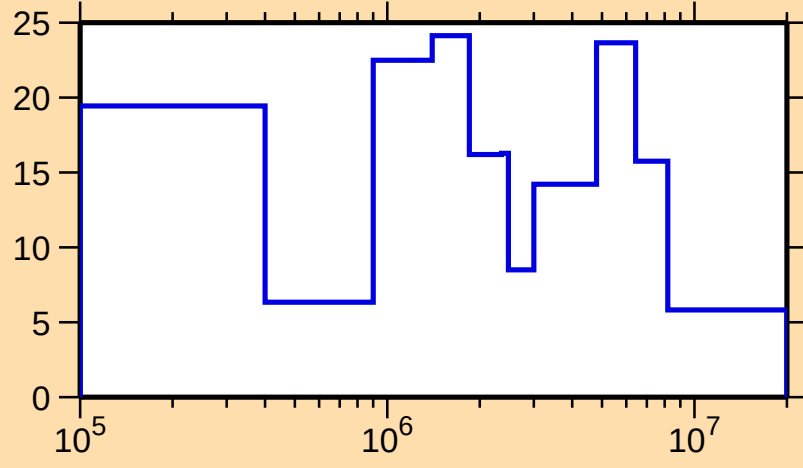
\Delta\sigma/\sigma vs. E for ^{164}\text{W}(n,\text{el.})
