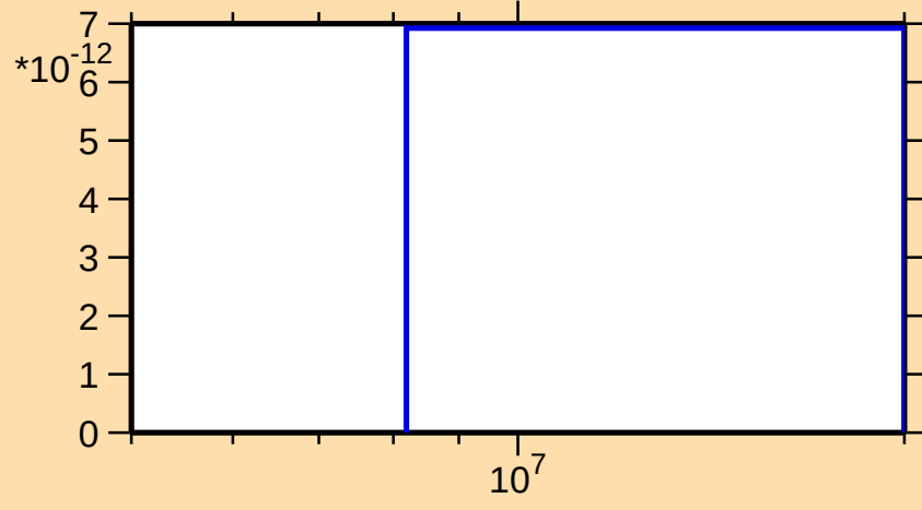
\sigma vs. E for ^{164}\text{W}(\text{mt } 34)
