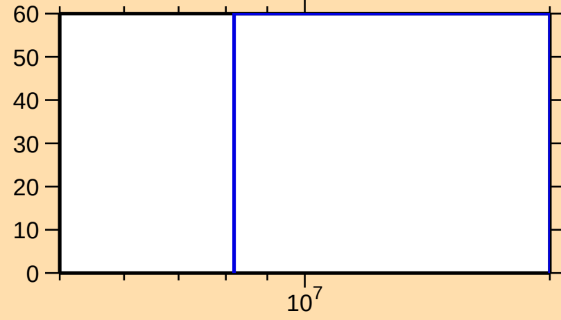
\Delta\sigma/\sigma vs. E for ^{164}\text{W}(\text{n},2\text{n})
