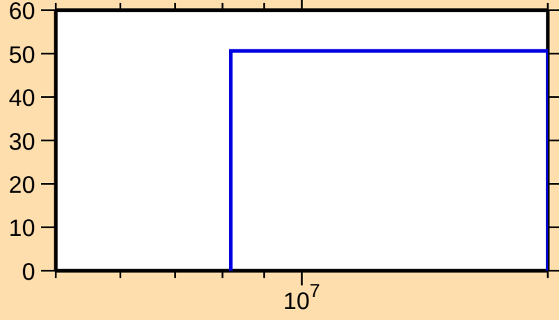
\Delta\sigma/\sigma vs. E for ^{164}\text{W}(n,\text{inel.})
