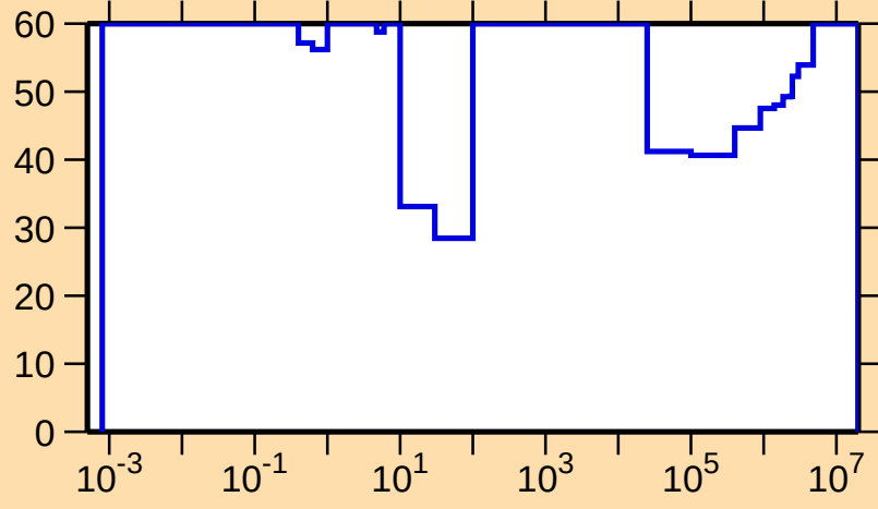
\Delta\sigma/\sigma vs. E for ^{164}\text{W}(n,\gamma)
