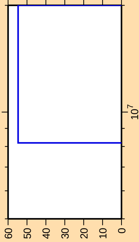
\Delta\sigma/\sigma vs. E for ^{164}\text{W}(\text{mt } 34)
