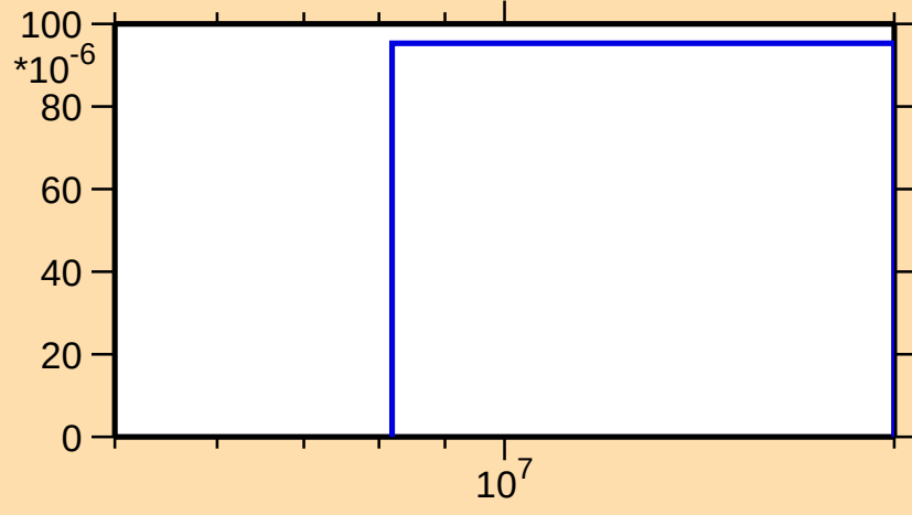
\sigma vs. E for ^{164}\text{W}(n,2n\alpha)
