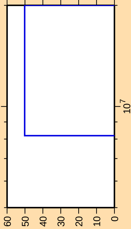
\Delta\sigma/\sigma vs. E for ^{164}\text{W}(n,n_1)
